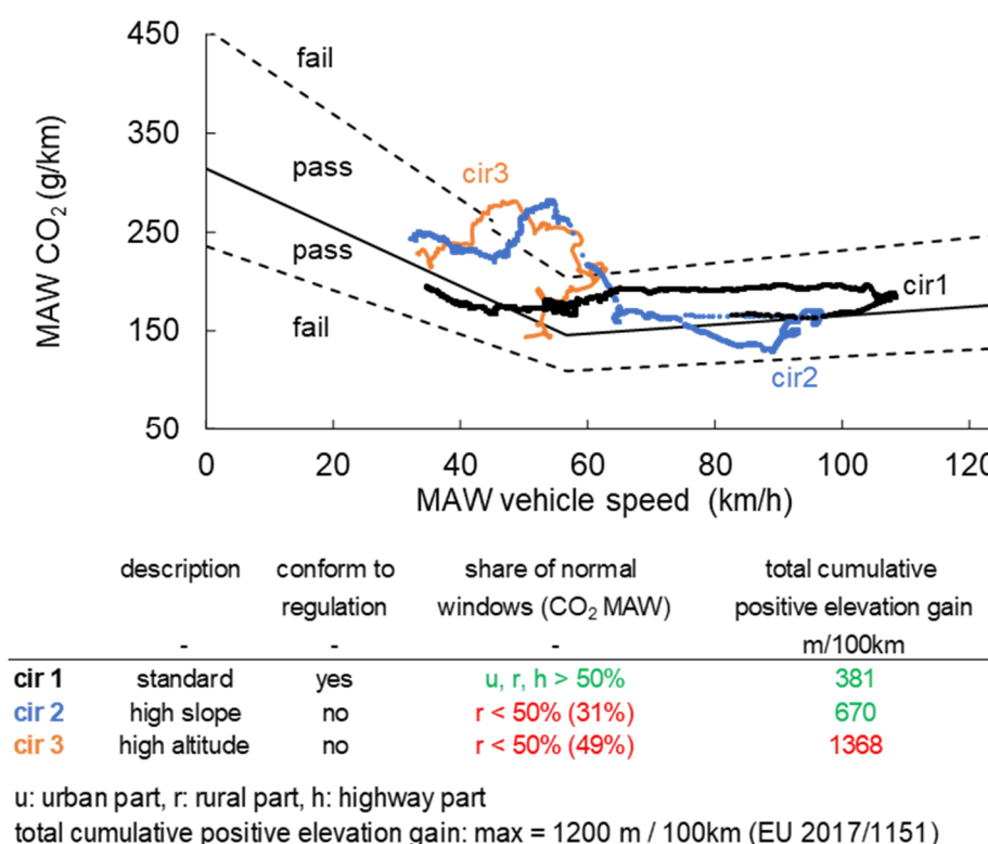
Figure 11. Influence of the varying altitude and slope on the trip validity, gasoline (V1).
