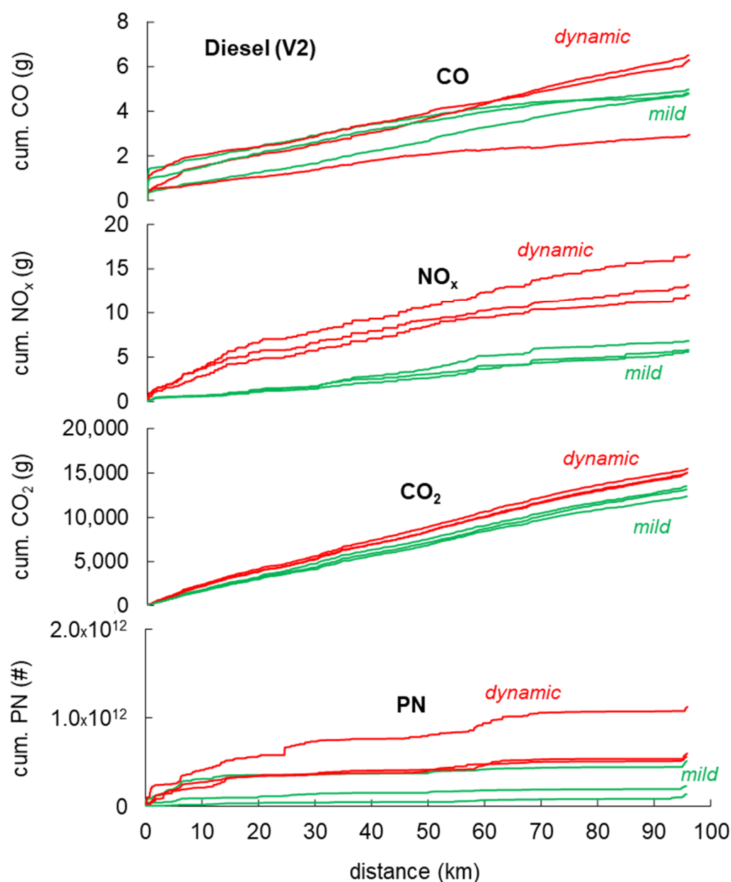
Figure 8. Influences of the driving style on the cumulated emissions of the diesel vehicle (V2).
