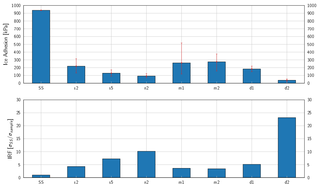
Figure 4.7: Ice adhesion strength using a share stress test and Ice Reduction Factor (IRF) using SS as reference.
