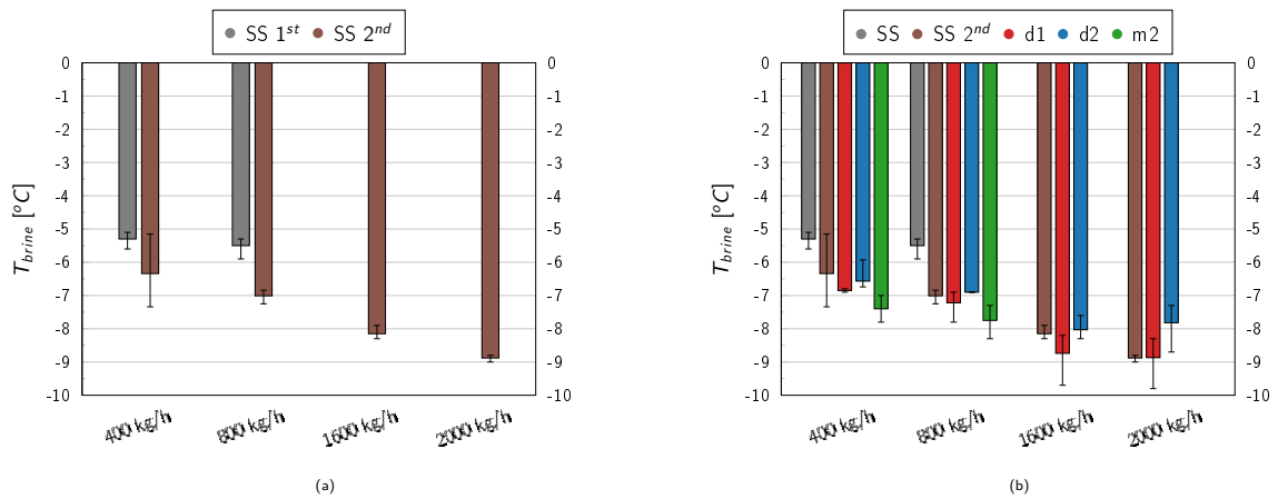
Figure 5.7: (a) First and second round of experiments for the reference stainless steel tubes; (b) All experimental results including those from the first and second campaign for the stainless steel tubes
