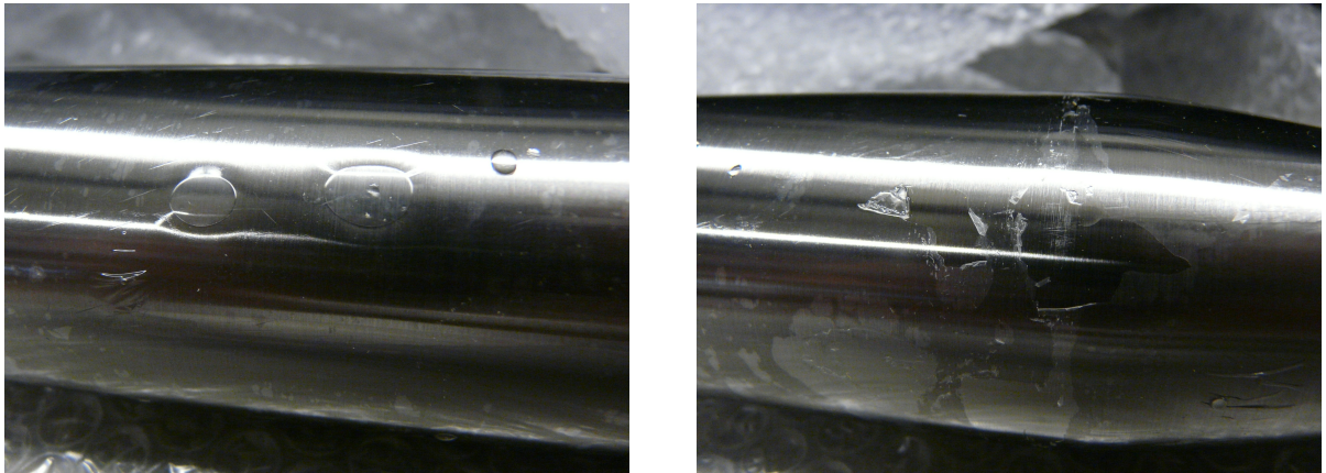
Figure 5.4: Left: Detached coating m2 after running the experiment with a mass flow of 1600 kg/h. Water filled bubbles on the tube surface and right: pilled off coating at the tip of the tube within the region where the coldest temperatures are reached in the system.
