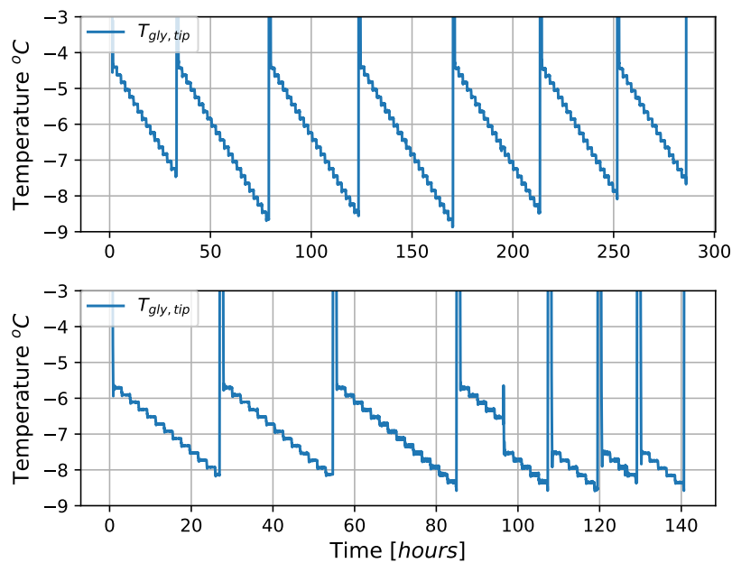
Figure 5.6: Top: Brine temperature at the tip of the tube. Comparison of cycles with fixed starting temperature. Bottom: and with freezing-point dependent starting temperature for the cooling procedure. Experiments with stainless steel tube at a mass flow rate of 1600 kg/h.
