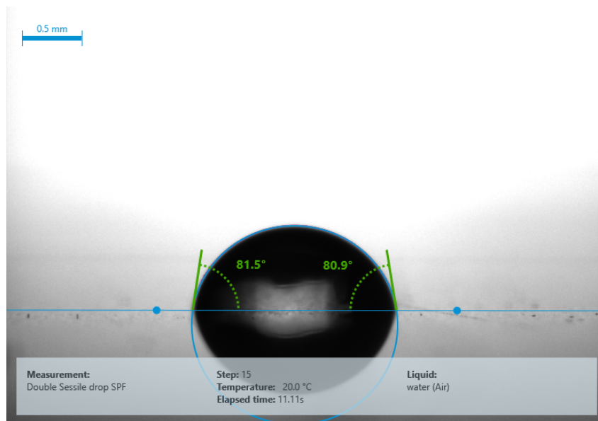
Figure 3.3: Example of the static contact angle determined using the KRÜSS Mobile Surface Analyzer from HSR-IWK and the sessile drop method.
