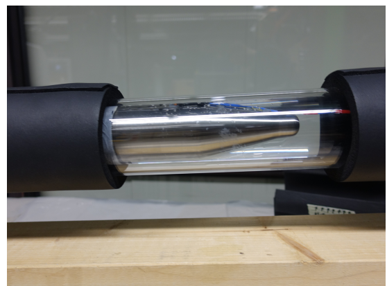
Figure 3.13: Left: Laboratory setup to test the coated tubes under flow conditions; right: tip of sample tube
