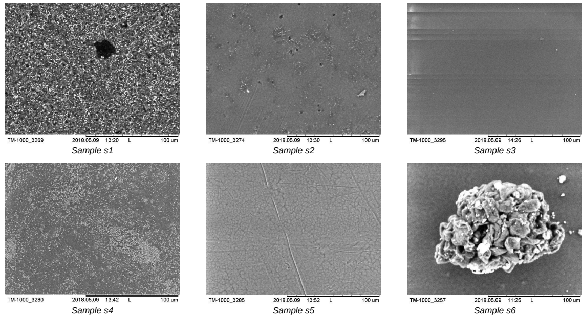
Figure 4.2: Microscope pictures of sample s1, s2, s3, s4, s5 and s6 showing coatings defects like holes and cracks.
