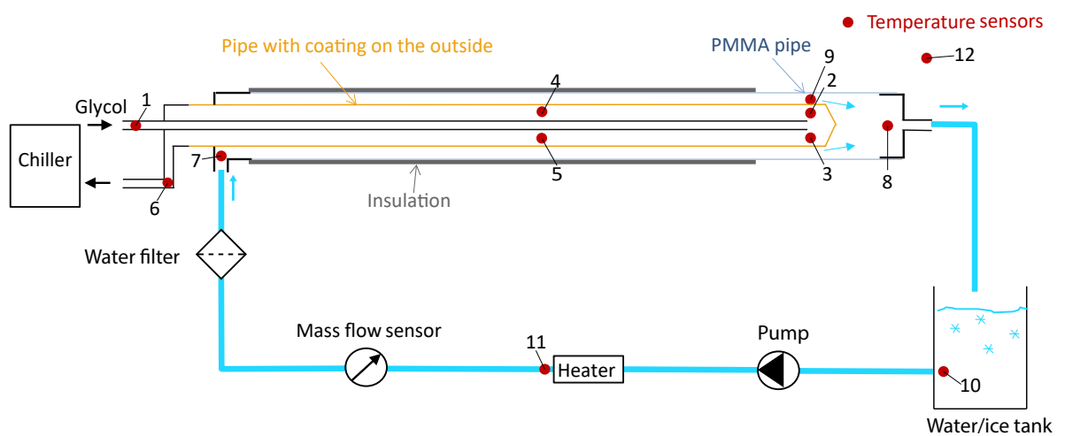
Figure 3.12: Schematic of the experimental setup used to test coated tubes under flow conditions.
