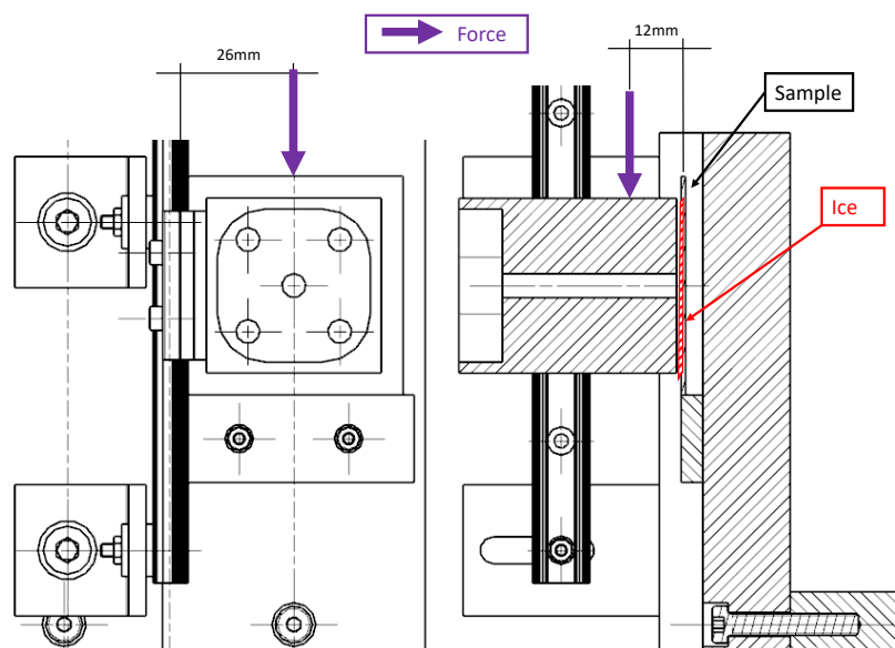
Figure 3.9: Left: experimental set-up used for measuring the shear stress. Right: enclosure with controlled temperature used for ice adhesion test.
