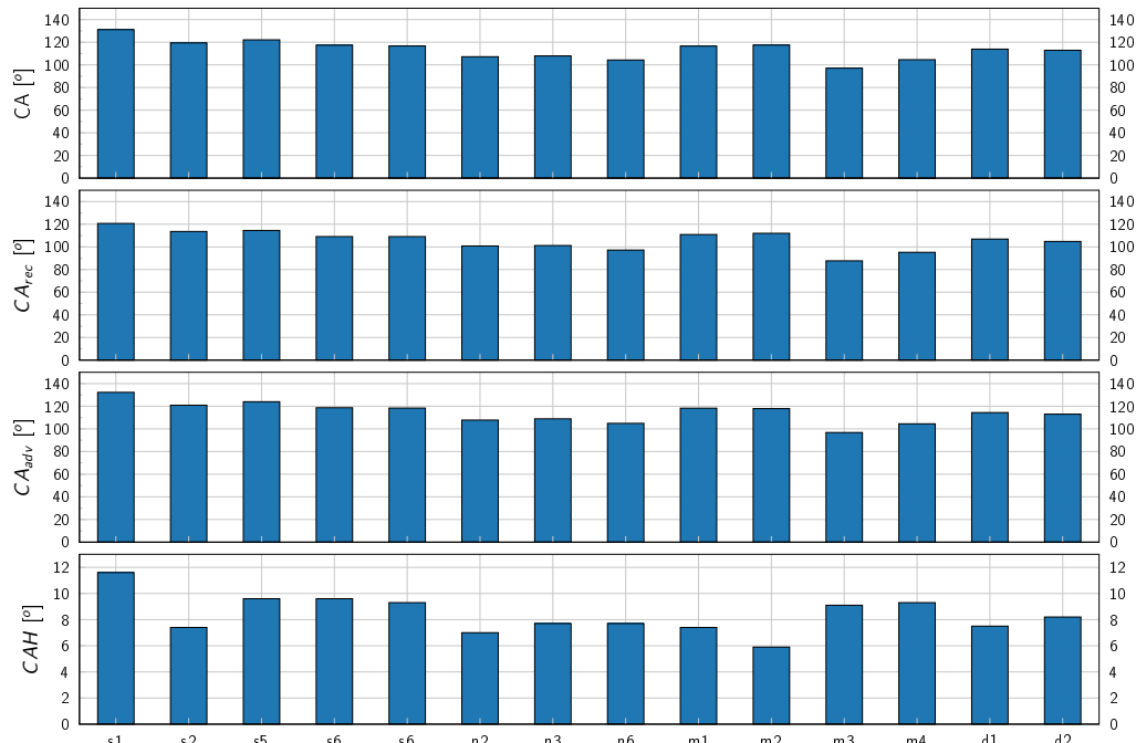
Figure 4.4: Contact angle (CA), receding CA, advancing CA and CA hysteresis (CAH).
