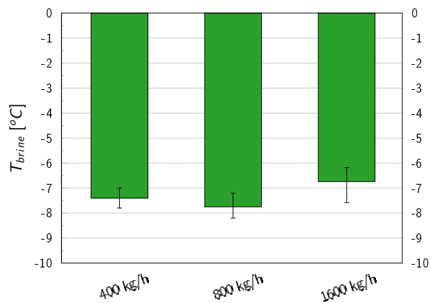
Figure 5.5: Results of the tube experiments with m2 coating including the experiment with a mass flow of 1600 kg/h, where the coating failed during an early stage of the experiment.
