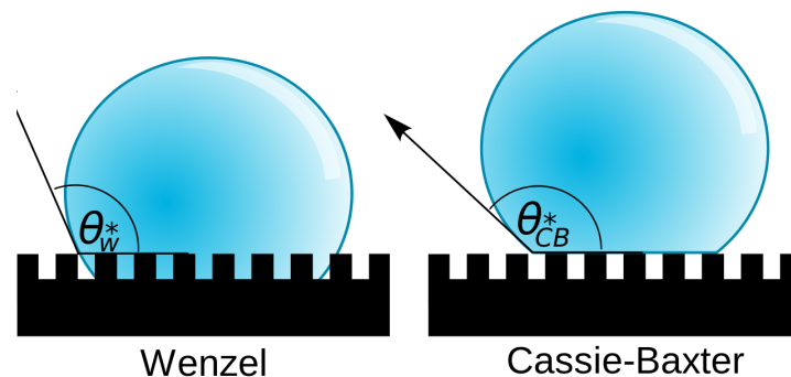
Figure 2.2: Wetting models for superhydrophobic surfaces: (left) homogenous wetting (Wenzel), the liquid follows the solid surface and penetrates into the roughness grooves, (right) heterogeneous wetting (Cassie) where air or another fluid is trapped underneath the liquid, inside the roughness grooves and the liquid is in contact only with top asperities. Picture from https://de.wikipedia.org/wiki/Datei:Contact_angle_microstates.svg
