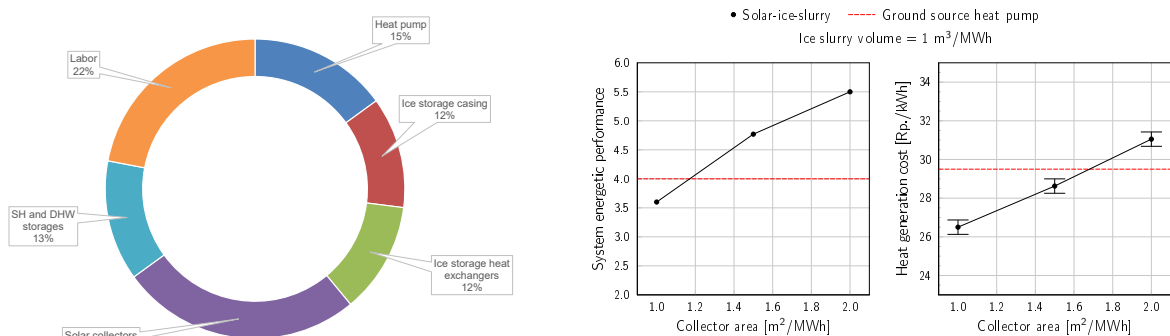
Figure 1.2: Left: installation cost shares for a state-of-the-art ice storage used in solar-ice systems (Carbonell et al., 2017a). Right: System seasonal (yearly) performance factor and heat generation cost for the potential ice-slurry system in comparison to state-of-the-art ground source heat pump system. Results obtained from Carbonell et al. (2017b).
