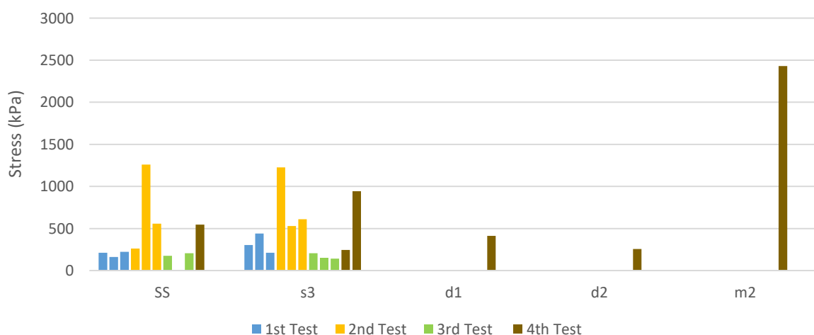
Figure 4.5: Results of the first ice adhesion test with predominantly cohesive ruptures of the ice instead of adhesive detachment. Here only test results with cohesive ruptures are shown.
