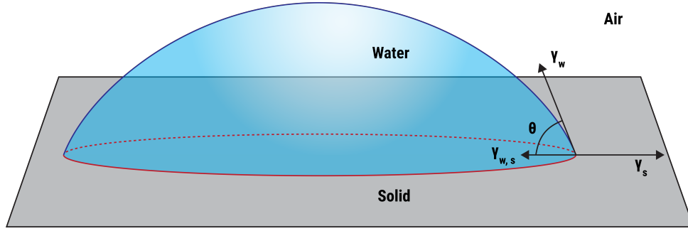
Figure 3.1: Contact angle formed by sessile liquid drop on a smooth homogeneous solid surface
