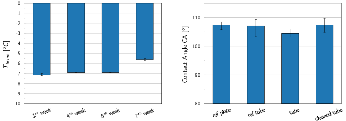
Figure 5.3: Possible effects of degradation or fouling visible in tube measurements with coating d2. Left: Brine temperature for the d2 coating observed in 4 experiments at same mass flow (800 kg/h) over 7 weeks. Right: Contact angle measurements on the tube surface (ref tube: part of the tube without contact to water, tube: tube surface with contact to the water, cleaned tube: tube surface which was in contact to water, but was cleaned afterwards) and on a reference piece - a coated plate (ref plate). The error bars indicate the range of values measured in the different cycles or experiments.
