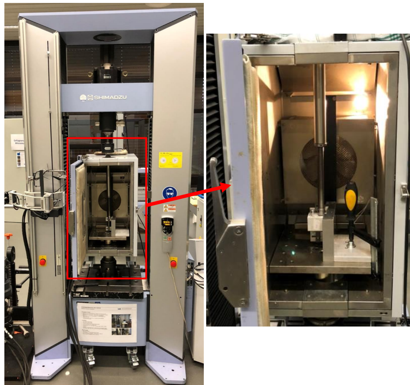
Figure 3.9: Left: experimental set-up used for measuring the shear stress. Right: enclosure with controlled temperature used for ice adhesion test.
