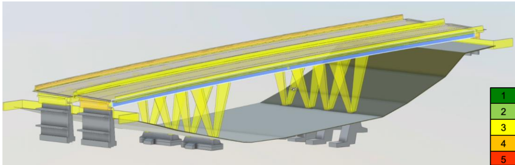
Figure 12: BIM model with the ability to display condition forecasts for various structural components (blue = selected structural element; green through red represent the colors of the ASTRA condition state definition for engineering structures).
