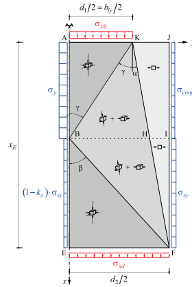
Fig. 4.2 - Dual-Wedge stress field (only one symmetrical half is shown). Transverse stresses are exaggerated compared to vertical stresses.
