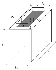
Fig. 4.1 - Definition of strip loading parameters.
