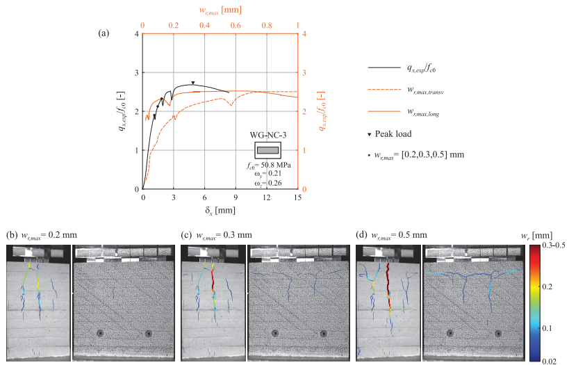
Fig. 4.11 - Crack development in Specimen WG-NC-3: (a) normalised applied average stresses q_{x,exp}/f_{c0} versus penetration \delta_x and maximum crack width w_{r,max} , (b)-(d) crack patterns of two neighbouring lateral sides for load stages with (b) w_{r,max} = 0.2 mm, (c) w_{r,max} = 0.3 mm and (d) w_{r,max} = 0.5 mm.
