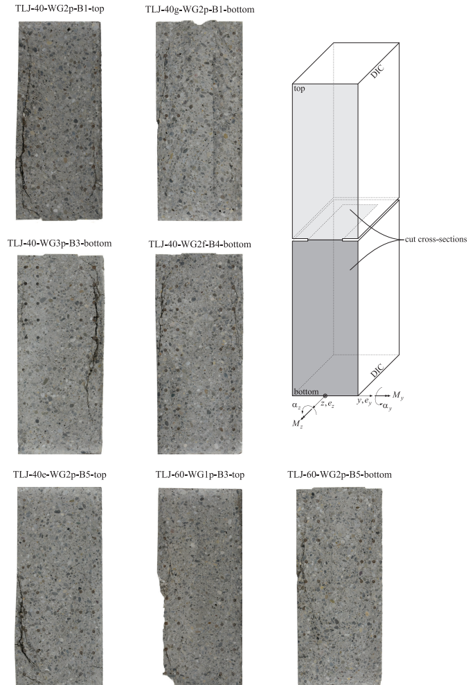
Fig. 5.7 - Vertical transverse cuts through half specimens (top or bottom) after testing. Orientation of half specimens as in the experiments. Longitudinal DIC surface to the positive y side.
