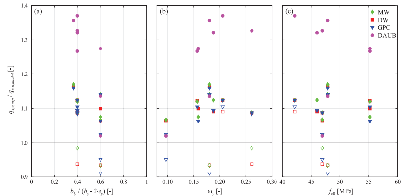
Fig. 5.11 - Comparison of experimental data with model predictions plotted against (a) load concentration ratio b_{ly}/(b_y - 2 \cdot e_y) , (b) transverse mechanical reinforcement ratio \omega_y , and (c) uniaxial concrete compressive strength f_{c0} . Markers without filling indicate the comparison if only the confined zone is considered for specimens with a governing unconfined zone.
