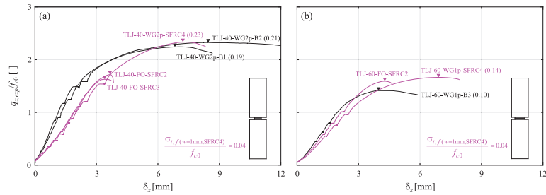
Fig. 6.7 - Comparison of joint tests made of SFRC (purple) and RC (black): (a) specimens with load concentration ratio b_y/b_y = 0.40 and (b) specimens with load concentration ratio b_y/b_y = 0.60 . Transverse mechanical reinforcement ratio \omega_{y,hyb} for hybrid and \omega_y for conventional reinforcement in brackets, where applicable.
