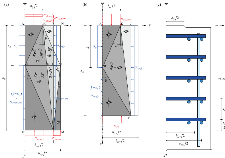
Fig. 5.8 - Modelling of longitudinal joints with stress fields: (a) Multi-Wedge stress field, (b) Dual-Wedge stress field, and (c) corresponding reinforcement layout for the half specimens of TLJ-40-WG2p-B1. Only one symmetrical half is shown. Transverse stresses are exaggerated compared to vertical stresses.
