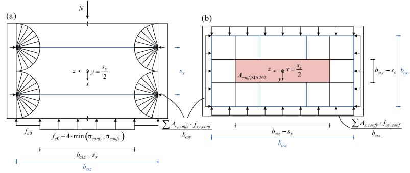
Fig. 2.3 - Definition of confined concrete area according to SIA 262: (a) stress field and (b) lateral section at the level of the confining reinforcement (e.g. x = s_x/2 ). Adapted and adjusted from Sigrist [18].
