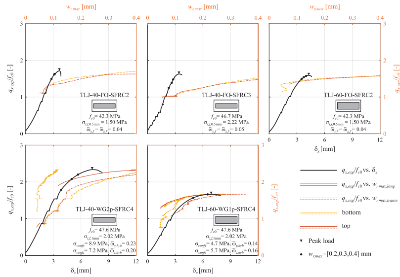
Fig. 6.3 - Load-compression and load-crack width diagrams for tests on longitudinal joints of tunnel lining segments.
