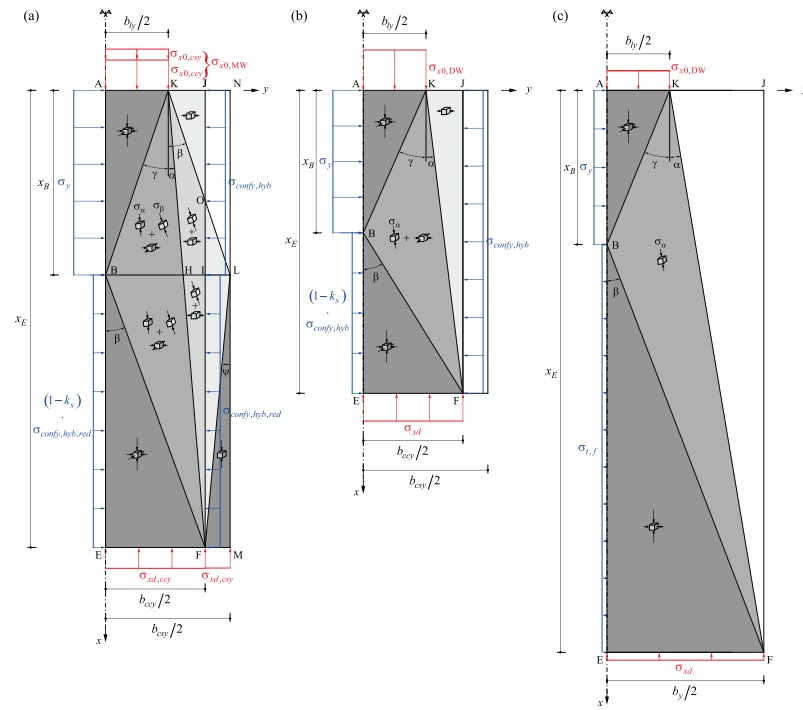
Fig. 6.9 - Models for strip-loaded SFRC: (a) Multi-Wedge stress field for hybrid-reinforced specimens, (b) Dual-Wedge stress field for hybrid-reinforced specimens, and (c) Dual-Wedge stress field for SFRC specimens without additional reinforcement. (a) and (b) drawn to scale for the specimen WG-SFRC1-1 and (c) for the specimen TLJ-40-FO-SFRC2. Only one symmetrical half is shown, and transverse stresses are exaggerated compared to vertical stresses. (a) and (b) with the same scaling to allow a direct comparison.
