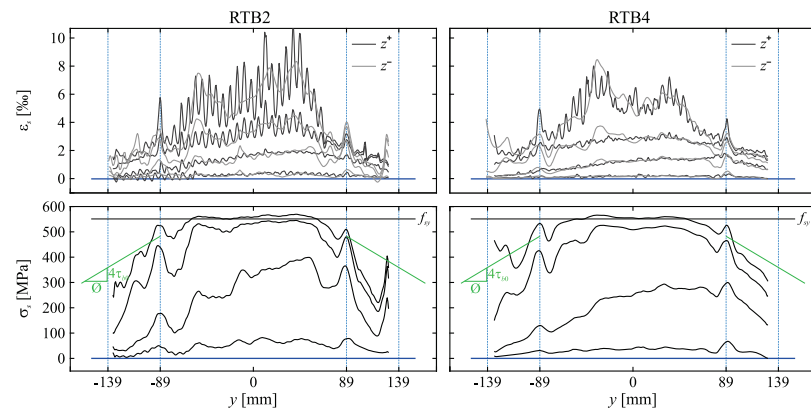
Fig. 3.5 - Results of FO measurements of the transverse reinforcing bars RTB2 and RTB4 showing the individual measured strains and the mean normal stresses for different load levels.
