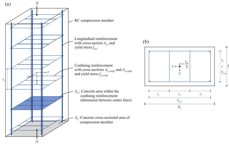
Fig. 2.1 - Definition of most important geometrical parameters used to account for passive confinement: (a) RC compression member ( s_x:s_z:s_y = 1:1:1.5 ) and (b) section at the level of confining reinforcement (e.g. x = s_x/2 ).
