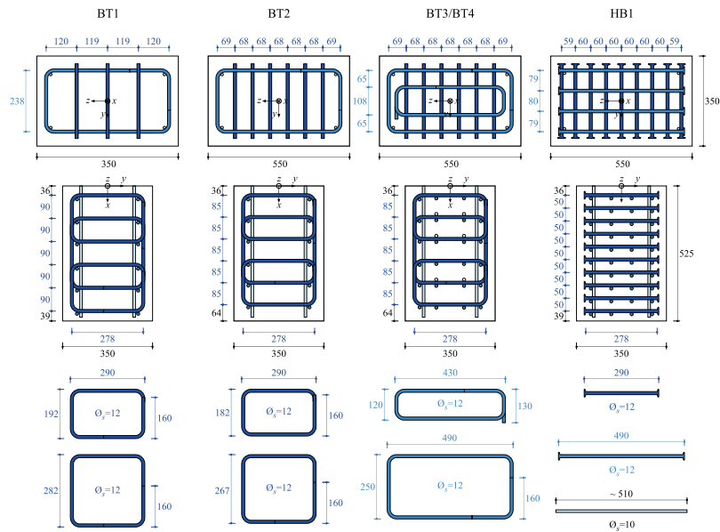
Fig. 4.8 - Reinforcement configurations of bent ties and double-headed bars (dimensions in mm). Top two rows show reinforcement spacings between centre lines, bottom two rows external dimensions. Three pairs of the inner longitudinal ties (shown without filling) were placed in BT4 but not in BT3.
