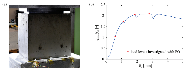
Fig. 3.1 - Experimental test: (a) partially loaded concrete specimen and (b) load-displacement diagram of test with indicated load levels used for the presentation of fibre optical measurements.
