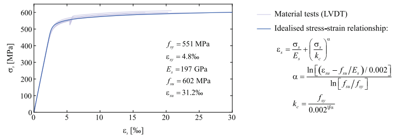
Fig. 3.3 - Material property of reinforcing bars used for welded grid reinforcement, showing material tests and idealised stress-strain relationship.
