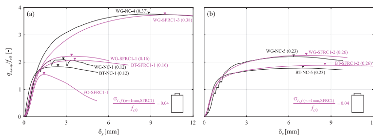
Fig. 6.6 - Comparison of SFRC (purple) and RC (black) block tests: (a) specimens with load concentration ratio b_y/b_x = 0.40 and (b) specimens with load concentration ratio b_y/b_x = 0.60 . Transverse mechanical reinforcement ratio \omega_{y,hyb} for hybrid and \omega_y for conventional reinforcement in brackets, where applicable.
