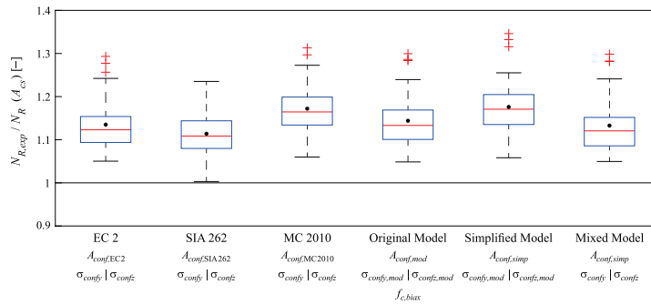
Fig. 2.9 - Comparison of the different models with the experimental data (40 specimens).
