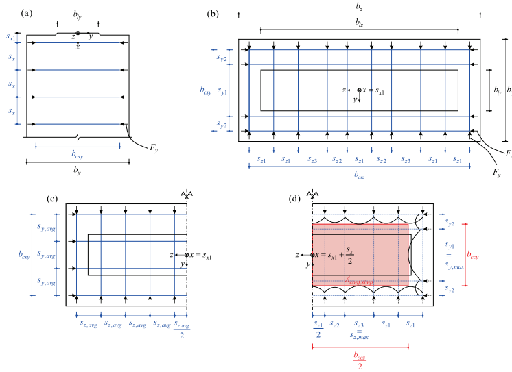
Fig. 5.A.1 - Definition of reinforcement spacings to determine the confinement properties: (a) vertical section, (b) horizontal section at the level of the confining reinforcement, (c) assumed average reinforcement spacings to compute confining stresses, and (d) confined concrete area determined based on maximum spacings in the respective directions. Adapted from Morger et al. [10].
