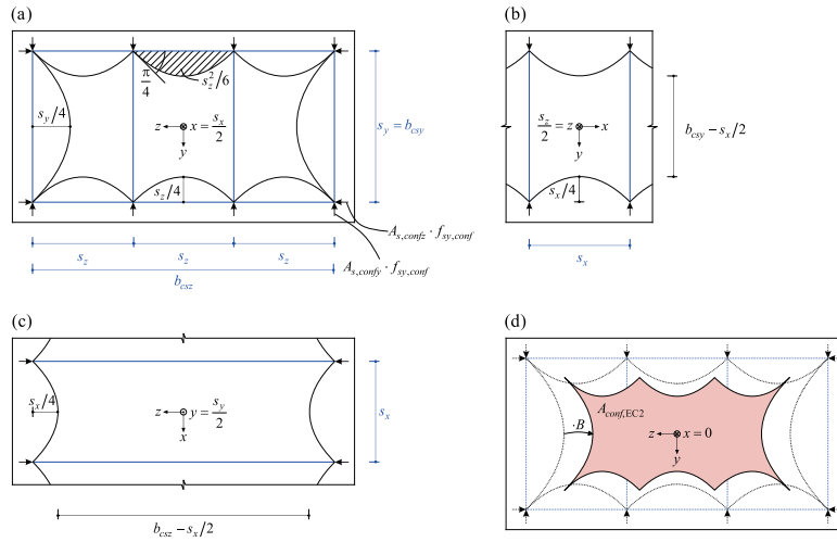
Fig. 2.2 - Definition of confined concrete area according to EC 2: (a) confined concrete area at the section of a confining reinforcement layer (e.g. x = s_x/2 ), (b) and (c) longitudinal dispersion of confining forces, and (d) governing confined concrete area at the centre between two confining reinforcement layers (e.g. x = 0 , dotted lines indicating section from (a) as reference).
