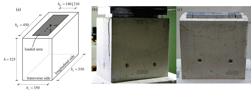
Fig. 4.6 - (a) Specimen geometry [mm], (b) test setup, and (c) tested specimen with steel bricks used for load introduction. Adapted from Morger and Kaufmann [24].
