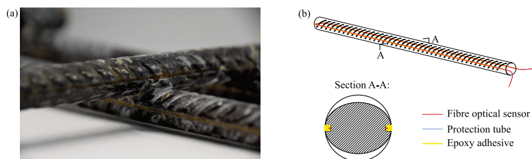
Fig. 3.4 - Instrumentation of welded reinforcement grid with FO: (a) welded cross joint with fibre optical sensors placed in the grooves and glued with epoxy resin and (b) schematic drawing of placing of fibre optical sensors on reinforcing bars (not to scale).
