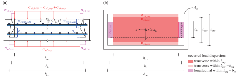
Fig. 5.9 - Load dispersion in longitudinal direction shown for the half specimens of TLJ-40-WG2p-B1: (a) vertical cut through centre with Dual-Wedge stress fields on the sides and (b) horizontal cut after load dispersion indicating the loaded areas. Transverse load dispersion considered according to the Multi-Wedge stress field.
