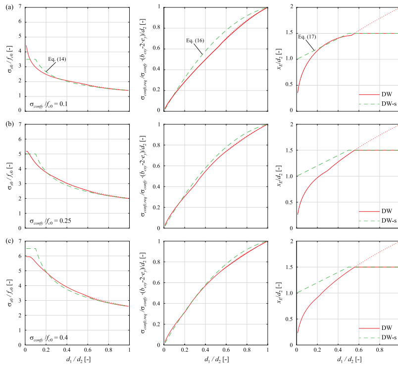
Fig. 4.A.1 - Comparison of Dual-Wedge stress field and the simplification for different mechanical confining reinforcement ratios.
