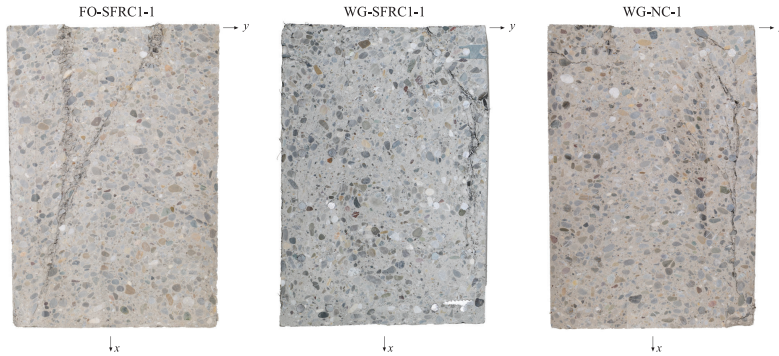
Fig. 6.4 - Vertical transverse cuts through three specimens after testing. Longitudinal DIC surface to the positive y side.
