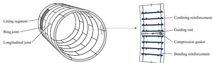
Fig. 1.2 - Definition of parameters of segmental tunnel linings and longitudinal joints.
