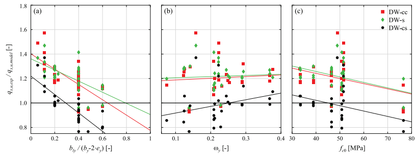
Fig. 4.12 - Comparison of experimental data with different model approaches based on the Dual-Wedge stress field plotted against (a) load concentration ratio b_y/(b_y - 2 \cdot e_y) , (b) transverse mechanical reinforcement ratio \omega_y , and (c) uniaxial concrete compressive strength f_{c0} .
