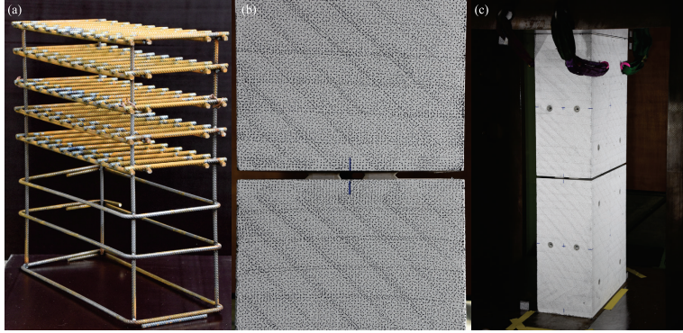
Fig. 5.3 - (a) Reinforcement configuration WG2p, (b) joint geometry TLJ-40g, and (c) test setup.
