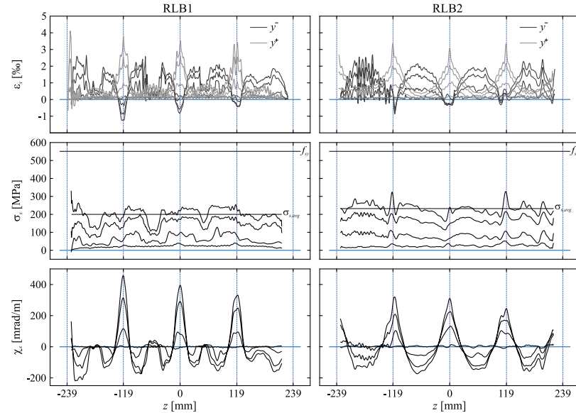
Fig. 3.6 - Results of FO measurements of the longitudinal reinforcing bars RLB1 and RLB2 showing the individual measured strains, the mean normal stresses and the curvatures.
