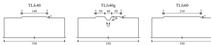
Fig. 5.2 - Joint geometries (dimensions in mm).
