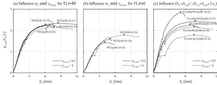
Fig. 5.6 - Normalised stress-compression diagrams for all tests investigating different influences: (a) mechanical transverse reinforcement ratio \omega_y and confined height x_{E,max} for tests with joint geometry TLJ-40, (b) mechanical transverse reinforcement ratio \omega_y and confined height x_{E,max} for specimens with joint geometry TLJ-60, and (c) load concentration ratio given by the joint type. The value of the respective influence parameter is indicated in brackets or by the legend. For more detailed information on the specimens, see Table 5.1.
