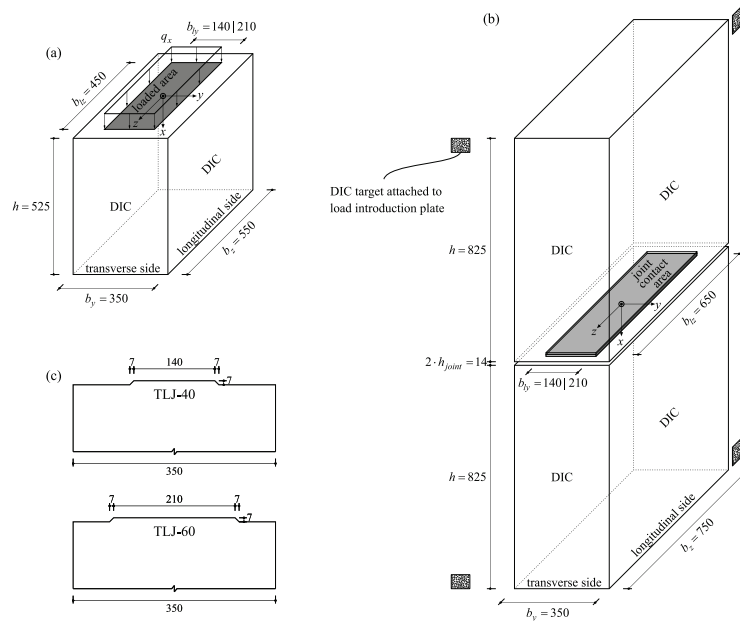
Fig. 6.1 - Geometry of the specimens (dimensions in mm): (a) block specimen, (b) longitudinal joint specimens, and, (c) joint geometry. Adapted from Morger et al. [3], [15].
