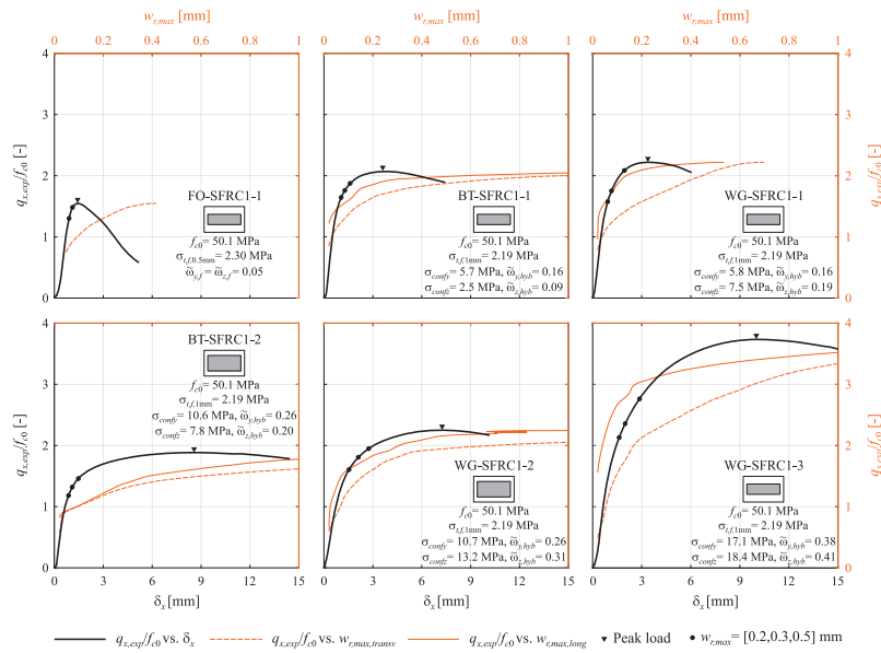
Fig. 6.2 - Load-compression and load-crack width diagrams for strip-loaded SFRC block specimens.
