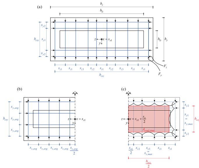
Fig. 4.4 - Confinement properties for irregular reinforcement spacings: (a) horizontal section at the level of the confining reinforcement with irregular reinforcement spacings in the transverse and longitudinal directions, (b) assumed average reinforcement spacings to compute confining stresses, and (c) confined concrete area determined based on maximum spacings in the respective directions.
