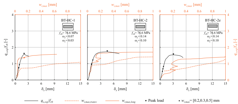
Fig. 4.C.2 - Load-penetration and load-crack width diagrams for high strength concrete specimens.
