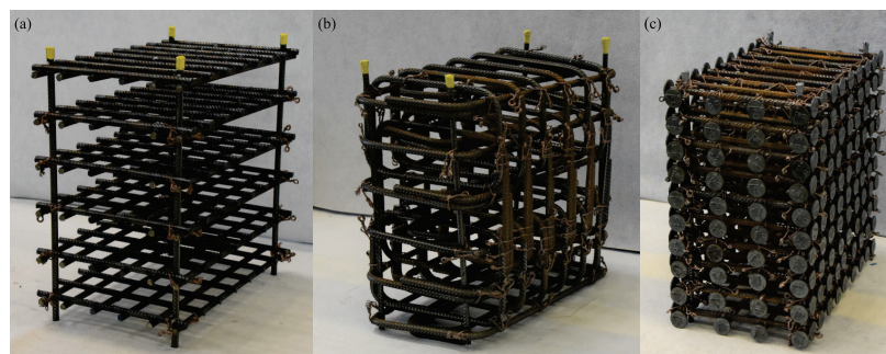
Fig. 4.7 - Reinforcement configurations: (a) welded grids (WG3), (b) bent ties (BT3) and (c) double-headed bars (HB1) [24].
