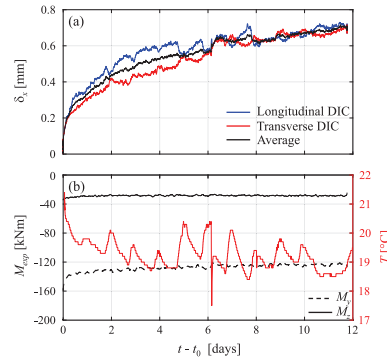
Fig. 5.D.1 - Creep investigation of TLJ-60-WG2f-B4: (a) Creep deformation determined with transverse and longitudinal DIC systems separately and average value and (b) bending moments M_y and M_z , respectively, and temperature T in the construction hall. All values plotted versus time t - t_0 , with t_0 = 215 days.
