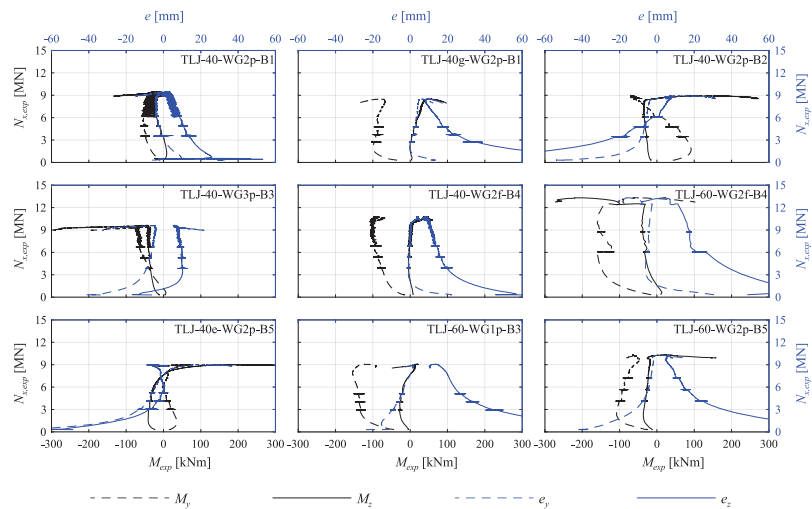
Fig. 5.C.1 - Measured bending moments and calculated load eccentricity at lower load introduction plate.
