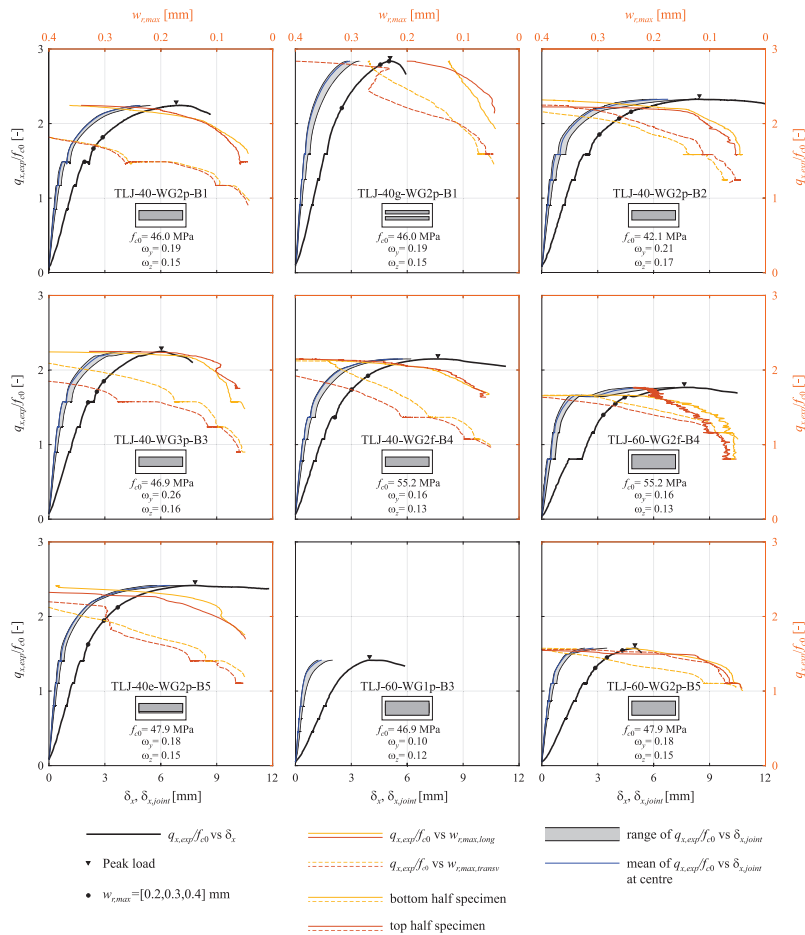
Fig. 5.5 - Load-bearing behaviour: Normalised stress-compression, normalised stress-joint closing, and normalised stress-crack width diagrams for tests on longitudinal joints of tunnel lining segments.
