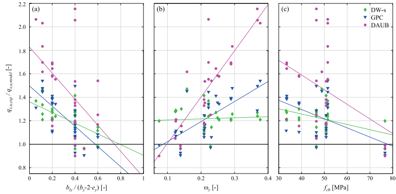
Fig. 4.13 - Comparison of experimental data with model predictions plotted against (a) load concentration ratio b_b/(b_f - 2e_y) , (b) transverse mechanical reinforcement ratio \omega_y , and (c) uniaxial concrete compressive strength f_{c0} .
