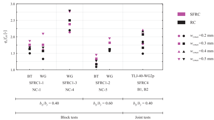
Fig. 6.8 - Load levels for a given crack width for SFRC and RC specimens of block and joint tests. RC specimens from Morger et al. [3], [15].
