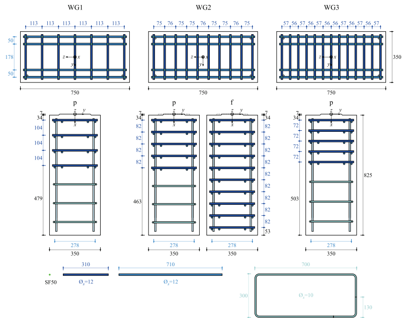
Fig. 5.4 - Configurations of welded grids (upper rows centre-line spacings, bottom row external dimensions, both in mm).
