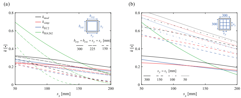
Fig. 2.7 - Comparison of the effectiveness factor k of the different model approaches: (a) RC member with one stirrup and varying cross-section and (b) RC member with fixed cross-section but varying reinforcement spacings.
