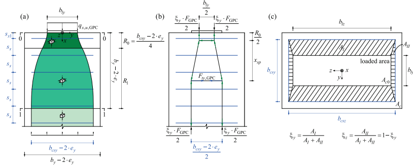
Fig. 4.5 - Geometric and passive confinement model: (a) definition of the two control sections, (b) determination of bursting force F_y with strut-and-tie model, and (c) definition of \xi_y and \xi_z determining the load spreading in the two lateral directions.
