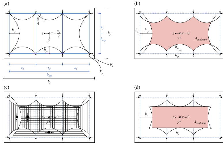
Fig. 2.6 - Different cross-sections of the compression member (Fig. 2.4) illustrating the confined concrete area according to the new model: (a) section at the level of the confining reinforcement (e.g. x = s_z/2 ), (b-d) sections at the centre between the confining reinforcement layers (e.g. x = 0 ), with (b,c) governing confined concrete area indicating (b) dimensions and (c) different stress states, and (d) simplified governing confined concrete area.
