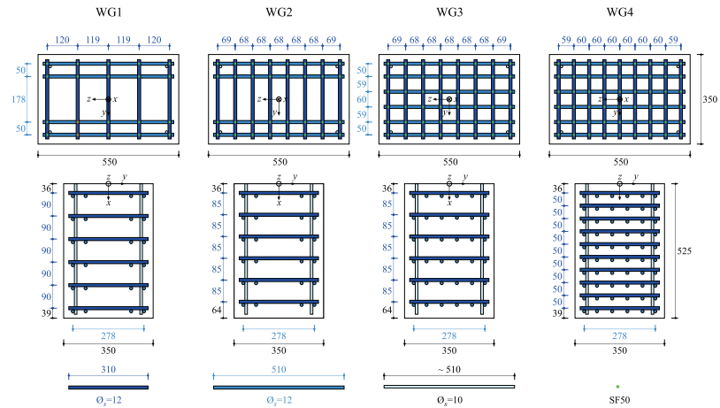
Fig. 4.9 - Reinforcement configurations of welded grids (dimensions in mm). Top two rows show reinforcement spacings between centre lines, bottom row external dimensions.
