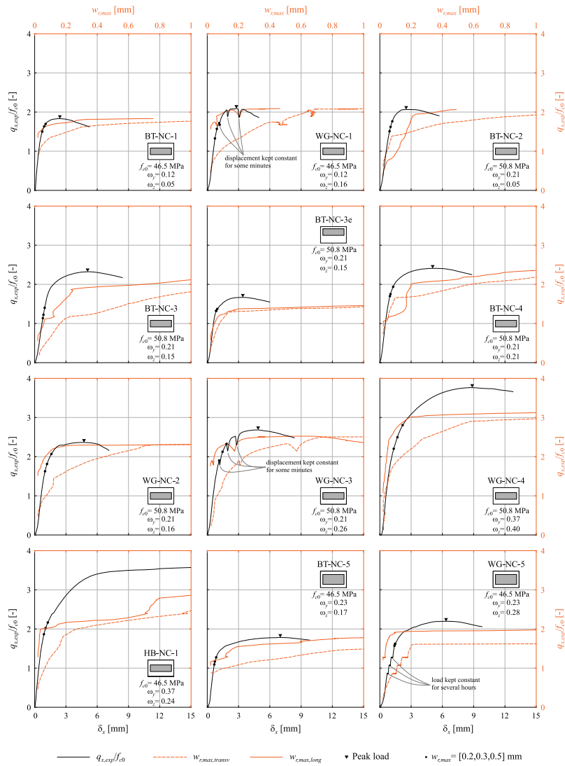
Fig. 4.C.1 - Load-penetration and load-crack width diagrams for normal strength concrete specimens.
