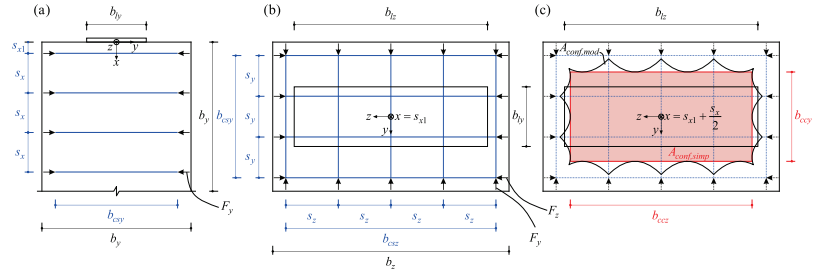
Fig. 4.3 - Confinement properties for regular reinforcement spacings: (a) vertical section, (b) horizontal section at the height of a reinforcement layer, and (c) horizontal section at the centre between two reinforcement layers.
