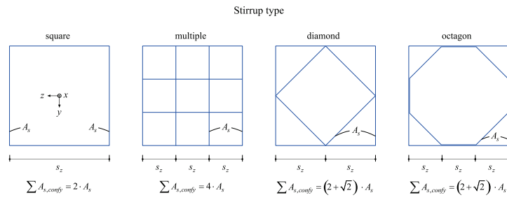
Fig. 2.A.1 - Definition of stirrup types.
