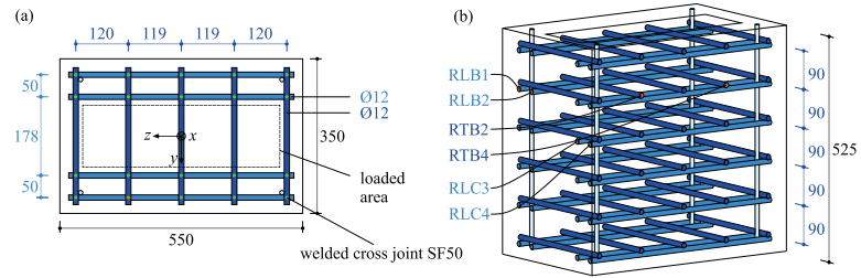
Fig. 3.2 - Reinforcement of welded grids: (a) grid with positions of welded cross joints and dimensions and (b) reinforcement layout of the specimen [mm].
