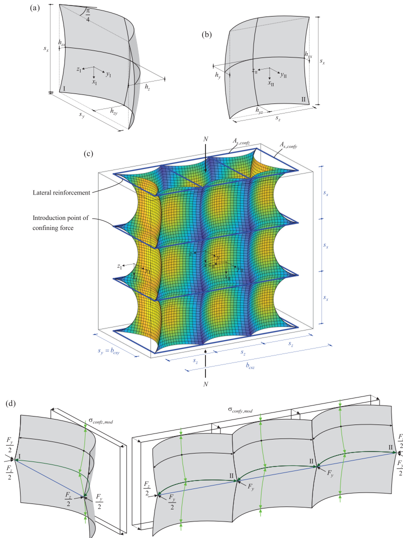
Fig. 2.4 - Definition of confined concrete volume in a rectangular compression member assuming s_x:s_z:s_y = 1:1:1.5 : (a) definition of paraboloid I, (b) definition of paraboloid II, (c) triaxially confined concrete volume, and (d) force flow.
