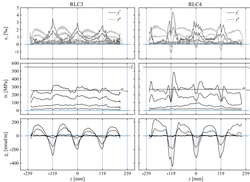
Fig. 3.7 - Results of FO measurements of the longitudinal reinforcing bars RLC3 and RLC4 showing the individual measured strains, the mean normal stresses and the curvatures.
