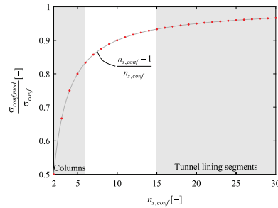
Fig. 2.5 - Comparison of the confining stresses resulting from determination with current guidelines ( \sigma_{conf} ) and the new model proposal ( \sigma_{conf,mod} ) depending on the number of confining reinforcement legs ( n_{s,conf} ).
