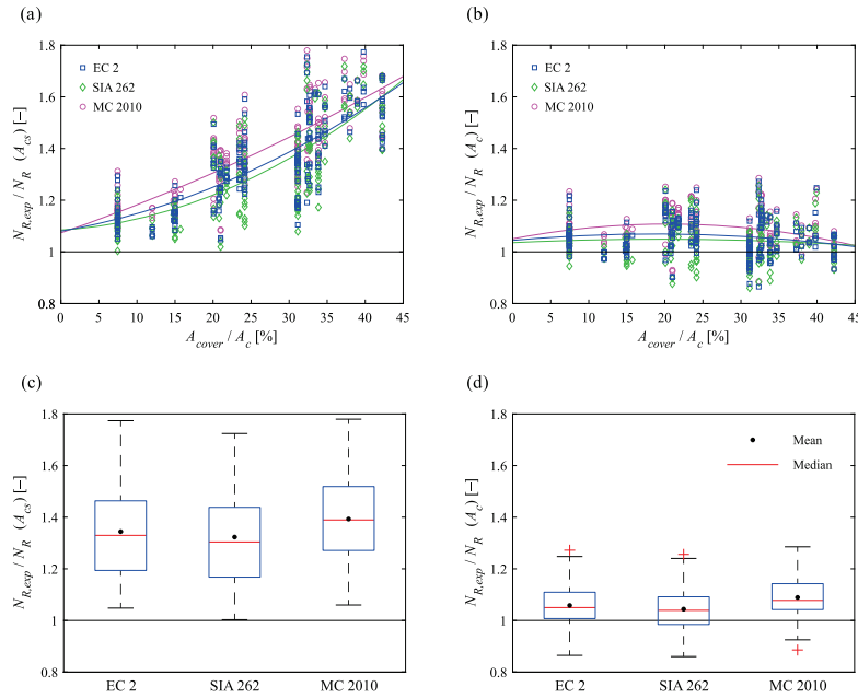
Fig. 2.8 - Impact of the cover concrete on the load-bearing capacity prediction N_R of current standards (EC 2, SIA 262 and MC 2010) and comparison with experimental results (193 specimens): (a) cover concrete neglected, (b) cover concrete considered with uniaxial concrete compressive strength, (c) box plot associated with (a), and (d) box plot associated with (b).
