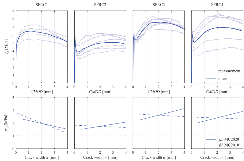
Fig. 6.A.1 - Classification of residual post-cracking strength of different SFRC batches.
