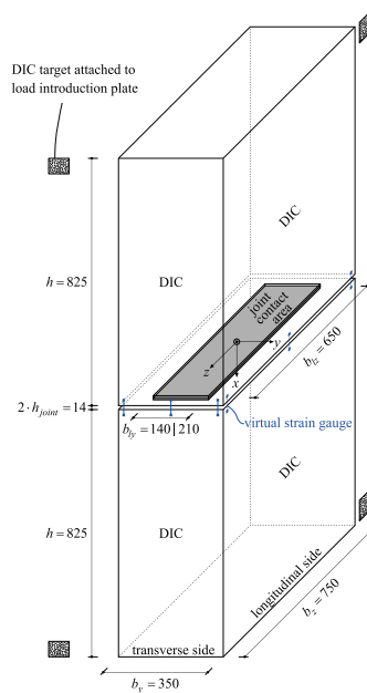
Fig. 5.1 - Geometry of the specimens (dimensions in mm).
