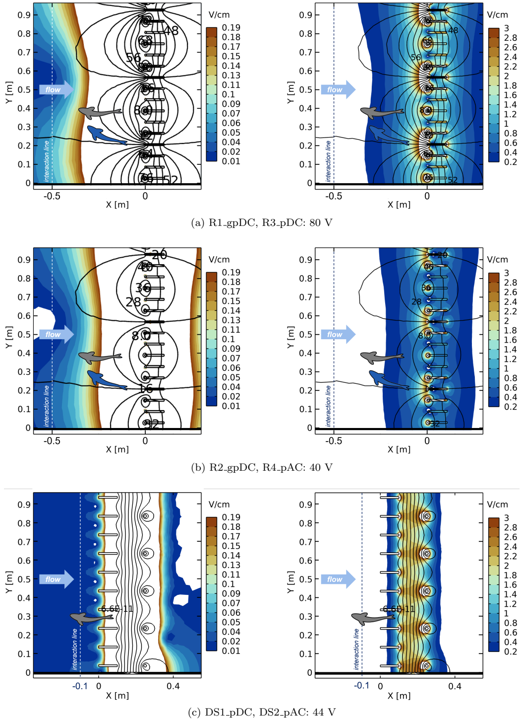
Figure 4. Numerical simulation of the electric field for the experimental groups R1_gpDC - R4_pAC and DS1_pDC - DS2_pAC. The field is simulated as a horizontal cut at the flume bottom. The left and right column show a low and high range of the voltage gradient, respectively. White areas are either below or above the respective colour scale. Black lines indicate equipotential lines (i.e., constant voltage) with a distance of 4 V.
