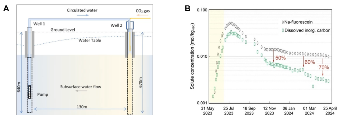
Figure 8. A) Well-doublet injection scheme at the Jizan site in which groundwater from the reservoir is extracted from Well 1 and reinjected together with \text{CO}_2 into the reservoir through Well 2. The two fluids mix completely within the well before entering the reservoir. The inert, non-adsorbing tracer Na-fluorescein was co-injected with the same concentration as \text{CO}_2 . After Ahmed et al. (submitted). (B) Analyses of dissolved inorganic carbon (DIC; sum of all dissolved species of \text{CO}_2 ) and of Na-fluorescein in water extracted from Well 1 as a function of monitoring time. Note that y-axis is logarithmic. Injection of \text{CO}_2 began on 31 May 2023 and continued for one month (pale yellow region). Groundwater flow carried the injected solution towards well 1, consistent with the rise of DIC sampled at well 1 (peak in late July, 2023). Decay of DIC thereafter is due to dispersion of flow. The evolution of Na-fluorescein concentrations tracks the migration of injected \text{H}_2\text{O} through the reservoir. The deficit in aqueous \text{CO}_2 (DIC) with respect to Na-fluorescein points to removal of \text{CO}_2 from the solution by precipitation of carbonate minerals.
