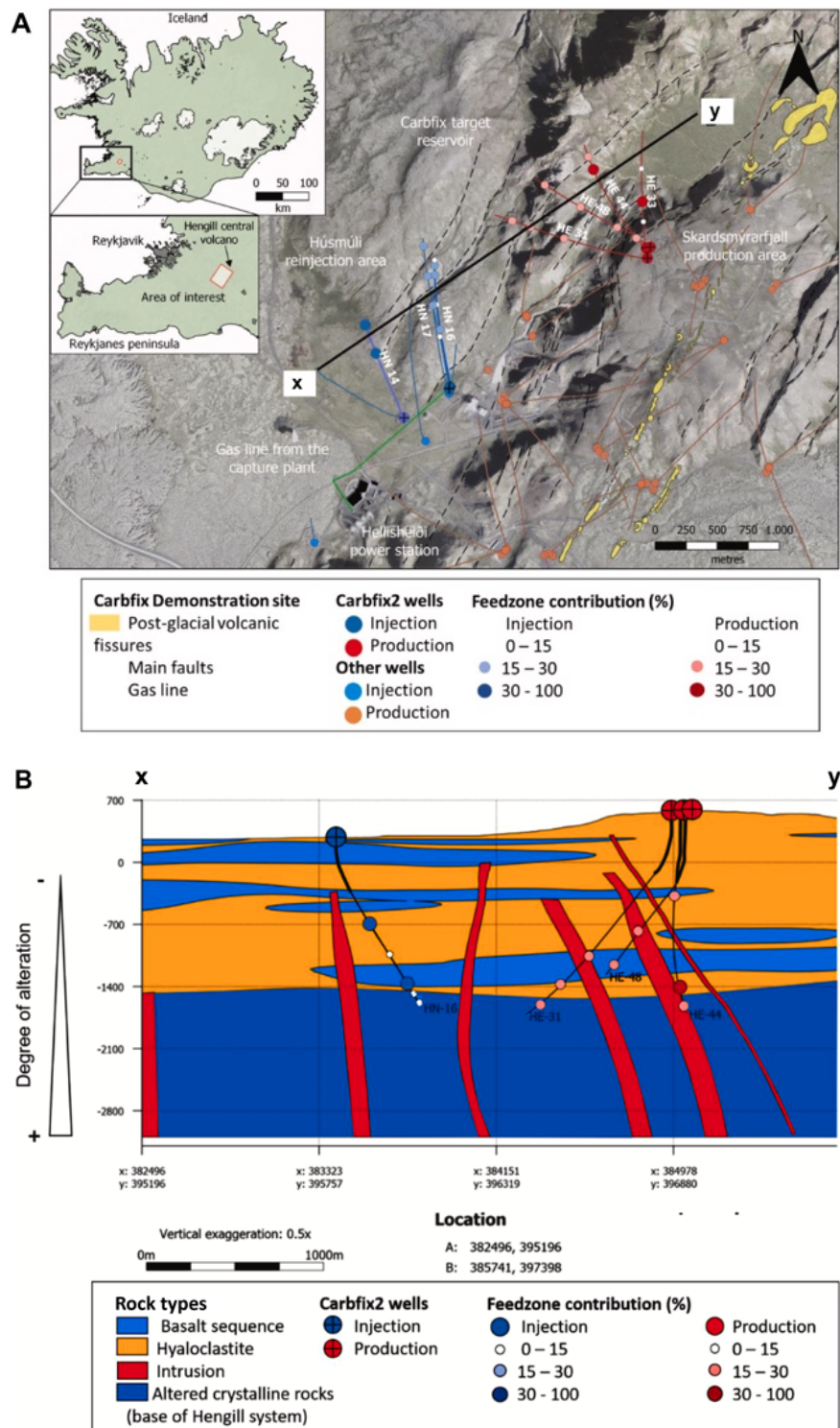
Figure 3. (A) Location of CarbFix2 injection sites in a barren basalt lava field, 20 km east of Reykjavík. The source of the CO 2 for injection is the Hellisheiði geothermal power plant (bottom centre of Fig.). The original CarbFix pilot site was located 2 km SW of the power plant. (B) Vertical cross-section along the line x–y in panel A, showing injection and production wells. The target aquifer for CO 2 injection is the stack of lavas (basalt and glassy hyaloclastite) between 700 and 1400 m depth. Modified (labels adjusted) after Ratouis et al. (2022).
