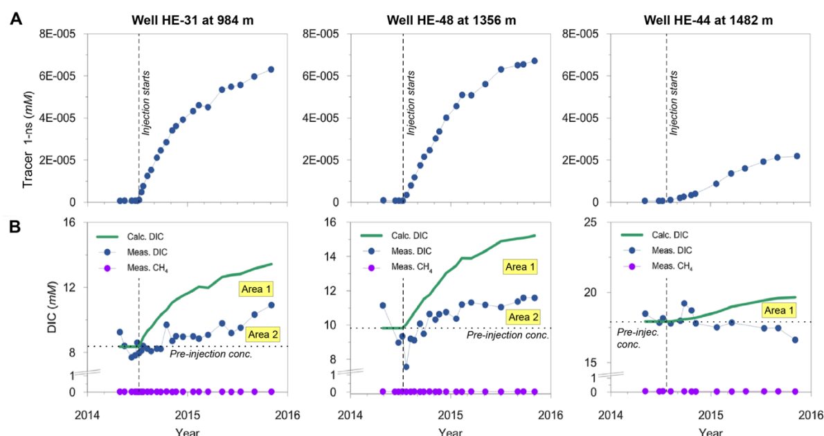
Figure 5. Principal proof for permanent, in-situ mineralization of \text{CO}_2 in the CarbFix2 project, based on chemical analyses at the wellheads of three production wells (HE-31, HE-48 and HE-44) over a two-year period. (A) Time-series analyses of a non-reactive, non-sorbing, temperature-resistant tracer (1-naphthalenesulfonate) that had been co-injected with the \text{CO}_2 -bearing solution. These data track the breakthrough of the injected fluid into the production wells, and enable quantification of the dispersion and mixing of the injected fluid as it migrates through the basalt reservoir. (B) Chemical analyses of the concentration of \text{CO}_{2(\text{aq})} (expressed as total Dissolved Organic Carbon, DIC) in samples taken in a time series over ~1.5 years at the wellheads of the three production wells. Green curve: hypothetical behaviour assuming no carbonate precipitation has occurred in the reservoir (based on the tracer behaviour in panel A). Blue dots: observed concentrations. The differences in behaviour of the three sampled wells are ascribed to their differing distances from the injection well (cf. Fig. 4: fluid travel times to the injection wells are 130 days to HE-31, 163 days to HE-48 and 272 days to HE-44). The purple dots show methane concentrations, ruling out any loss of \text{CO}_{2(\text{aq})} by chemical reduction. Between the green curve and blue dots, “Area 1” (labelled for this report) indicates the amount of \text{CO}_{2(\text{aq})} that has been lost from the injected fluid. Between the blue dots and the pre-injection concentration (dashed line), “Area 2” indicates the amount of \text{CO}_{2(\text{aq})} that has passed through the production well and degassed to the atmosphere at the wellhead. Modified (labels and guidelines added) after Gunnarsson et al. (2018).
