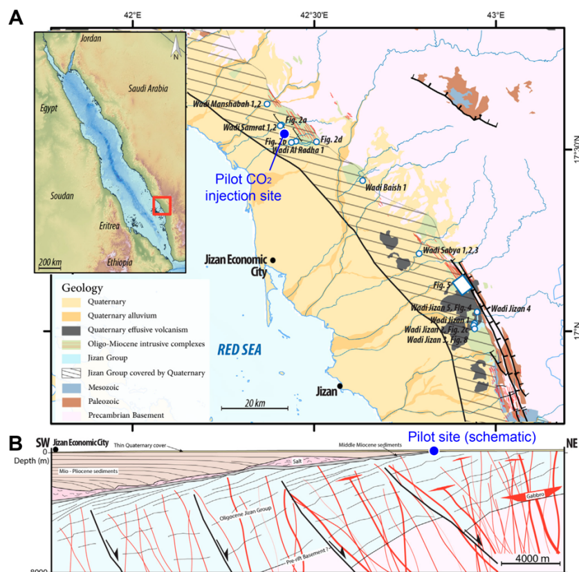
Figure 7. Location and geological setting of the Jizan in-situ mineralization pilot project. (A) The reservoir basalts into which CO 2 was injected belong to the SW-dipping Jizan Group. These are locally overlain by 10,000 year-old “Quaternary effusive” basalts. (B) Vertical cross-section from Jizan Economic City to the NE. Jizan Group basalts are cut by Quaternary basalt feeder dikes (red) and inferred faults. The basaltic dikes induced hydrothermal alteration and clogging of the rock-matrix pores in the older Jizan Group basalts. Location of pilot site is projected into the cross-section. Modified (labels added) after Fedorik et al. (2023).
