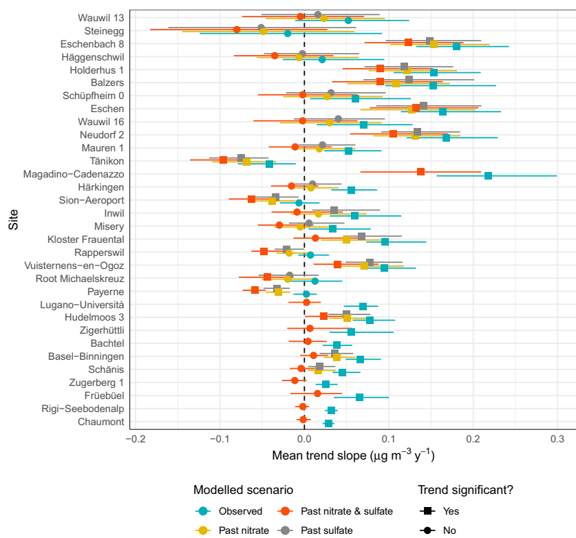
Fig. A9. ISORROPIA II-derived \text{NH}_3 trend slopes for four scenarios between 2004 and 2021 for 32 sampling locations in Switzerland and Liechtenstein. The sites are ordered by their mean \text{NH}_3 concentration.
