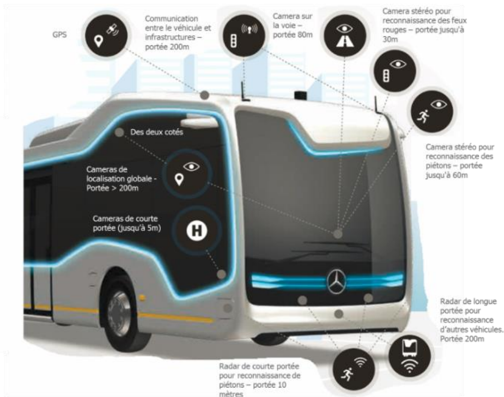
Image 4 : Future Bus and its various sensors.
