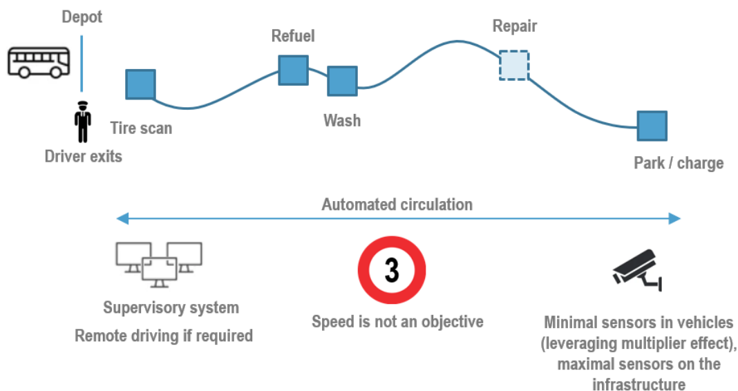
Image 15 : Diagram of the "AutoDepot" Technical Concept
