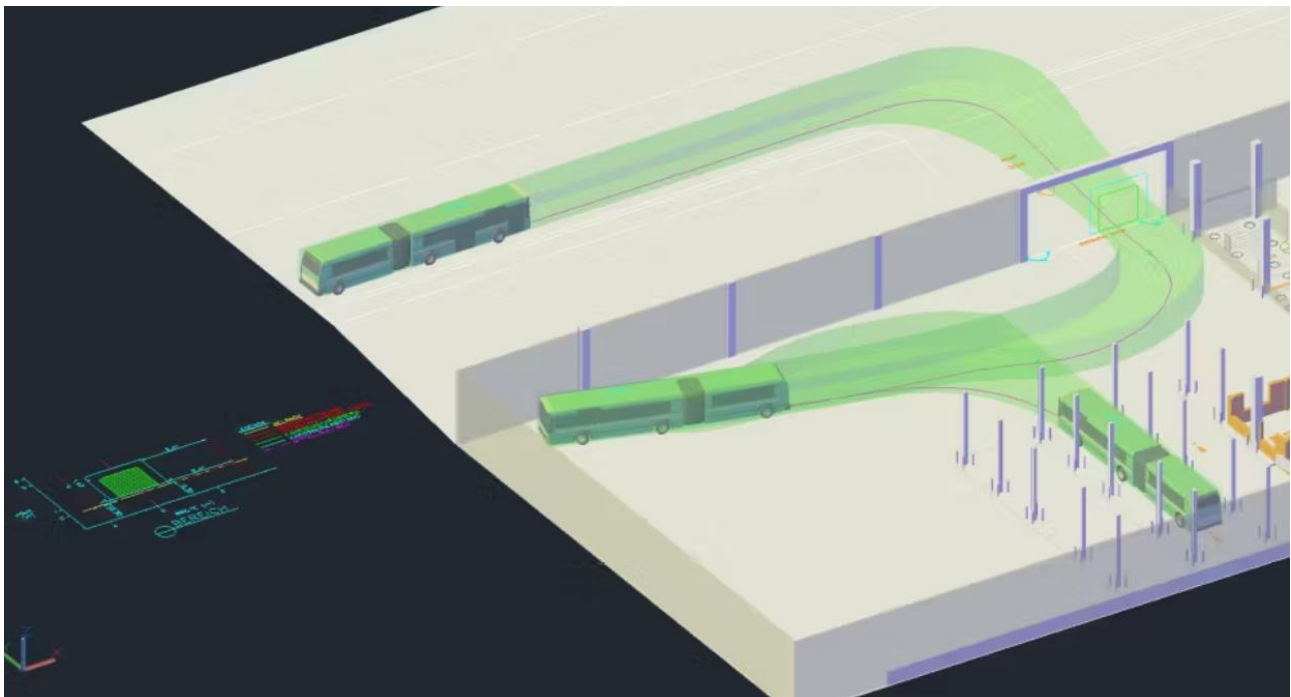
Image 11 : An example of verifying vehicle turning, including in three-dimensional mode. Source: Capterra.fr with AutoTurn Pro
