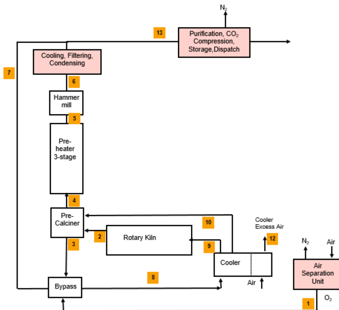
Figure 7. Lägerdorf oxyfuel design – Version 1.
