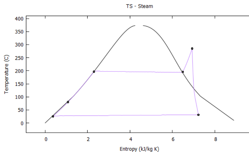
Figure 21. T-s diagram of the Rankine cycle.
