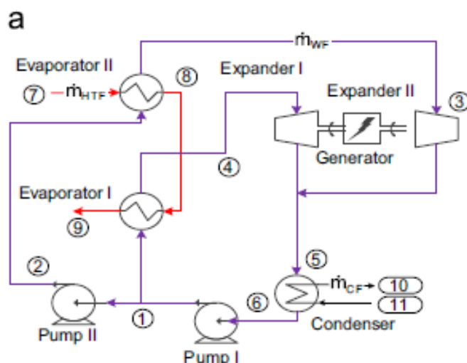
Figure 15. Dual pressure ORC [16].
