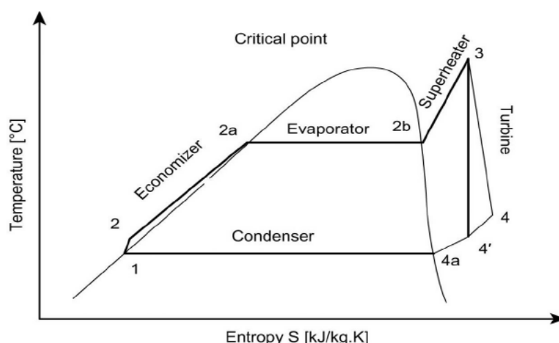
Figure 13. T-s diagram for R134a [30].
