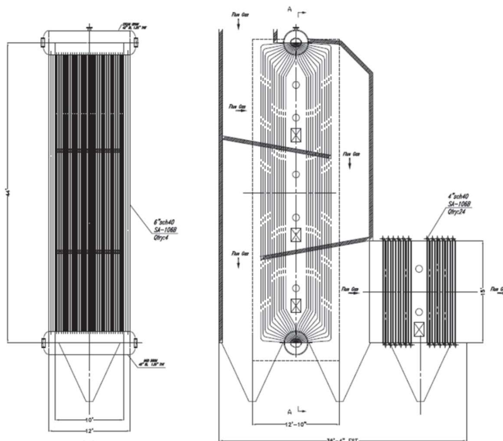
Figure 20. Vertical boiler arrangement illustrating downflow design, water in tubes, bottom hopper and sootblowing passages [41].
