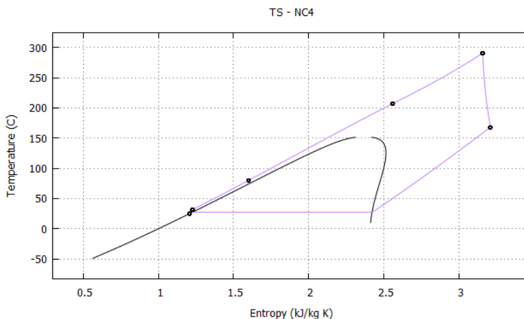
Figure 25. T-s diagram of ORC using butane.
