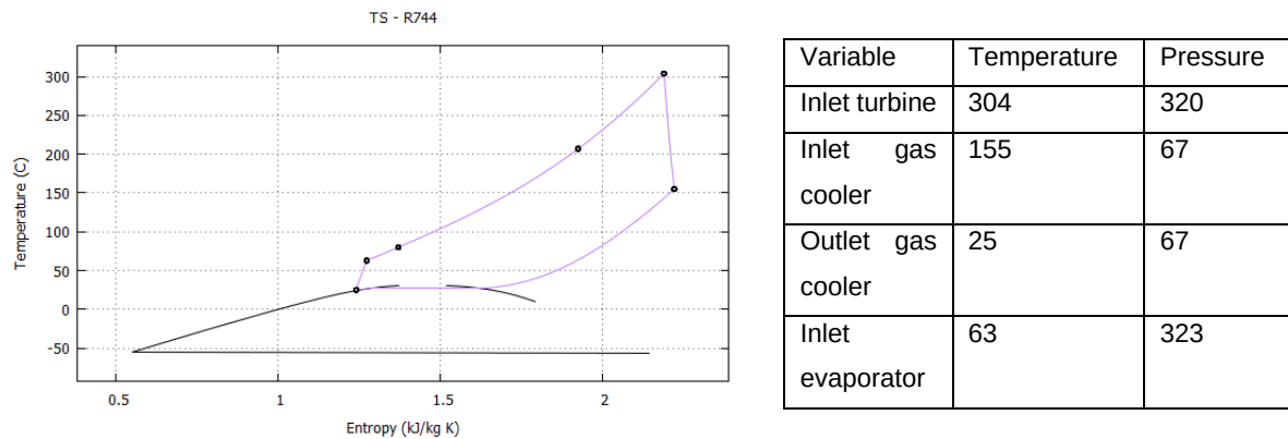
Figure 26. T-s diagram and process data of tCO 2 Rankine cycle.
