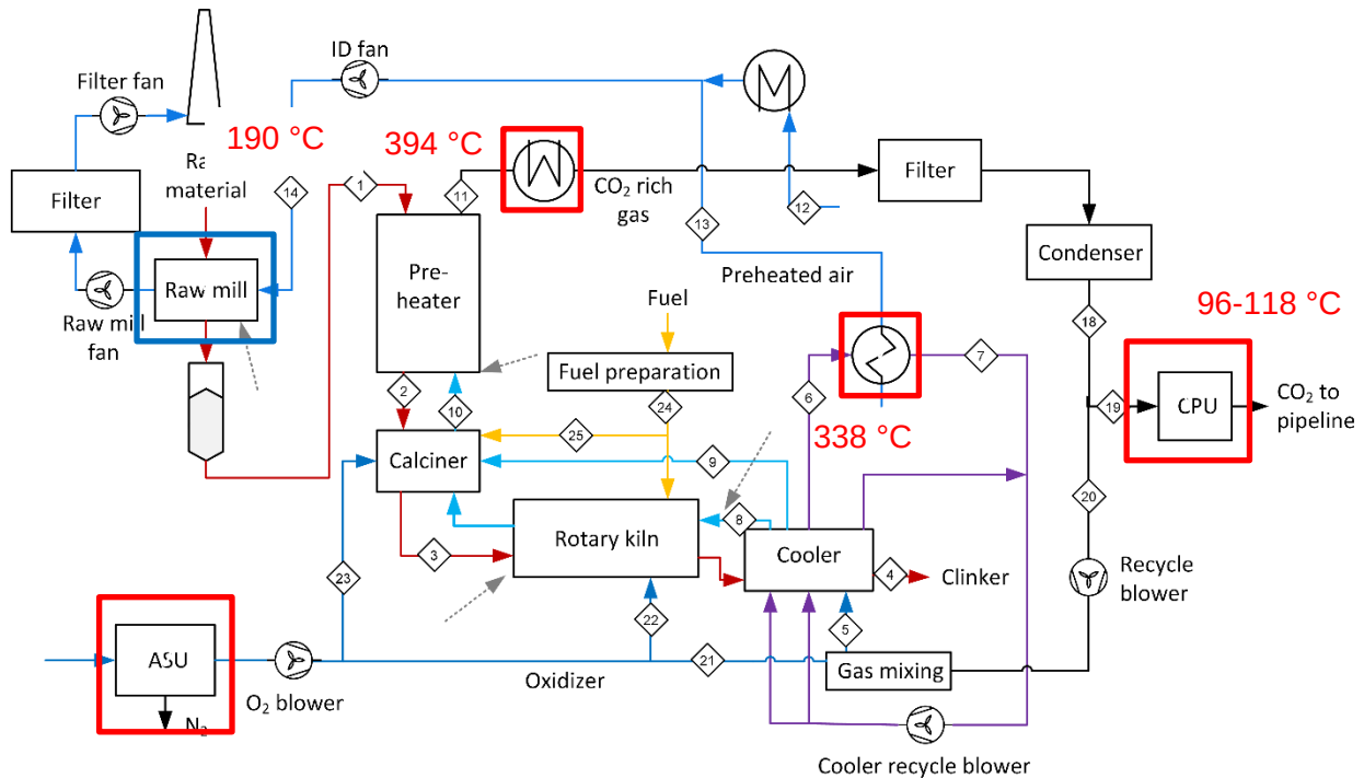
Figure 4. Schematic overview of the Oxyfuel BAT plant with indicated heat sources and sinks.
