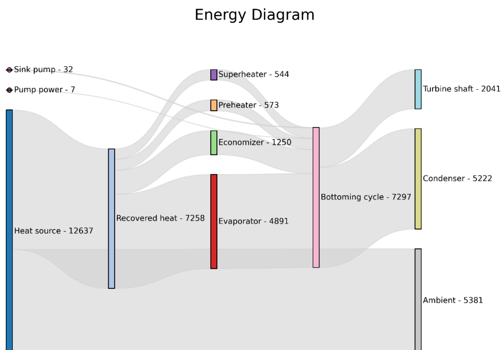
Figure 22. Energy diagram of steam RC.
