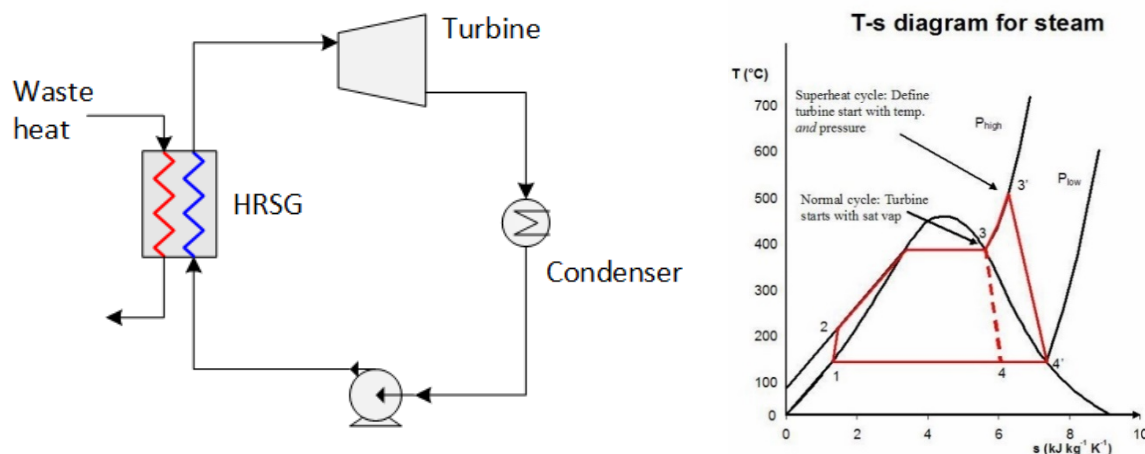
Figure 9. Schematic diagram and T-s diagram of a steam Rankine cycle.
