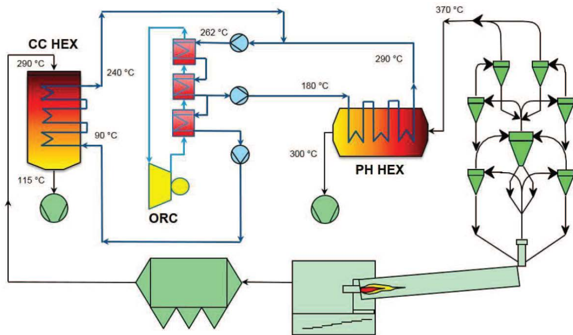
Figure 18. ORC waste heat recover system [55].
