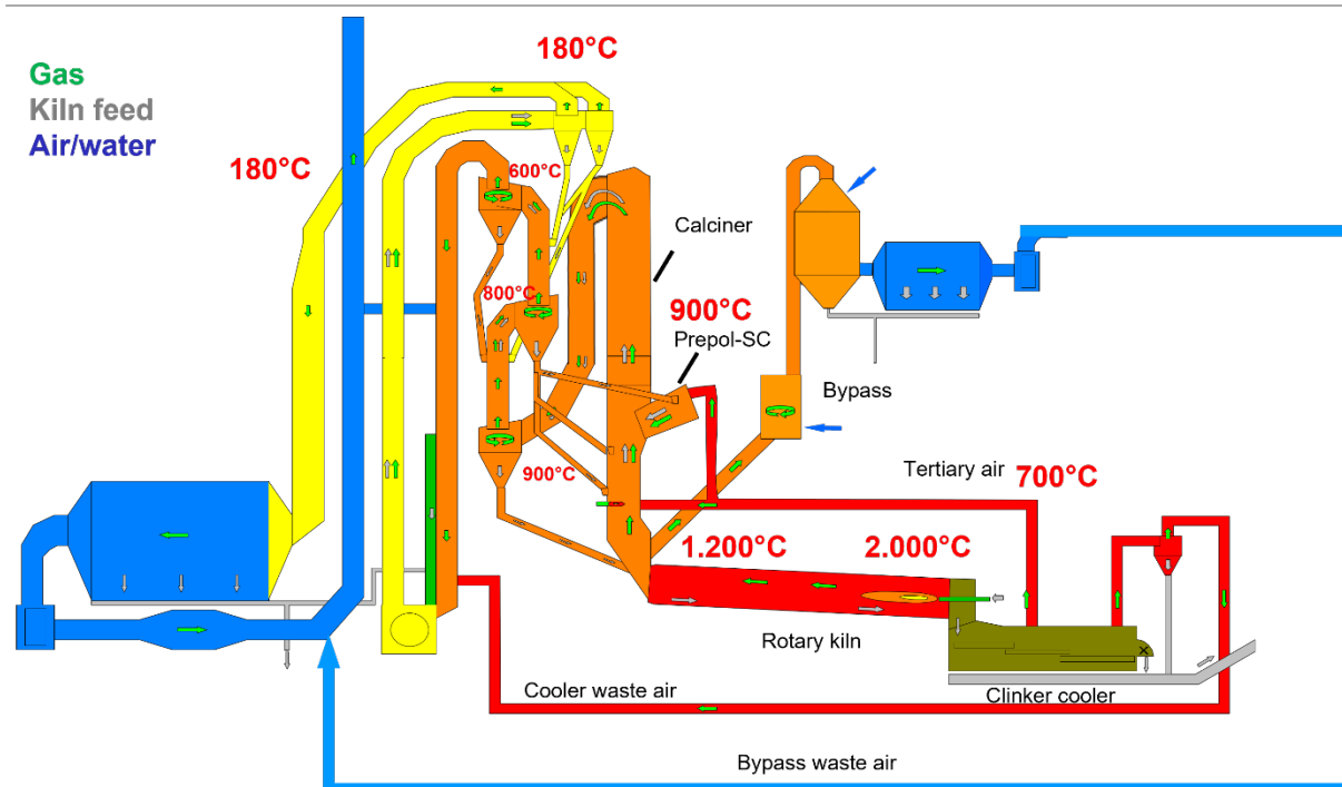
Figure 6. Schematic overview of the Lägerdorf plant.
