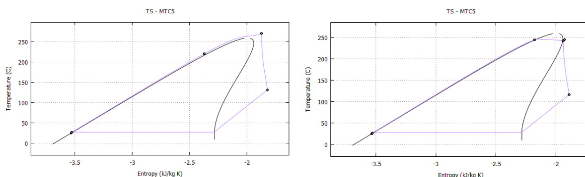
Figure 24. T-s diagram of ORC using methylcyclopentane. Left transcritical; Right subcritical
