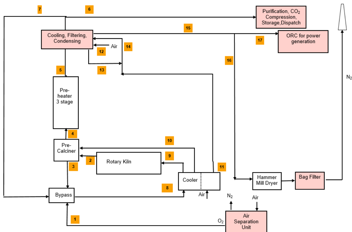
Figure 8. Lägerdorf oxyfuel design – Version 2.
