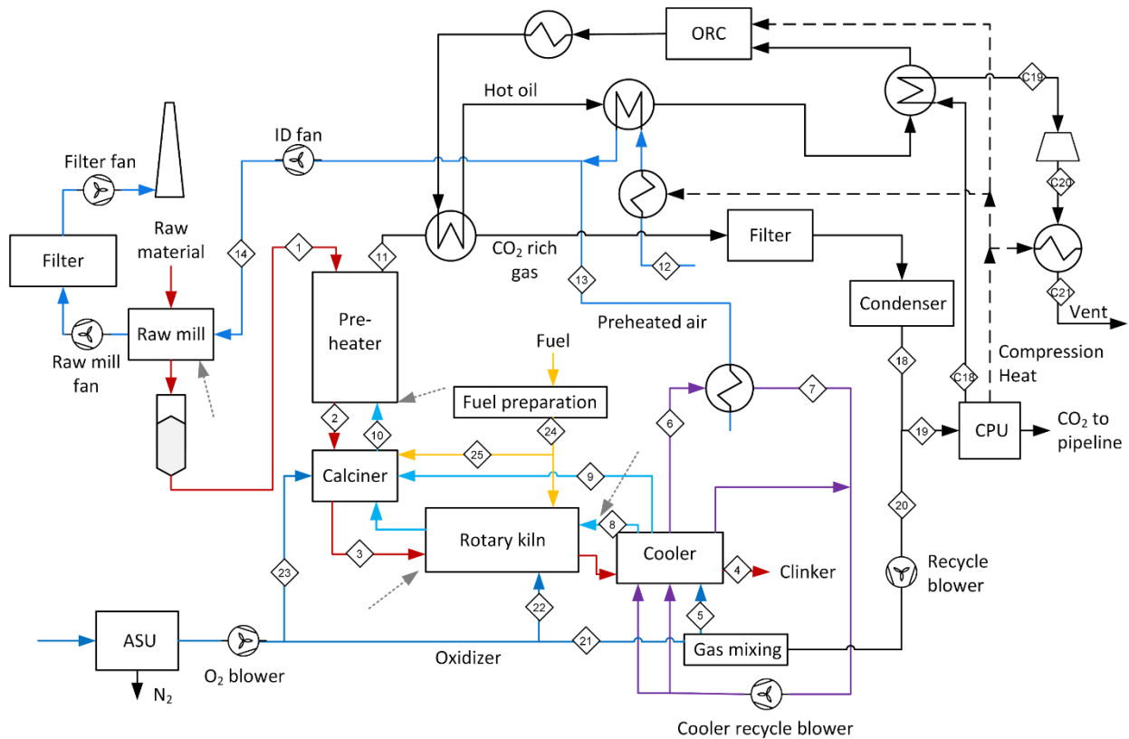
Figure 5. Schematic overview of the BAT oxyfuel cement plant with integration of ORC.
