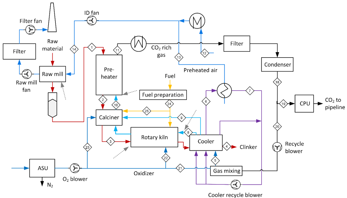
Figure 3. Schematic overview of the oxyfuel BAT cement plant configuration investigated in CEMCAP.
