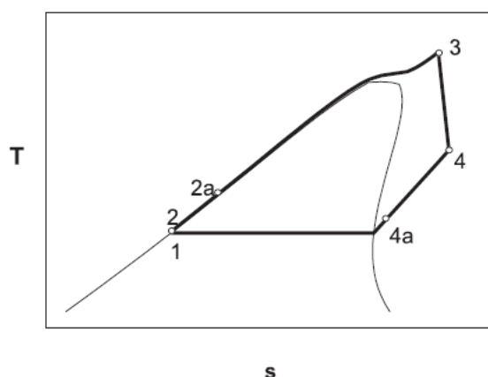
Figure 14. T-s diagram where the maximum pressure is supercritical [32].
