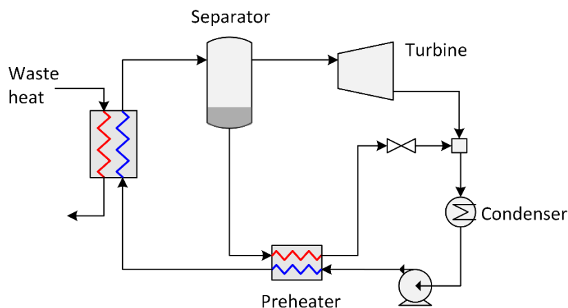
Figure 12. Schematic diagram of a basic Kalina cycle.
