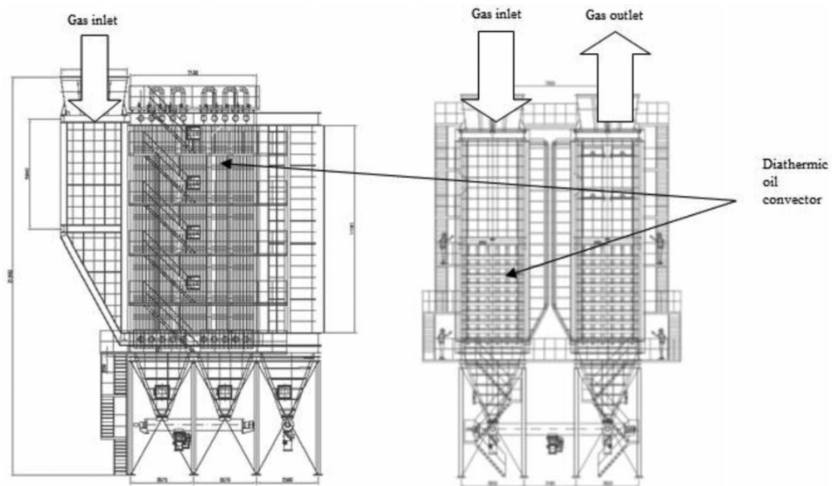
Figure 16. Heat exchanger and convectors to recuperate heat from the kiln gases [61].
