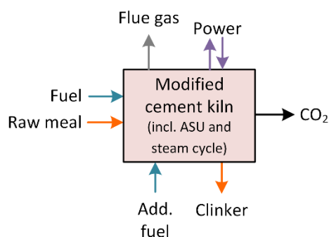
Figure 1. Schematic overview of the integration of the oxyfuel process with a cement kiln.
