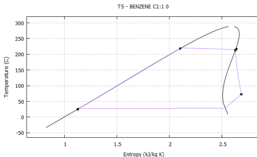
Figure 23. T-s diagram of the ORC with working fluid benzene.
