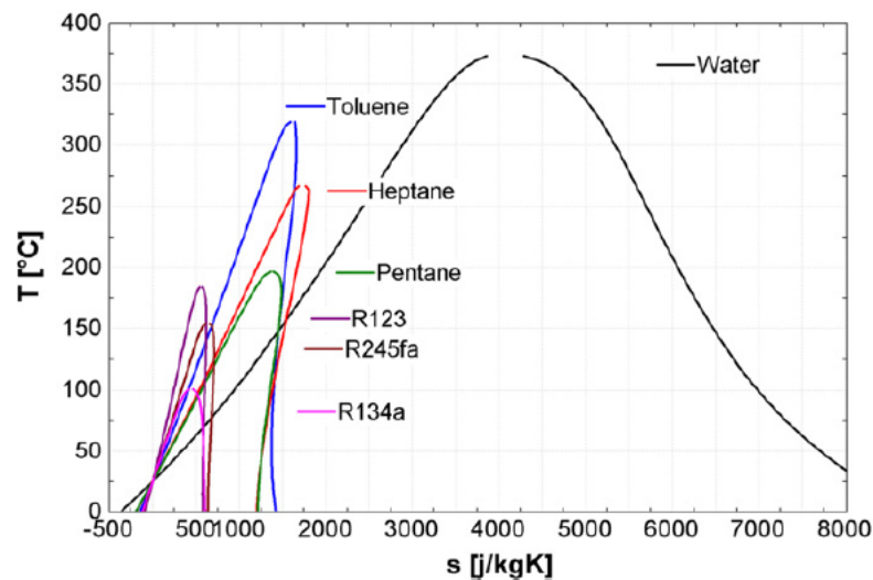
Figure 10. T-s diagram of water and various typical ORC working fluids [7].
