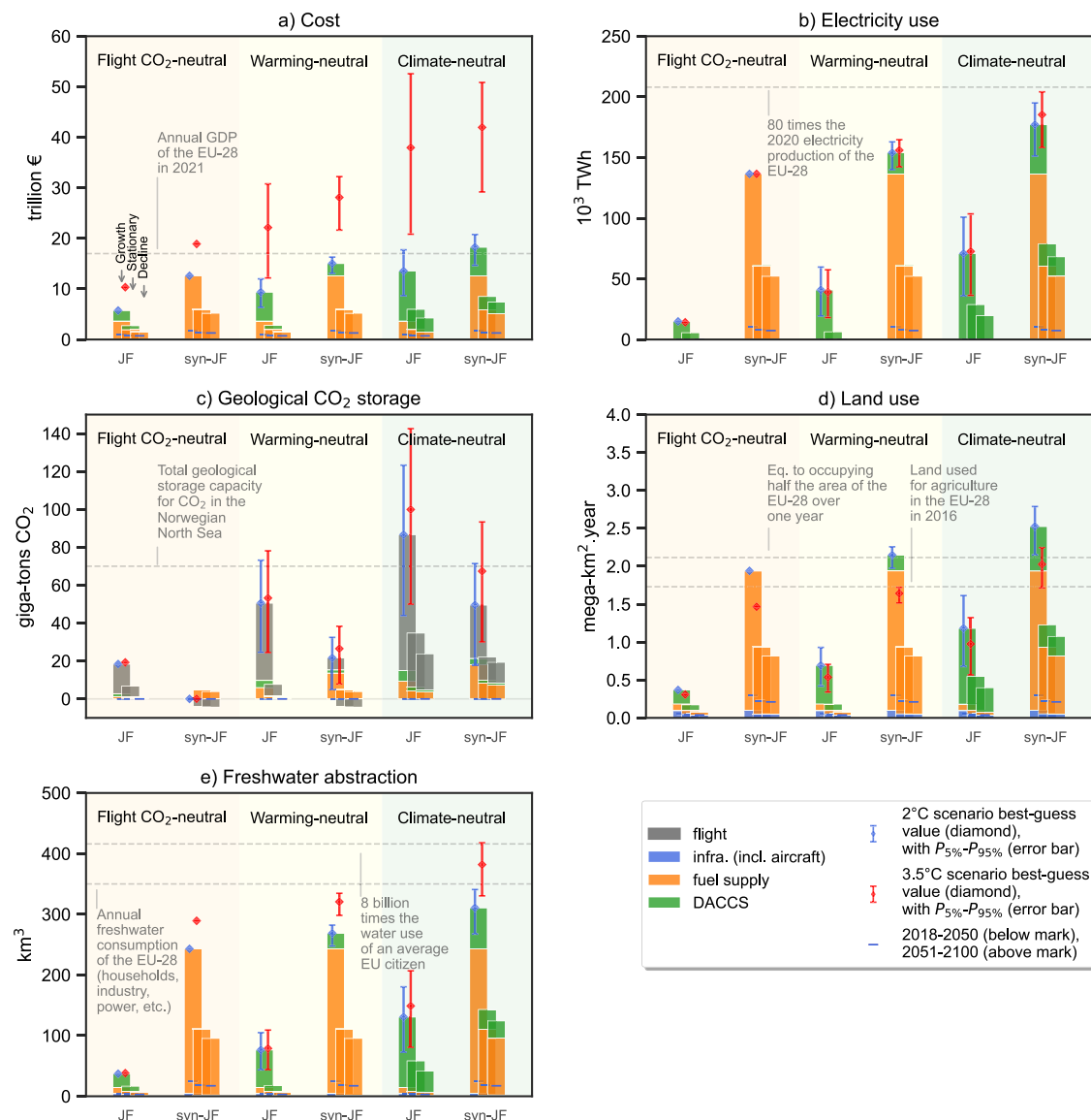
Fig. 4 | Cumulative resources required to achieve flight-CO 2 , warming, and climate-neutrality for a growing, stationary, and decreasing European passengers' fleet activity over the 2018–2100 period, using jet fuel and syn-jet fuel complemented by direct air capture and carbon storage (DACCS), considering a 2 °C (stacked bars and blue diamonds) and 3.5 °C climate scenario (red diamonds). a Cumulative cost, in trillion Euros, in today's terms. b Cumulative electricity use, in thousands of terawatt-hours. c Cumulative geological storage, in
