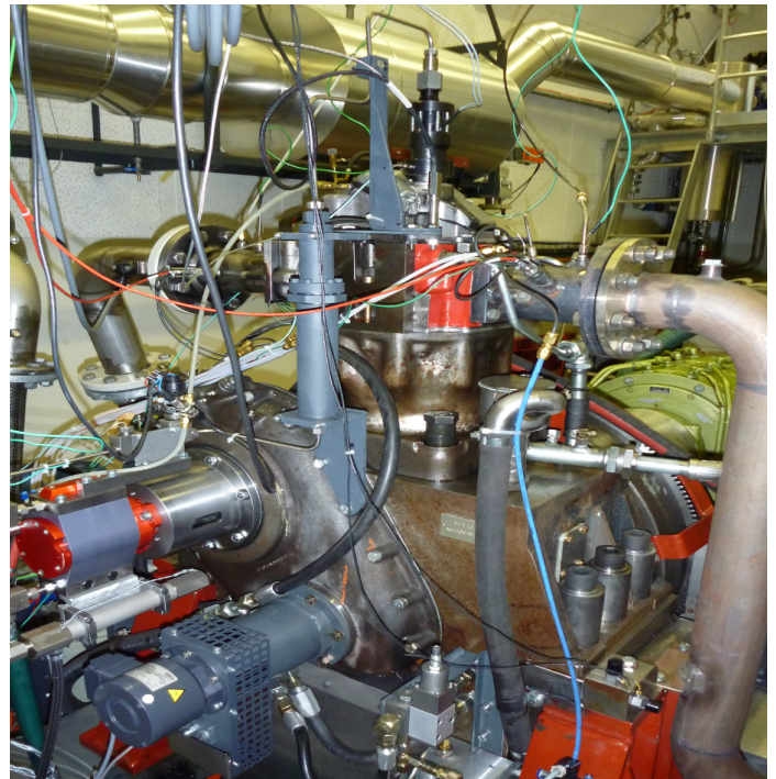
The basis of the ETHZ test bench is a single-cylinder diesel engine with a displacement volume of 4 liters, such as is used in ferries. Photo: ETHZ
