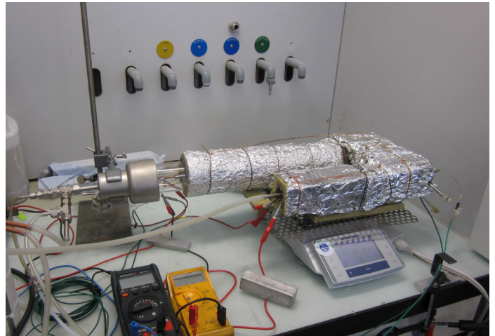
Empa researched the aspect of exhaust gas aftertreatment in the ReVerDi project. In the picture: Test set-up to investigate the regeneration of the diesel particulate filter. Photo: Empa
