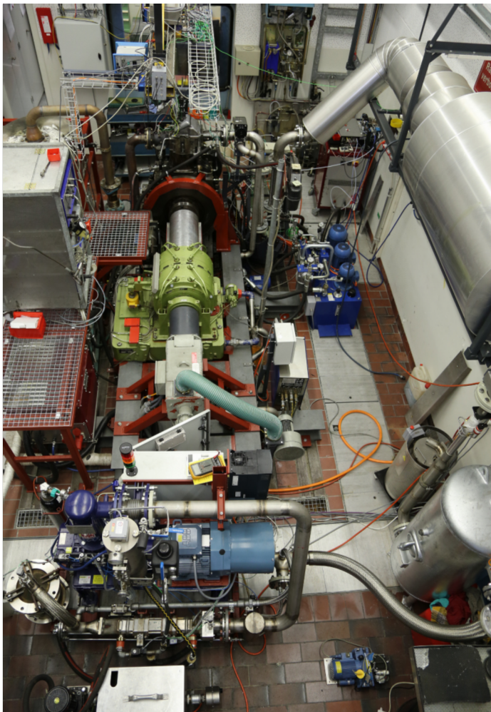
View of the (now dismantled) engine test bench in the machine hall at ETH Zurich. Here, researchers investigated the efficiency of bio-fuels for the ReVerDi research project. Photo: ETHZ
