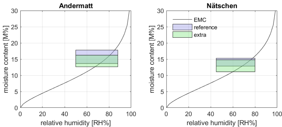
Figure 14: Comparison of moisture contents measured in the between the reference location and extra location of the cable car station of Andermatt and Nätschen.
