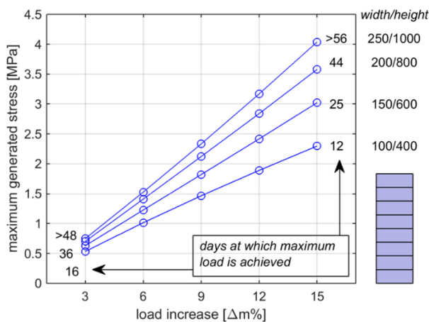
Figure 57: Maximum tensile stress due to selected step in a closer analysis where either pith location or ratio load magnitude in different cross-sections of width from 100 mm to 250 mm.
