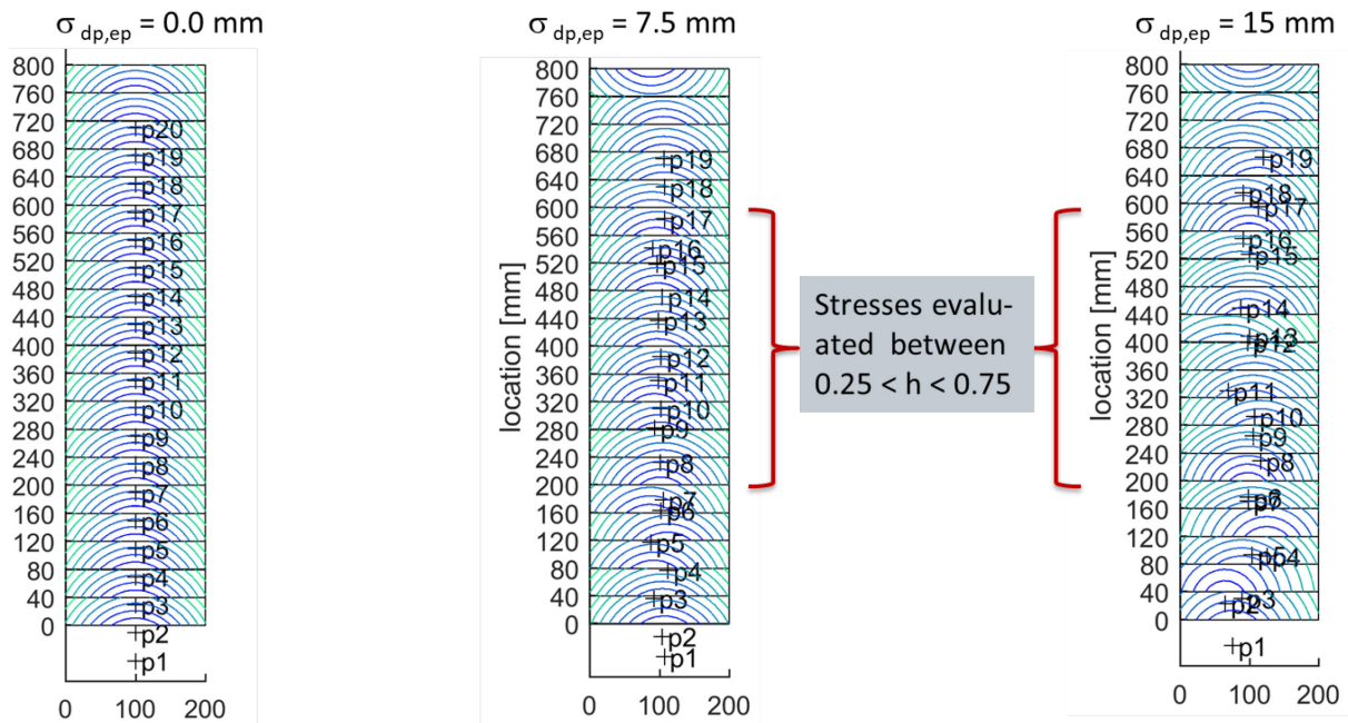
Figure 64: Glulam beam layup in the idealized condition (left) and the more realistic conditions (middle and right).
