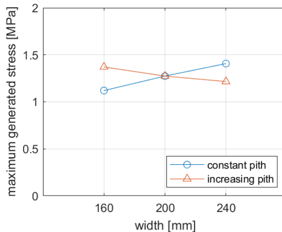
Figure 58: Dependency of tensile achieved stress levels of annual ring angle from edge to midplane was maintained constant
