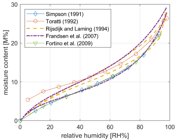
Figure 6: Comparison of mathematical equilibrium moisture content models for Spruce found in literature for a temperature of 20° C
