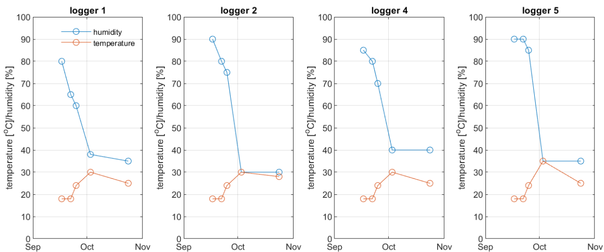
Figure 69: Summary of the measured humidity and temperature obtained from 'Quellgarten' on four out of six loggers (raw data not used)
