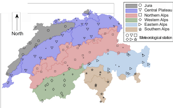
Figure 41: Biogeographical regions of Switzerland including the meteorological stations considered
