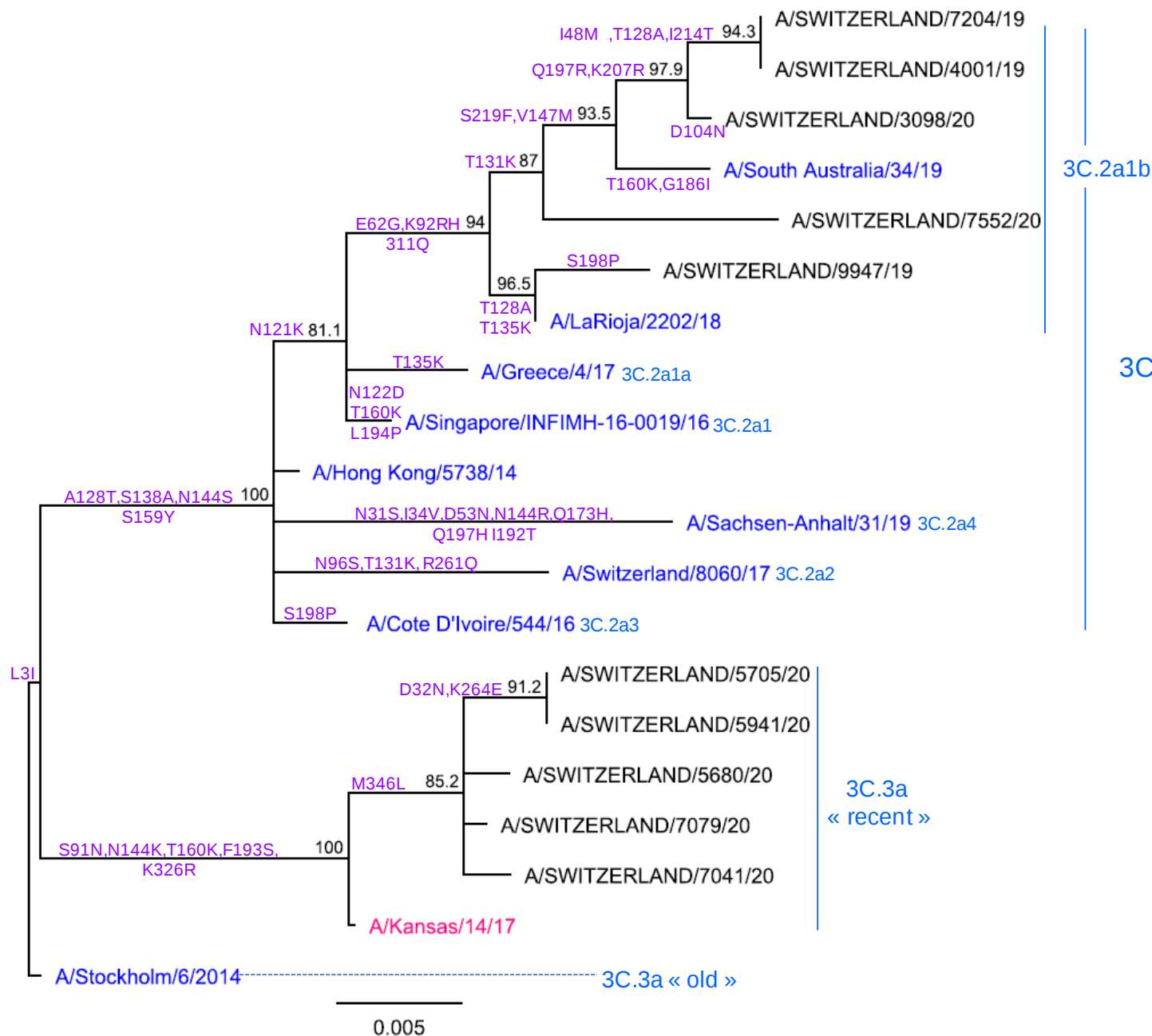
Figure 12. Phylogenetic analysis of the HA1 gene of A(H3N2) viruses. Black: influenza virus detected in the Sentinel network during the 2019/2020 season; strain names are A/Switzerland/isolate number/year (e.g. A/Switzerland/5214/19). Pink: 2019/20 vaccine strain. Blue: reference strains. Purple: typical substitutions described by the WIC and/or observed at the NRCI. 3C.2a, 3C.2a1 to 4 and 3C.3a are A(H3N2) genetic clades and subclades. Sequences were aligned using Geneious 9.1.7 MAFFT alignment (v7.017) with default settings. A consensus tree was built from 1000 original trees in ML (80% support threshold) constructed using Geneious 9.1.7 PHYML default settings.
