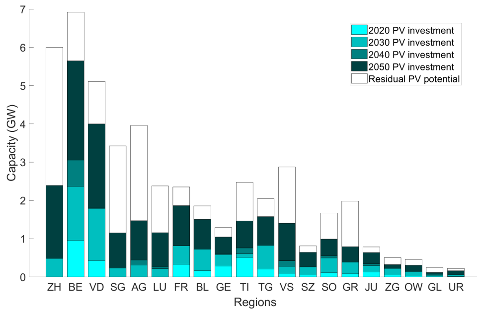
Figure 6: PV Investment per region
