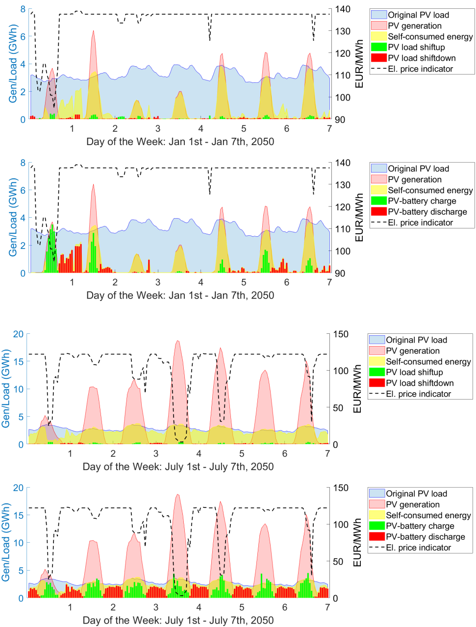
Figure 12: Hourly PV-controlled DR and PV-battery dispatch for one summer week and one winter week of year 2050
