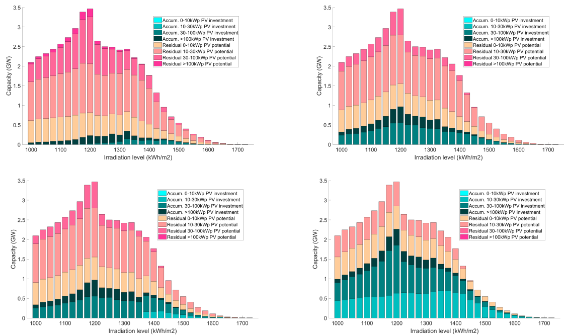
Figure 7: PV investments for the years 2020, 2030, 2040 and 2050.
