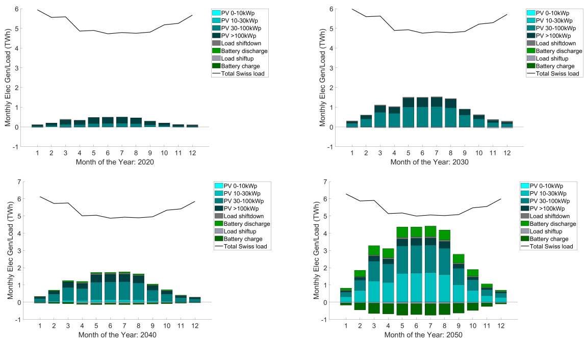
Figure 9: Monthly electricity generation for the years 2020, 2030, 2040 and 2050.
