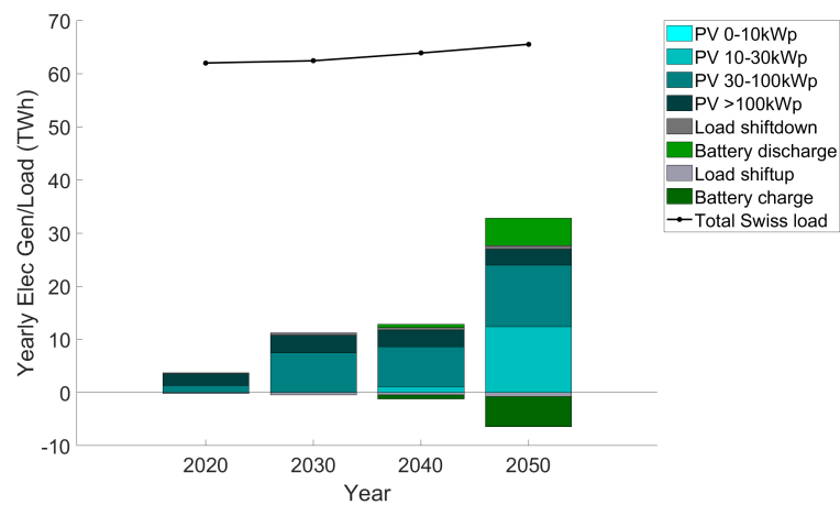
Figure 8: Electricity generation between 2020 and 2050.
