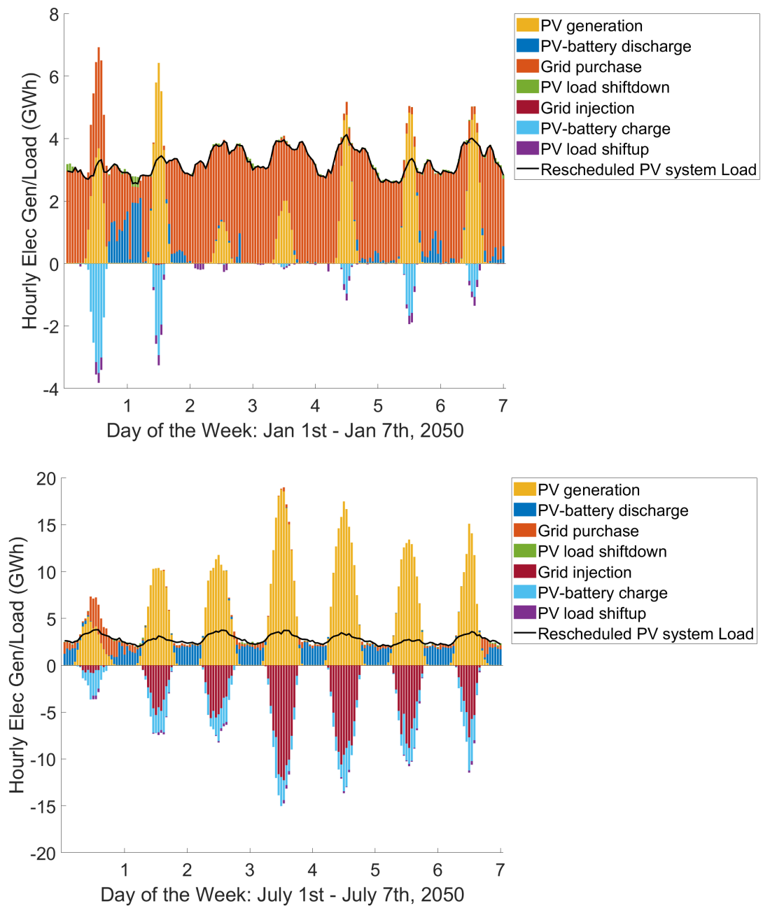
Figure 11: Hourly PV system dispatch for one summer week and one winter week of year 2050
