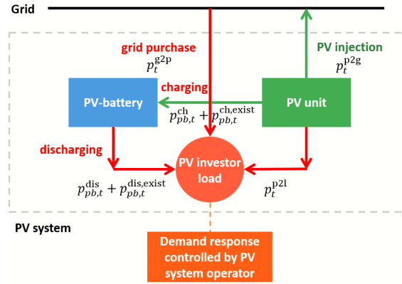
Figure 2: Structure of the PV system.
