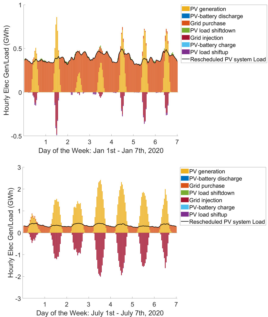
Figure 10: Hourly PV system dispatch for one summer week and one winter week of year 2020
