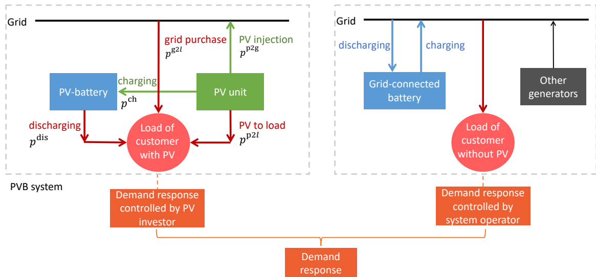
Figure 1: Structure of one sample aggregator.
