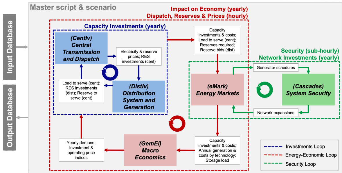
Figure 3: Illustration of the integration and interfacing of the various modules used in Nexus-e.
