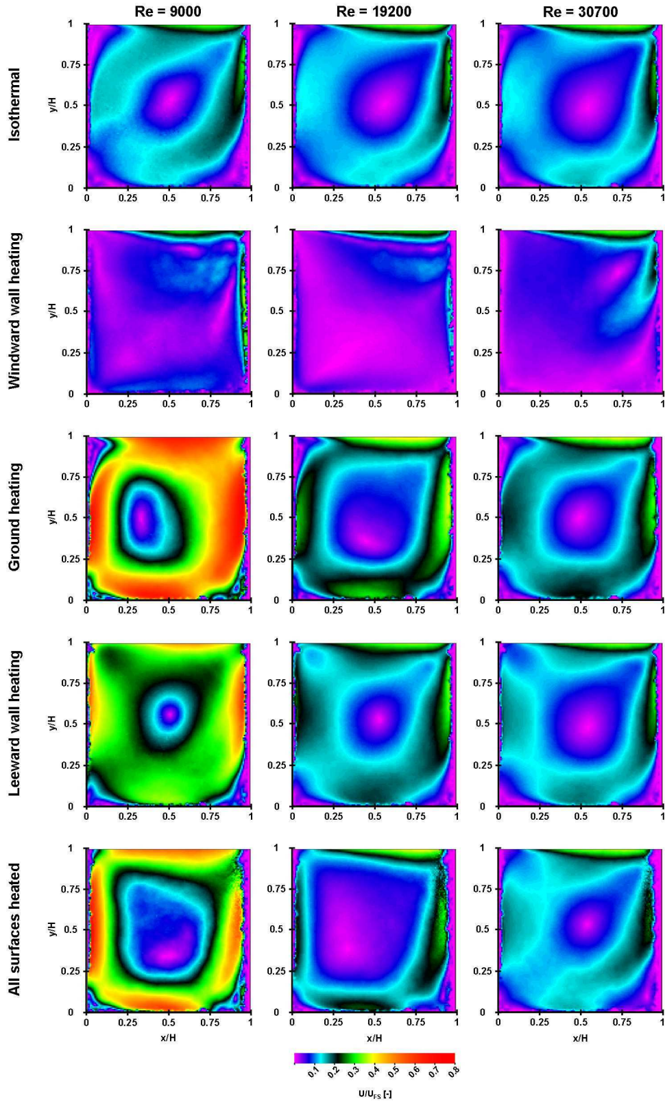
Figure 6.10: Contour plots of the normalised velocities inside the street canyon for various configurations of heated surfaces and for three different Reynolds numbers.
