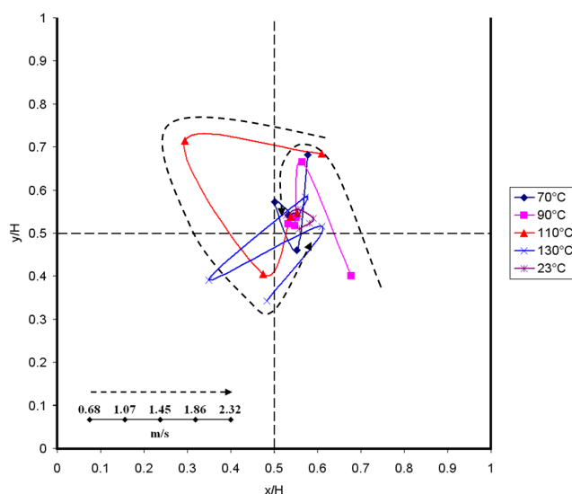
Figure 6.16: Trajectories of the centre of the main vortex as a function of the freestream velocities for five different surface temperatures.
