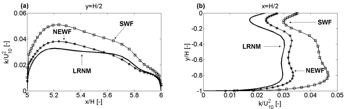
Figure 5.11: Turbulent kinetic energy profiles normalised by the square of the reference velocity as a function of the x or y position along the horizontal (a) and vertical centreline (b) (see Figure 5.4b). Results from simulations with SWF and NEWF are compared with result of a simulation with LRNM.
