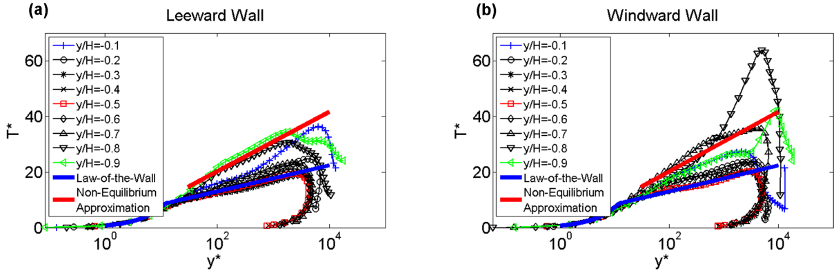
Figure 5.12: Dimensionless temperature profiles as a function of the y^* value on horizontal lines at different vertical positions y/H .
