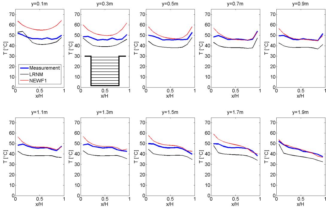
Figure 6.25: Temperature profiles on horizontal lines at different y -positions inside the street canyon. Wind tunnel measurements and CFD simulations for cases where all surfaces are heated using two different turbulence models and different near-wall modelling approaches (LRNM: Low-Reynolds number modelling with realizable k - \varepsilon ; NEWF1: non-equilibrium wall functions with standard k - \varepsilon ).
