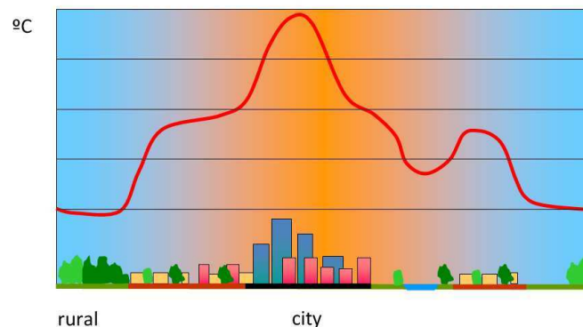
Figure 2.1: Sketch of an UHI profile (after [10]).
