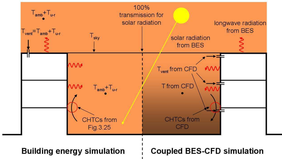
Figure 3.12: Schematic representation of the street canyon space.
