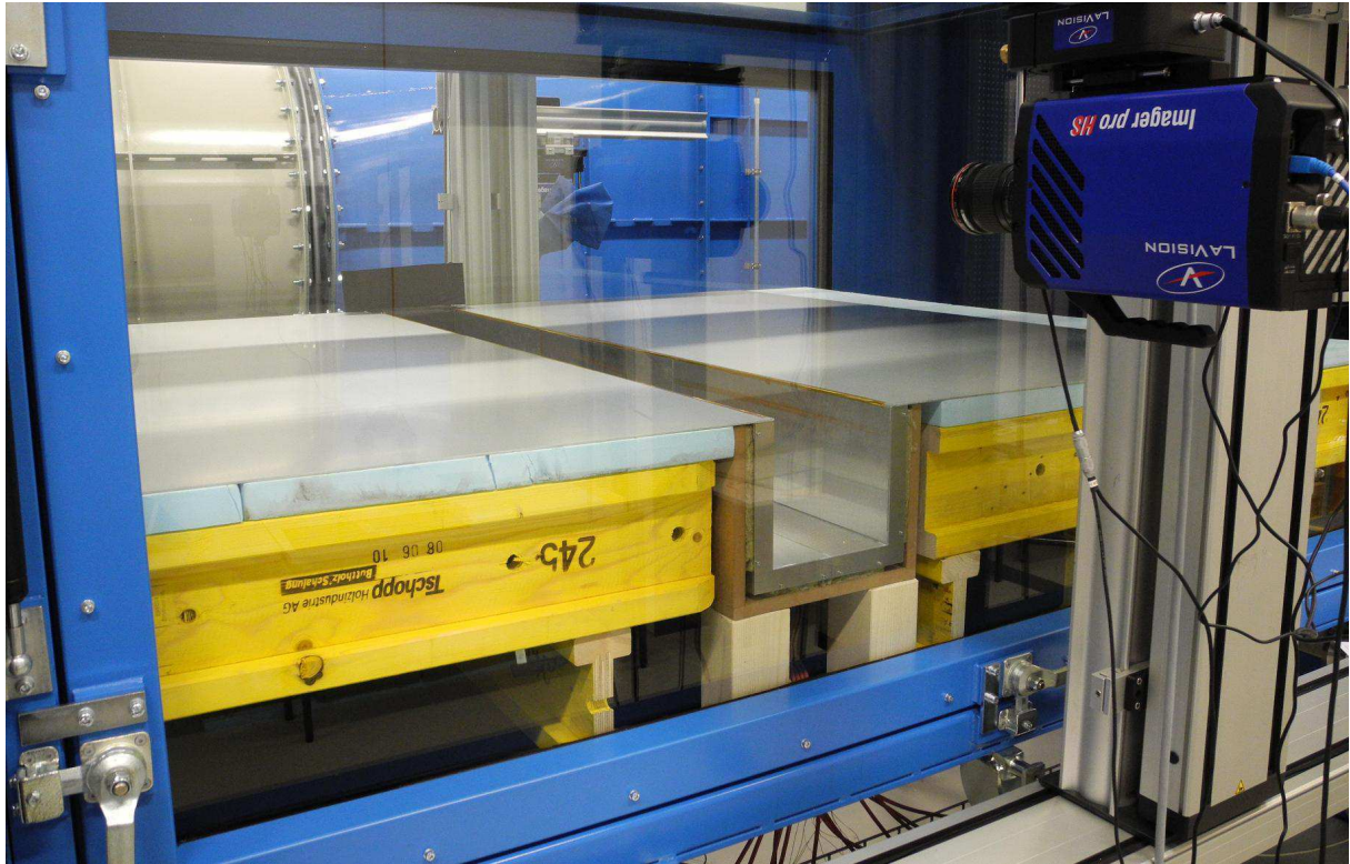
Figure 6.6: Picture of the wind tunnel model.
