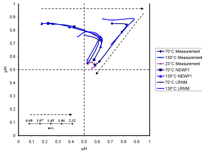
Figure 6.26: Trajectories of the centre of the main vortex as a function of the freestream velocity for different windward wall temperatures. Wind tunnel measurements and CFD simulations using two different turbulence models and different near-wall modelling approaches (LRNM: Low-Reynolds number modelling with realizable k-\varepsilon ; NEWF1: non-equilibrium wall functions with standard k-\varepsilon ).
