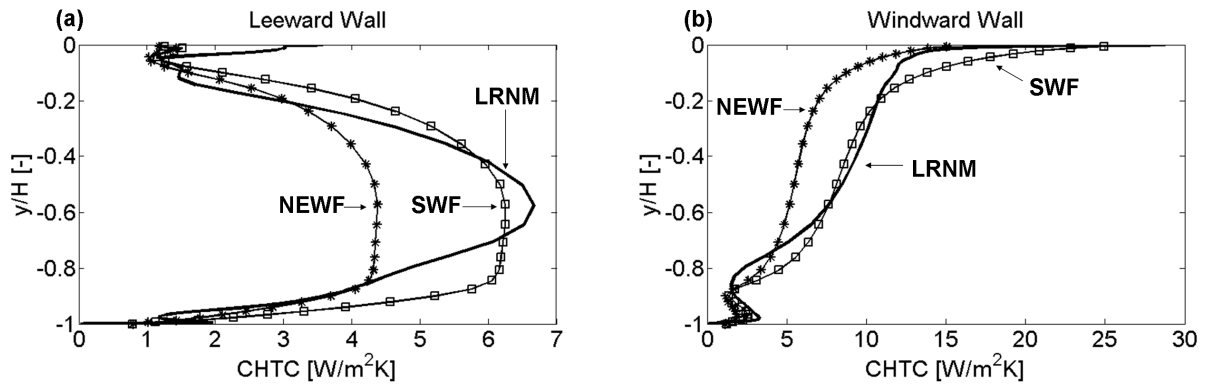
Figure 5.8: CHTC as a function of the vertical position y/H for a simulation with global Ri = 0.14 . Results from SWF and NEWF are compared with LRNM.
