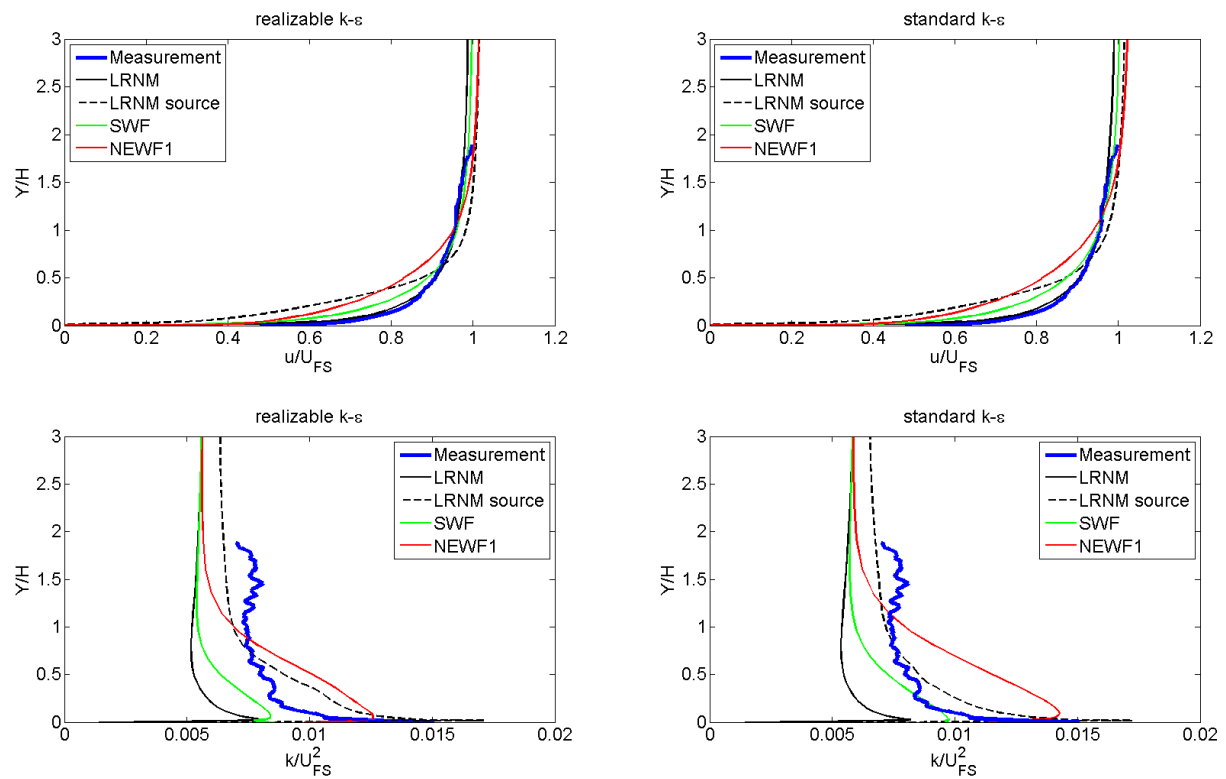
Figure 6.21: Normalised approach flow profiles of the velocity and TKE. Wind tunnel measurements and CFD simulations for the case with a freestream velocity of 1.45 \text{ m/s} using two different turbulence models and different near-wall modelling approaches (LRNM: Low-Reynolds number modelling; LRNM source: LRNM with source terms for k and predefined shear stresses at the surfaces in front and behind the street canyon; NEWF1: non-equilibrium wall functions; SWF: standard wall functions).
