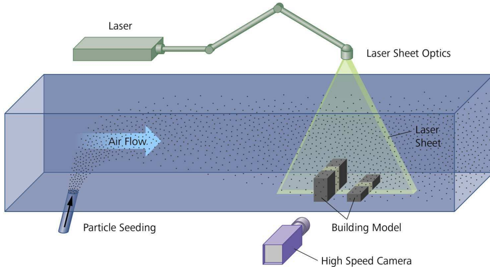
Figure 6.1: Sketch of the measurement equipment.
