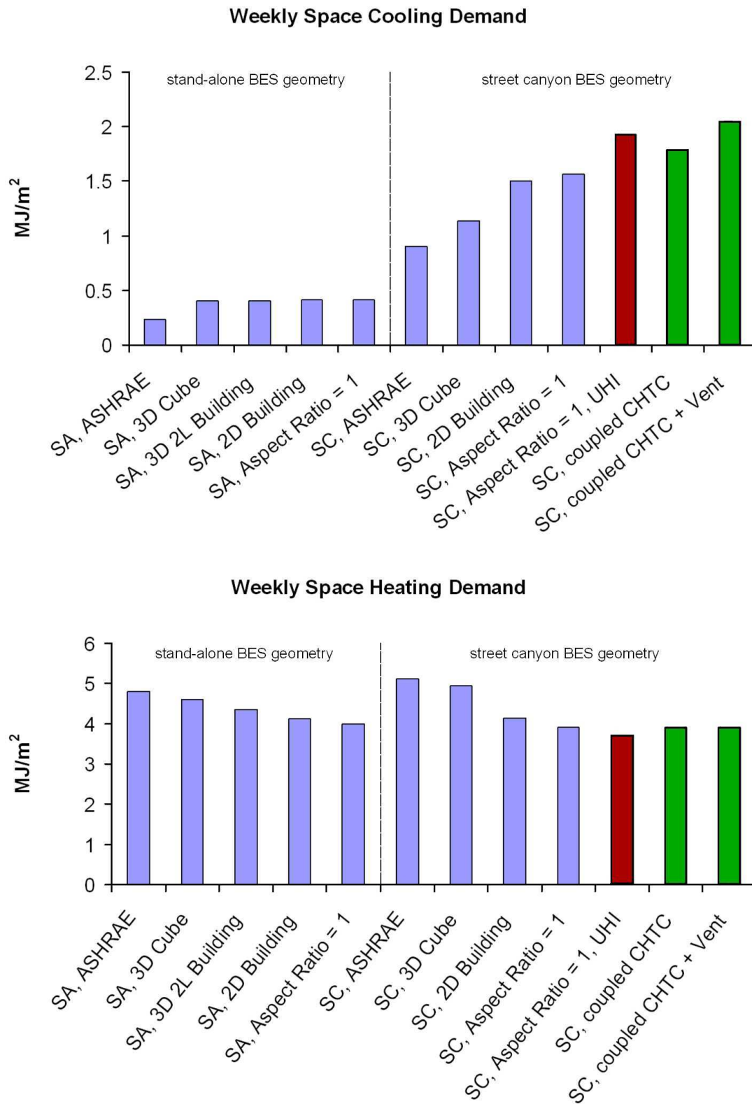
Figure 4.14: Weekly energy demand for space cooling and heating with different modelling approaches (Table 4.4).
