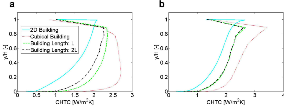
Figure 3.5: CHTC profiles on the vertical centreline of the leeward (a) and windward (b) walls of the 4 studied stand-alone buildings (simulations with 0.5\text{ m/s} and heated surface temperatures of 30^\circ\text{C} ).
