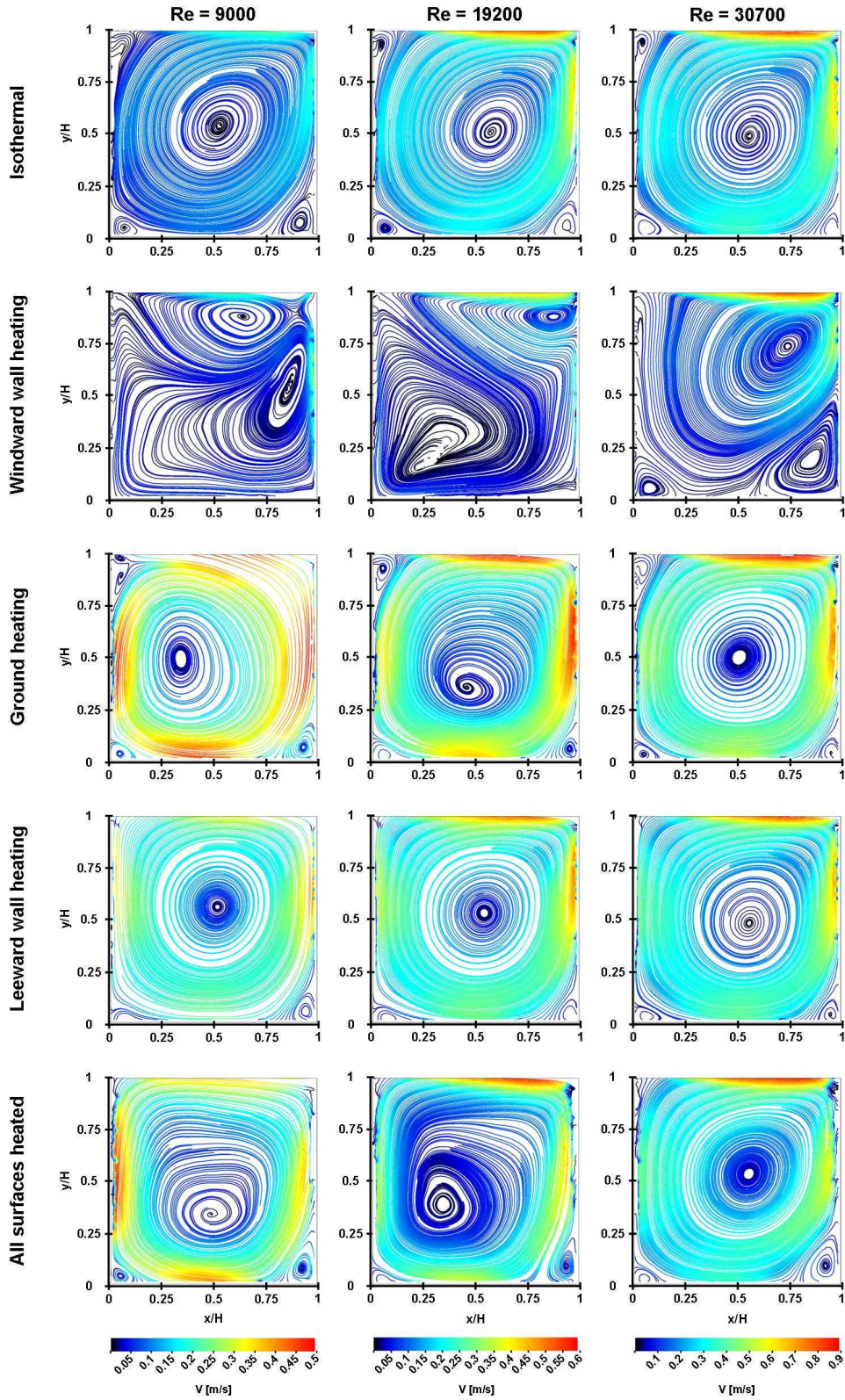
Figure 6.8: Streamlines for various configurations of heated surfaces and for three different Reynolds numbers.
