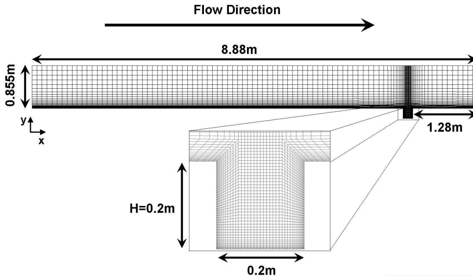
Figure 6.20: Computational domain.
