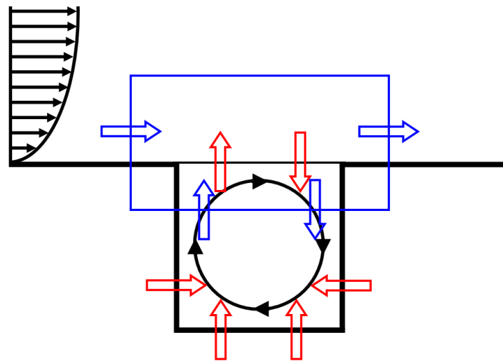
Figure 6.29: Sketch of the heat fluxes in a street canyon.
