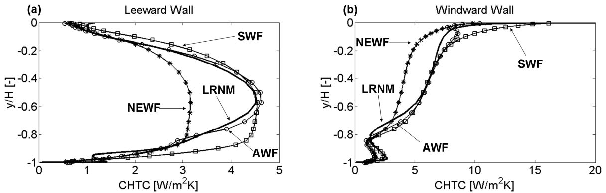
Figure 5.14: CHTC as a function of the vertical positions y/H for a simulation with global Ri = 0.38 . Results from SWF, NEWF and AWF are compared with LRNM.
