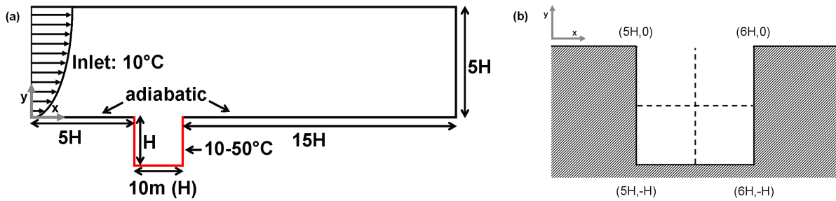
Figure 5.4: Computational domain (a); Horizontal and vertical centrelines in the street canyon (b). In all Figures y^* ranges from the surface to the intersection of the horizontal and the vertical centrelines.
