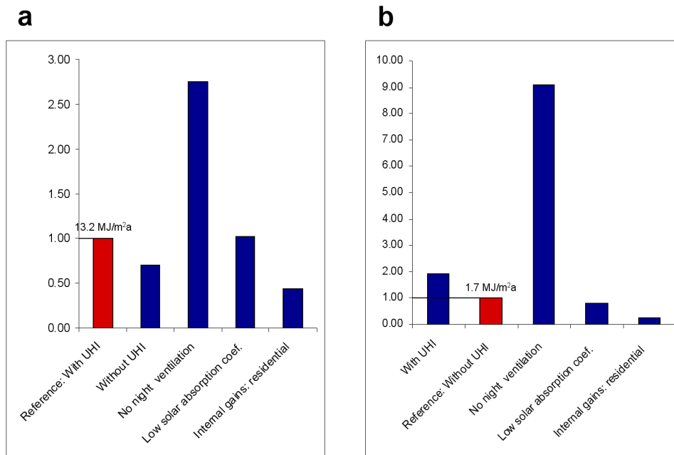
Figure 4.13: Annual space cooling demand for the New Building type and an orientation of 0^\circ . (a) Building surrounded by street canyons with an aspect ratio of 1, normalized by the case with UHI intensity; (b) stand-alone building, normalized by the case without UHI intensity.
