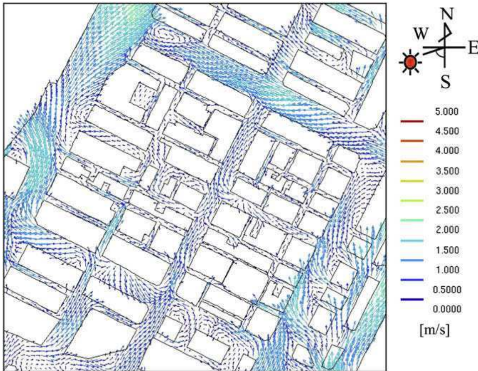
Figure 2.9: Horizontal distribution of the wind velocity in Kyobashi. (taken from [72]).
