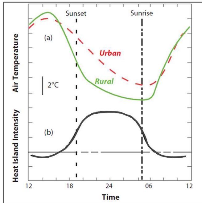
Figure 2.2: Sketch of diurnal temperatures in urban and rural areas (after [11]).
