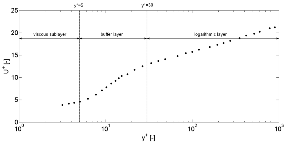
Figure 5.1: Dimensionless velocity ( U^+ ) boundary layer profile as a function of y^+ (experimental data of Hussain and Reynolds 1975 [176]).
