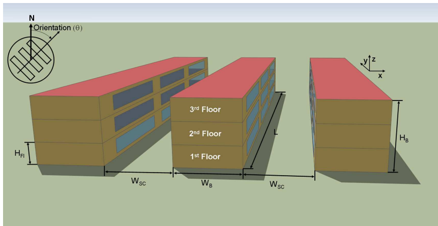
Figure 4.1: Studied building surrounded by street canyons with aspect ratios of 1 ( H/W ).
