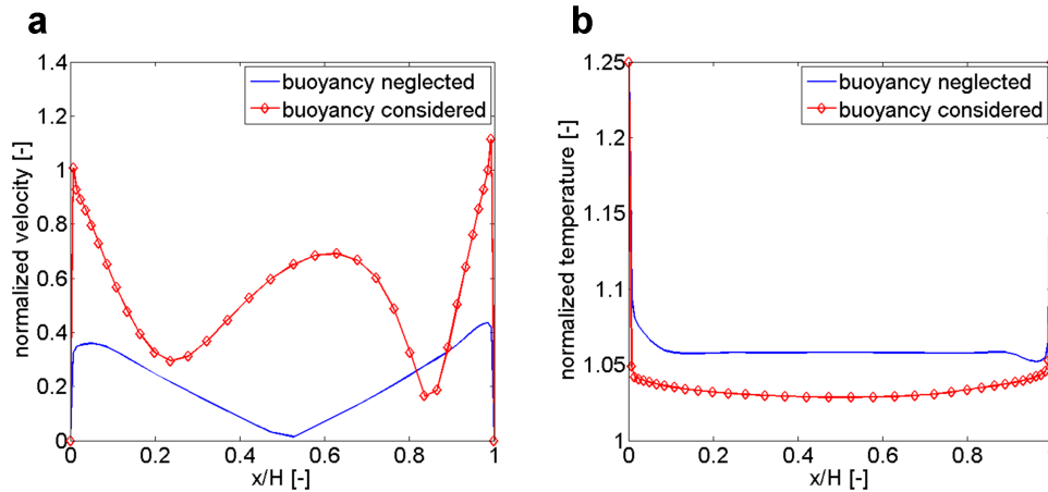
Figure 3.3: Velocity magnitude normalized by U_{10} (a) and temperature normalized by the inlet temperature (b) on the horizontal centreline in a street canyon with an aspect ratio of 2, U_{10} = 0.25 \text{ m/s} , inlet temperature 20^\circ\text{C} and wall and ground surface temperatures of 25^\circ\text{C} .
