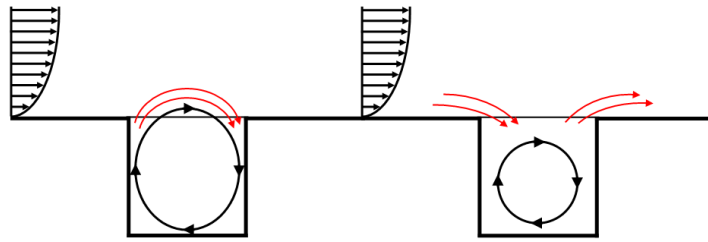
Figure 6.30: Sketch of the flow in a street canyons with a main vortex with a diameter larger than the street canyon height (left) and smaller than the street canyon height (right).
