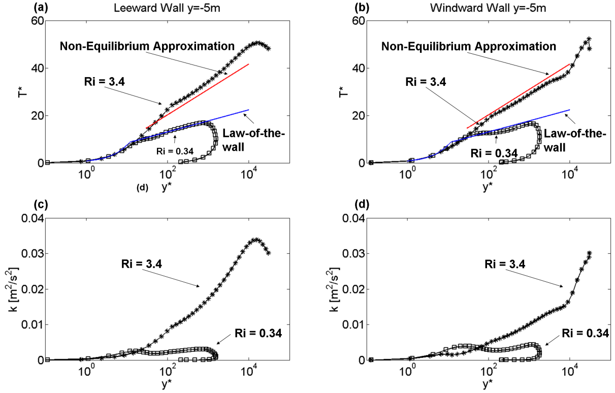
Figure 5.5: Dimensionless temperature profiles and turbulent kinetic energy profiles as a function of the y^* value on the horizontal centreline (see Figure 5.4b) of a street canyon for two simulations with different global Ri numbers (0.34 and 3.4).
