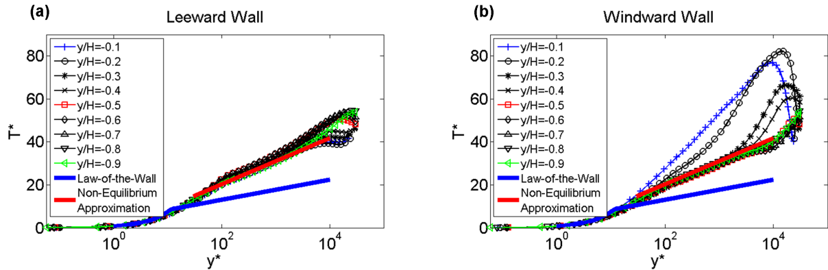
Figure 5.10: Dimensionless temperature profiles as a function of the y^* value on horizontal lines at different vertical positions y/H .
