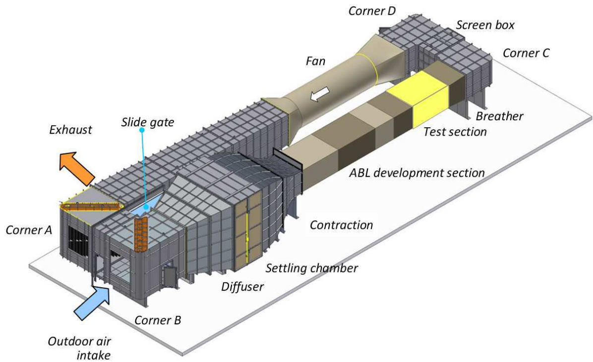
Figure 6.3: Sketch of the ETH/Empa atmospheric boundary layer wind tunnel.
