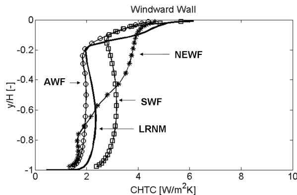
Figure 5.16: CHTC as a function of the vertical positions y for a simulation with a 3D street canyon with global Ri = 3.4 . Results from simulations with SWF, NEWF and AWF are compared with result of a simulation with LRNM.
