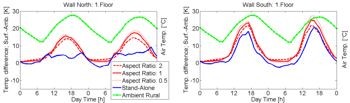
Figure 4.11: Differences between the wall surface temperature and the ambient air temperature for the north and south façades of the first floor for a stand-alone building and buildings surrounded by street canyons with different aspect ratios (0.5, 1 and 2).
