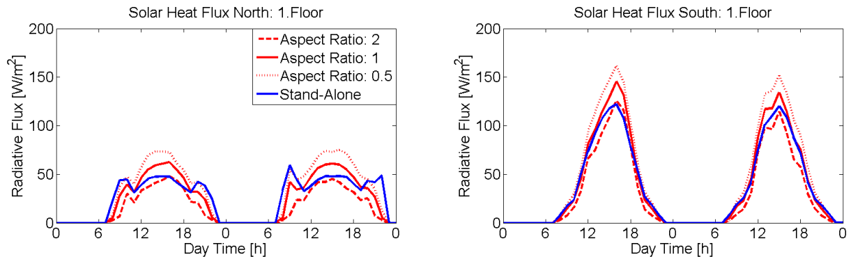
Figure 4.9: Absorbed solar radiation on the south and north façades of the first floor for a stand-alone building and buildings surrounded by street canyons with different aspect ratios (0.5, 1 and 2).
