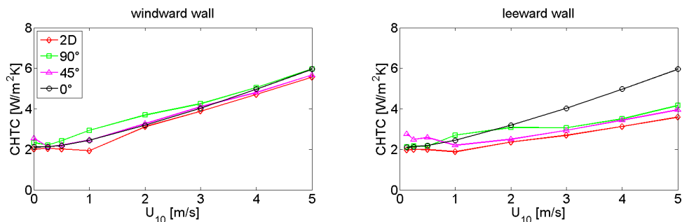
Figure 3.7: CHTC versus wind speed with a temperature of 30 °C for the heated surfaces for a 2D and a 3D street canyon (aspect ratio: 1) with different wind direction (90°: wind normal to the street axis, 0°: wind parallel to the street axis).
