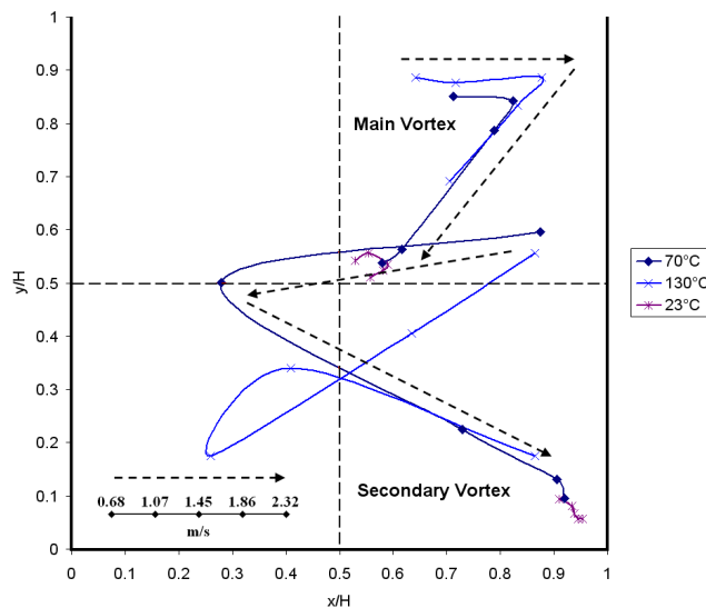
Figure 6.13: Trajectories of the centre of the main and secondary vortex as a function of the freestream velocity for three different windward wall temperatures.
