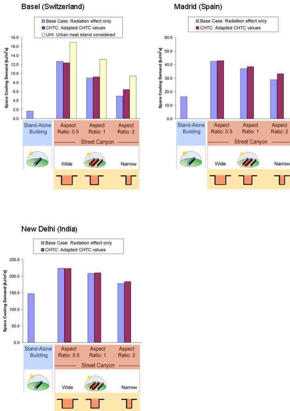
Figure 4.18: Annual space cooling demand for different climates and different modelling cases.
