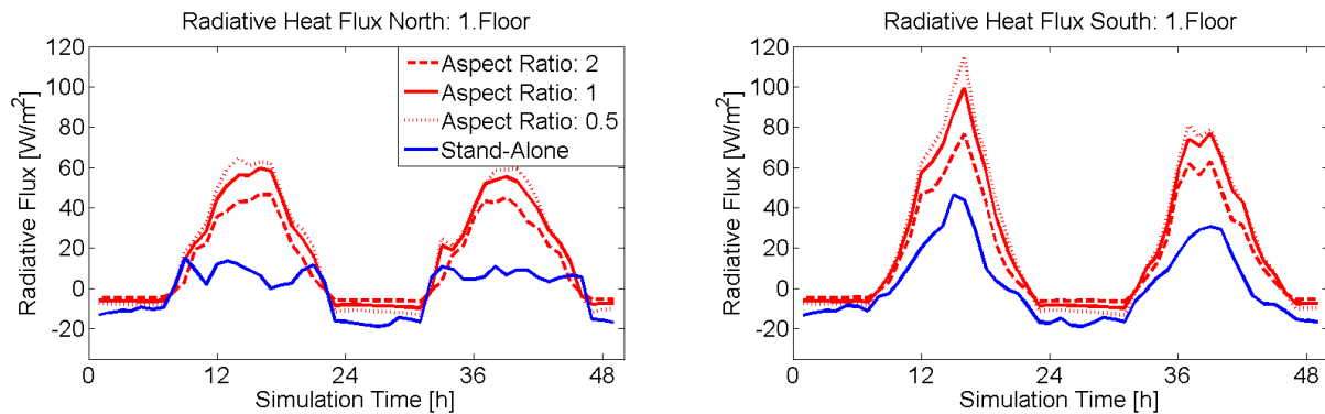
Figure 4.10: Absorbed radiation (longwave plus solar) on the south and north façades of the first floor for a stand-alone building and buildings surrounded by street canyons with different aspect ratios (0.5, 1 and 2).
