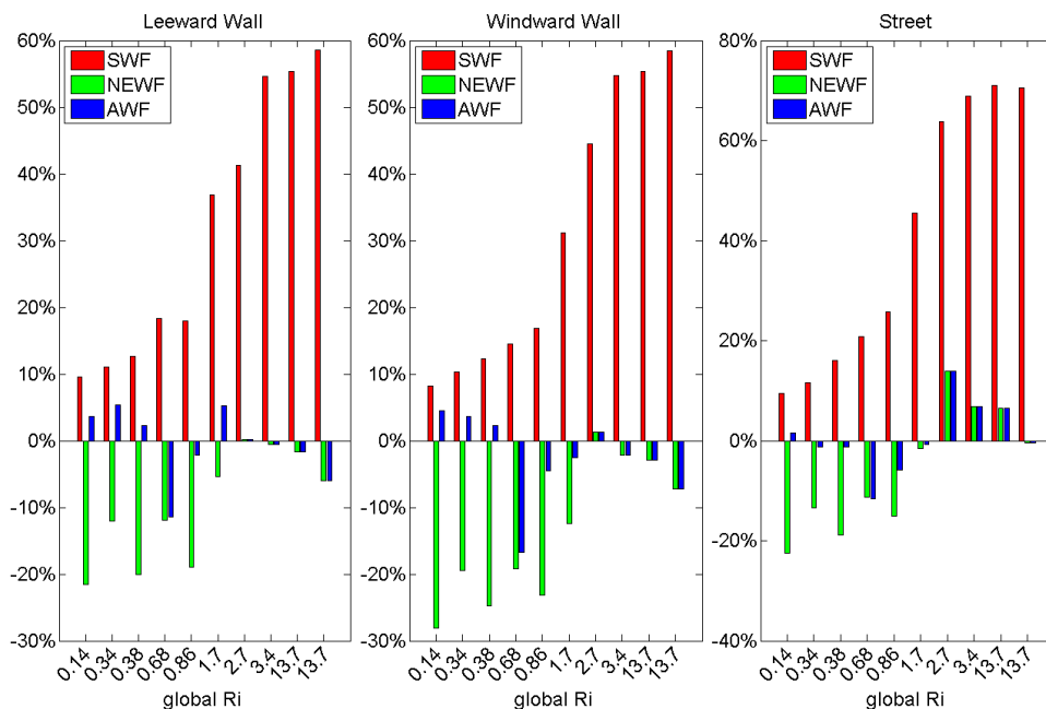
Figure 5.15: Relative differences of the total heat flux at the walls for the SWF, NEWF and the AWF compared to the LRNM for different global Ri .
