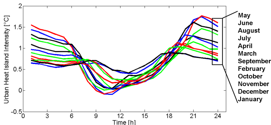
Figure 3.8: Average diurnal UHI intensity schedules for each month of a year.
