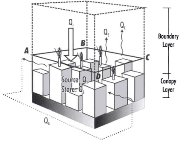
Figure 2.5: Schematic presentation of the energy fluxes in the urban environment (taken from [10], after [3]).
