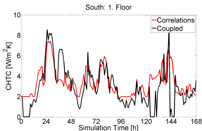
Figure 4.15: Comparison between CHTCs from correlations and coupled BES-CFD simulations.
