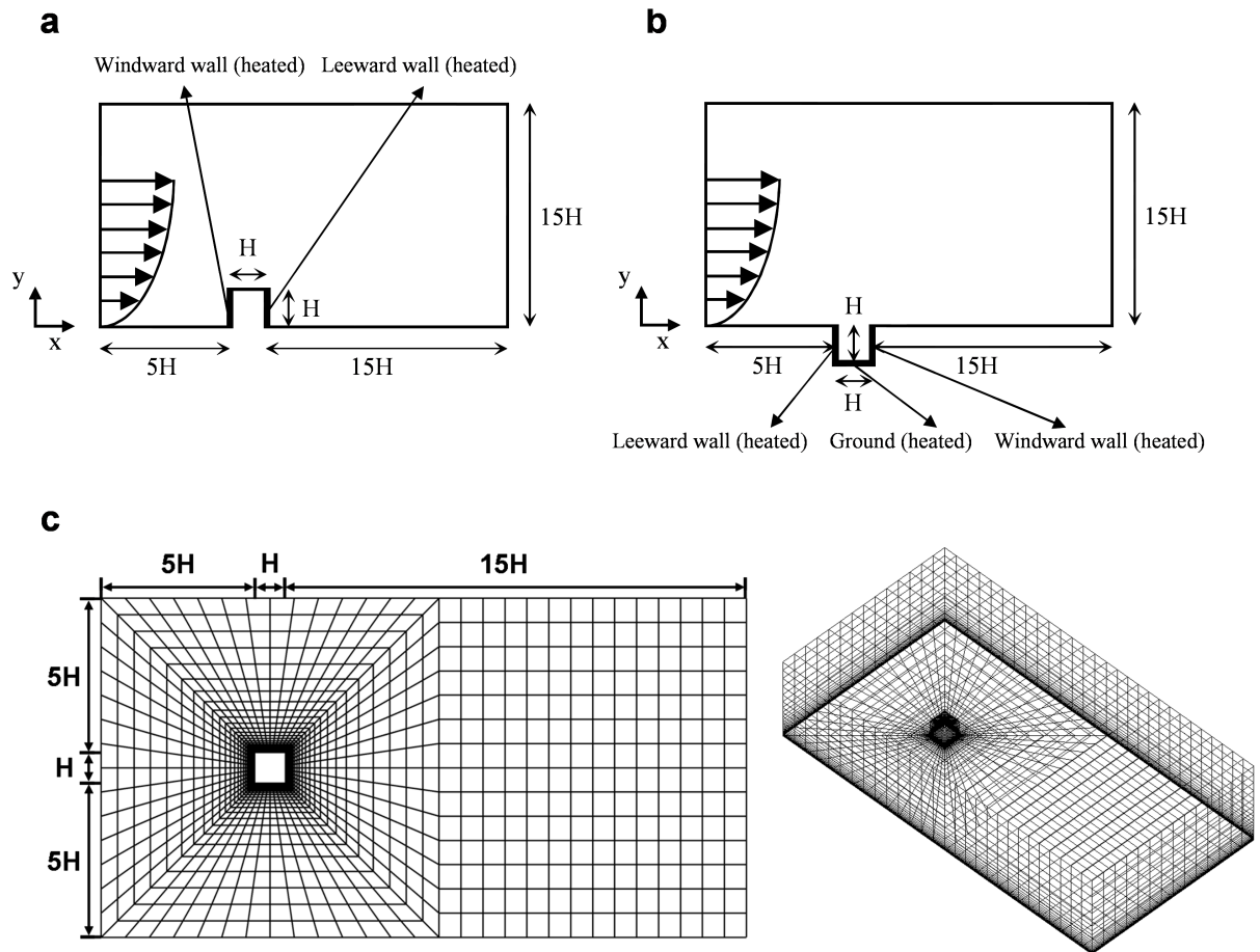
Figure 3.1: Computational domain for a 2D stand-alone building (a), a 2D street canyon (b) and a 3D cubical building (topview and 3D view) (c).
