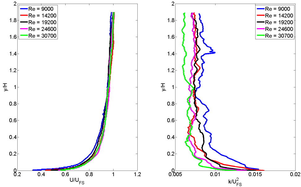
Figure 6.7: Time averaged boundary layer velocities normalised by the freestream velocity (left) and the TKE ( k ) normalised by the square of the freestream velocity (right).
