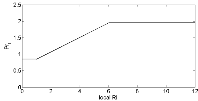
Figure 5.13: Turbulent wall Prandtl number as a function of the local Richardson number.
