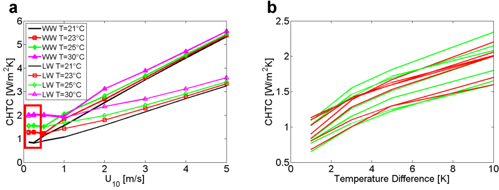
Figure 3.6: (a) CHTC versus wind speed for windward (WW) and leeward (LW) walls with different wall and ground surface temperatures for a street canyon with an aspect ratio of 1. (b) CHTC for low wind speeds (red box in Figure 3.6a) versus temperature difference between air and surfaces temperatures for all 7 geometries: windward (red) and leeward (green) walls.
