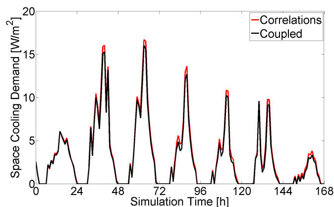
Figure 4.16: Space cooling demands for coupled and uncoupled BES simulations for a time period of a week.
