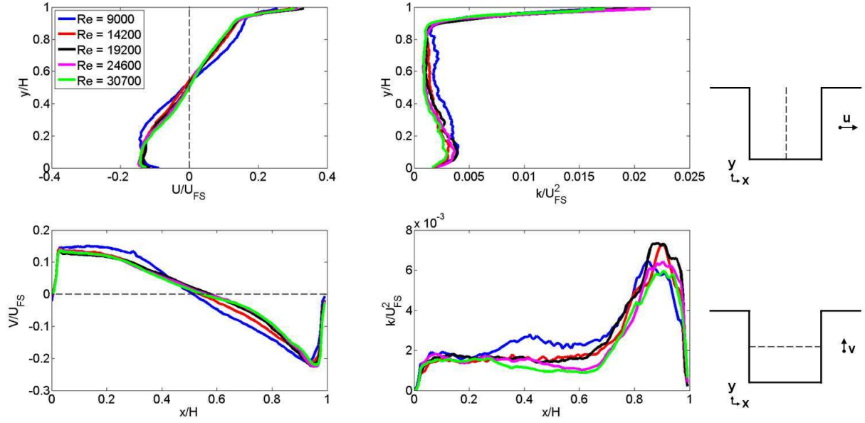
Figure 6.9: Normalised velocity (left) and TKE (right) profiles on the horizontal and vertical centrelines of the street canyon.
