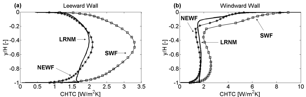
Figure 5.9: CHTC as a function of the vertical position y/H for a simulation with global Ri = 3.4 . Results from SWF and NEWF are compared with LRNM.
