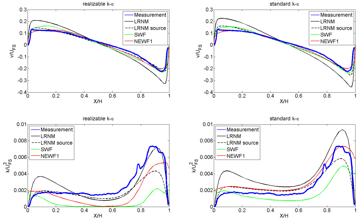
Figure 6.22: Normalised centreline profiles of the vertical velocity and TKE. Wind tunnel measurements and CFD simulations for the case with a freestream velocity of 1.45 \text{ m/s} using two different turbulence models and different near-wall modelling approaches (LRNM: Low-Reynolds number modelling; LRNM source: LRNM with source terms for k and predefined shear stresses at the surfaces in front and behind the street canyon; NEWF1: non-equilibrium wall functions; SWF: standard wall functions).
