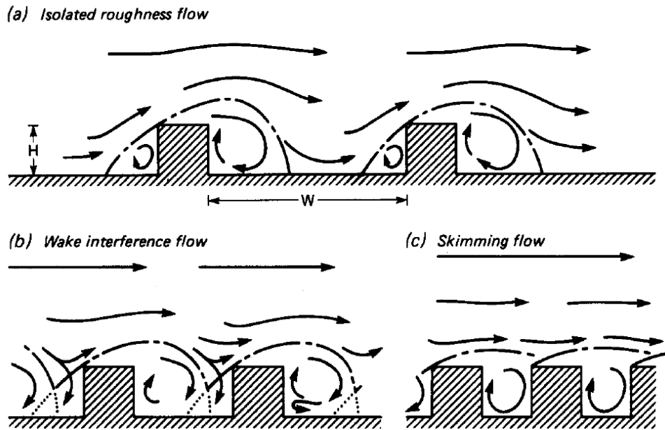
Figure 2.11: The flow regimes associated with air flow over building arrays of increasing H/W (taken from [73]).
