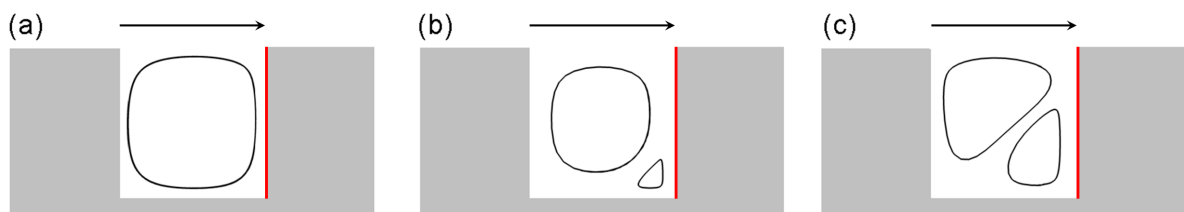
Figure 5.3: Streamlines of forced convective (a), intermediate convective (b) and mixed convective (c) cases (red walls are heated).
