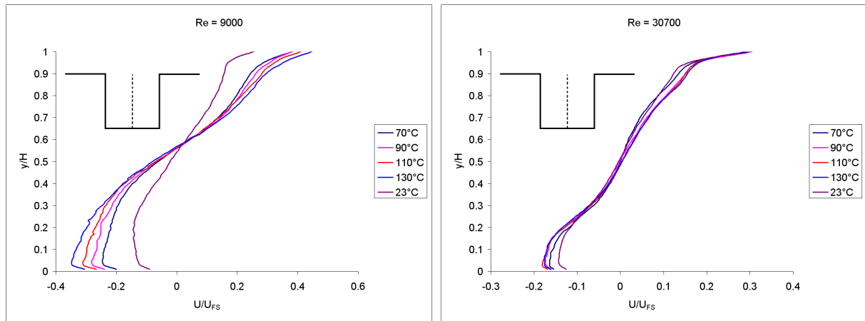
Figure 6.15: Normalised velocity profiles on the vertical centreline of the street canyon for different Reynolds numbers and different leeward wall temperatures.
