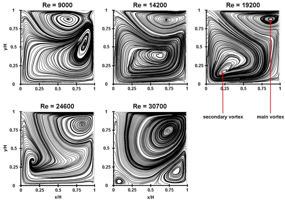
Figure 6.12: Streamlines for cases with windward wall heating and five different Reynolds numbers.
