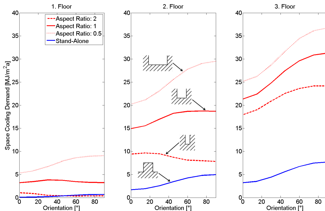
Figure 4.8: Annual space cooling demands for the three floors as a function of the street canyon orientation, for the three street canyon aspect ratios and the stand-alone building (New Building type).
