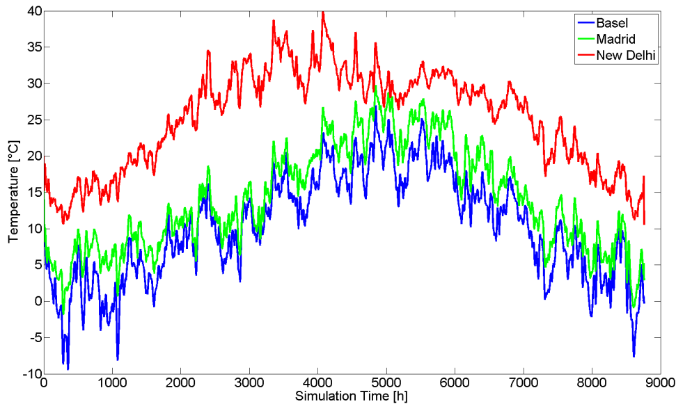
Figure 4.17: Air temperatures for Basel, Madrid and New Delhi (typical meteorological year TMY) for one year.
