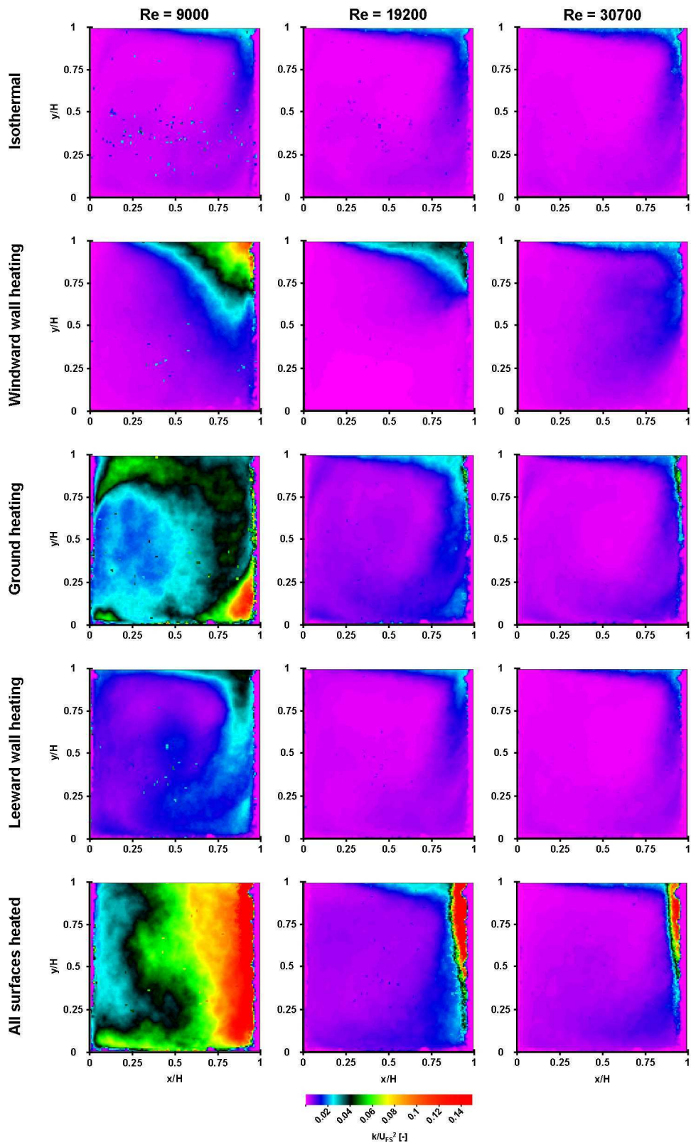
Figure 6.11: Contour plots of the normalised TKEs inside the street canyon for various configurations of heated surfaces and for three different Reynolds numbers.
