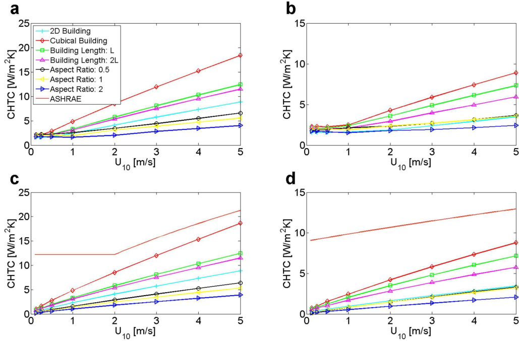
Figure 3.4: CHTC versus wind speed with a temperature of 30\text{ }^{\circ}\text{C} for the heated surfaces: (a) windward wall with buoyancy; (b) leeward wall with buoyancy; (c) windward wall without buoyancy; (d) leeward wall without buoyancy.
