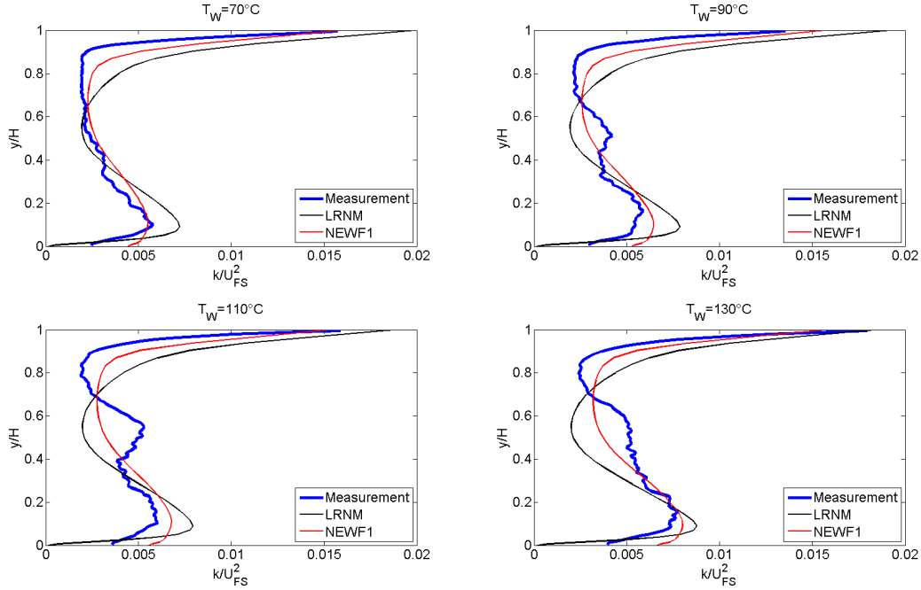
Figure 6.28: Normalised centreline profiles of the TKE. Wind tunnel measurements and CFD simulations using two different turbulence models and different near-wall modelling approaches (LRNM: Low-Reynolds number modelling with realizable k-\varepsilon ; NEWF1: non-equilibrium wall functions with standard k-\varepsilon ).
