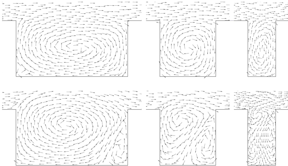
Figure 3.2: Flow fields neglecting buoyancy (top) and considering buoyancy (bottom) for aspect ratios of 0.5, 1 and 2 (left to right).
