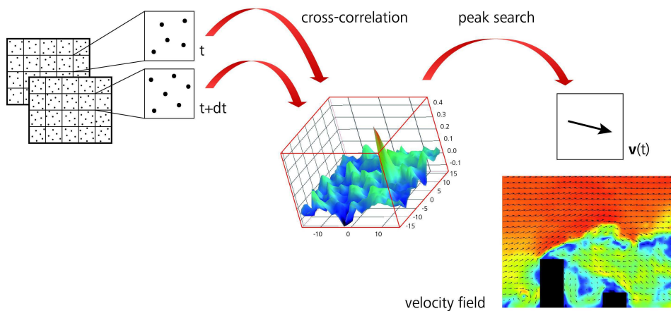
Figure 6.2: PIV measurement principle (LaVision GmbH).
