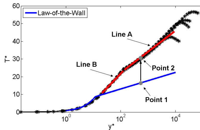
Figure 5.2: Dimensionless temperature profiles of LRNM simulations of non-equilibrium flows in street canyons (from CFD simulations of this study; compare with Figure 5.7) as a function of the y^* value; Blue: temperature law-of-the-wall; Red: logarithmic approximations.
