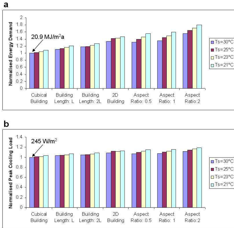
Figure 4.4: Total annual space cooling demands (a) and annual peak cooling loads (b) normalised by the results for the cubical building with T_s = 30\text{ }^\circ\text{C} for a street canyon with an aspect ratio of 1 using CHTC correlations developed for different geometries and temperature differences between building façades ( T_s ) and ambient air (here 20\text{ }^\circ\text{C} ).
