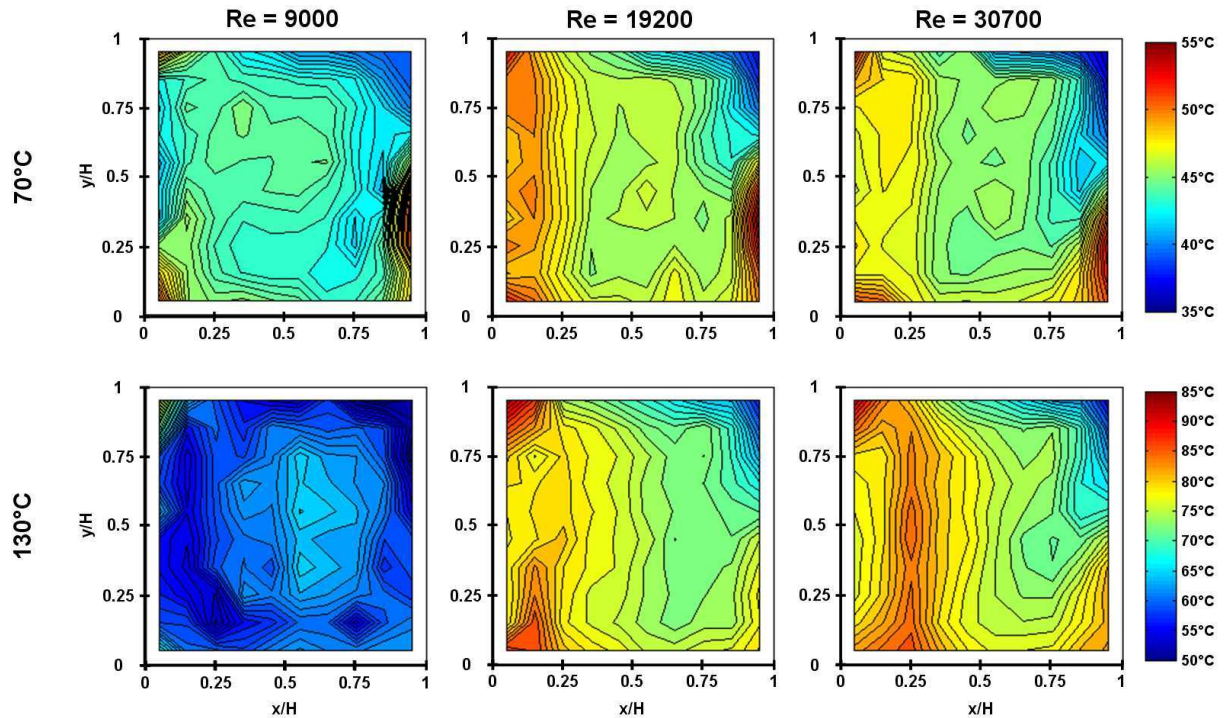
Figure 6.18: Contour plots of the air temperatures inside the street canyon for surface temperatures of 70^{\circ}\text{C} and 130^{\circ}\text{C} (all surfaces heated) and three different Reynolds numbers.
