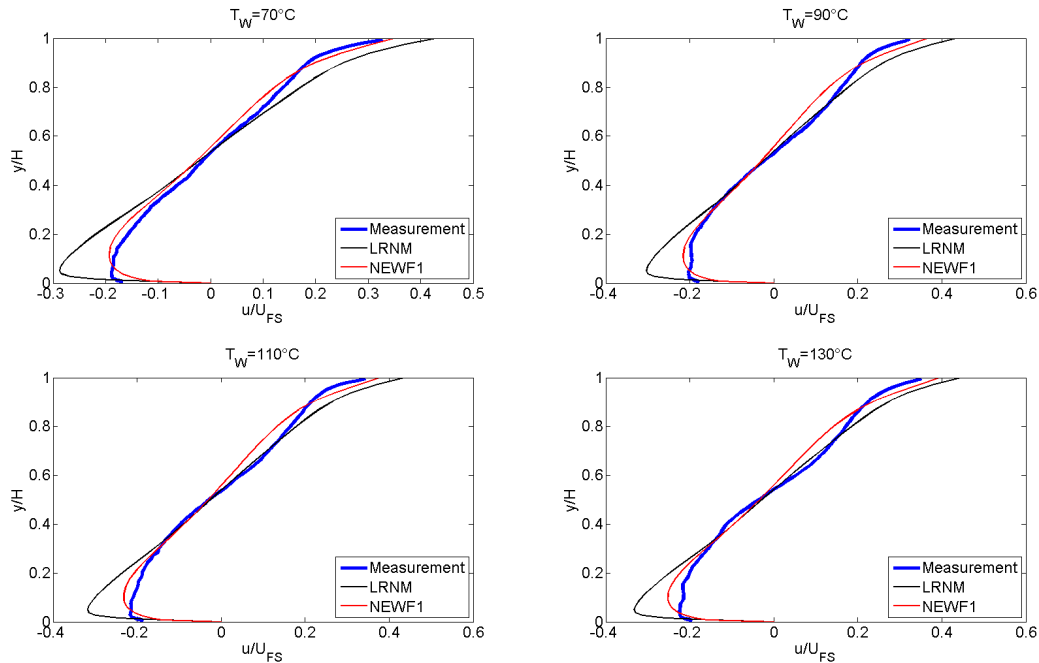
Figure 6.27: Normalised centreline profiles of the horizontal velocity. Wind tunnel measurements and CFD simulations using two different turbulence models and different near-wall modelling approaches (LRNM: Low-Reynolds number modelling with realizable k-\varepsilon ; NEWF1: non-equilibrium wall functions with standard k-\varepsilon ).
