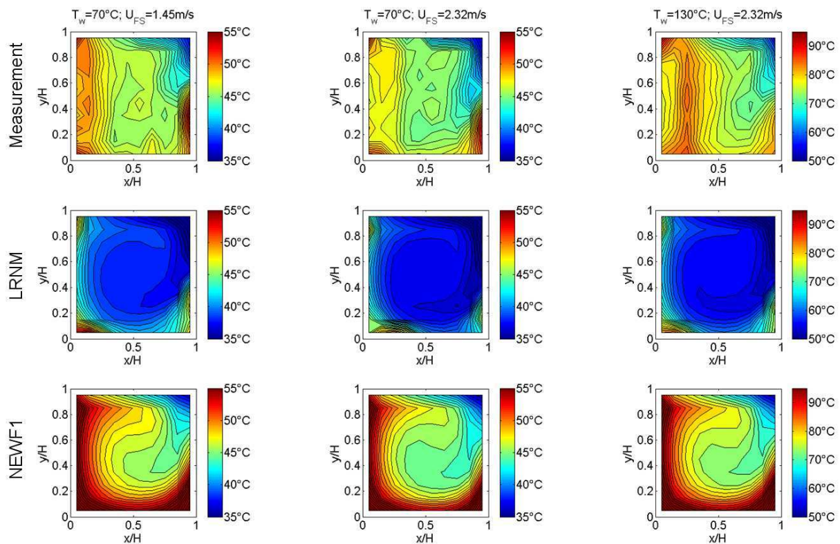
Figure 6.24: Contour plots of the air temperatures inside the street canyon. Wind tunnel measurements and CFD simulations for cases where all surfaces are heated using two different turbulence models and different near-wall modelling approaches (LRNM: Low-Reynolds number modelling with realizable k - \varepsilon ; NEWF1: non-equilibrium wall functions with standard k - \varepsilon ).
