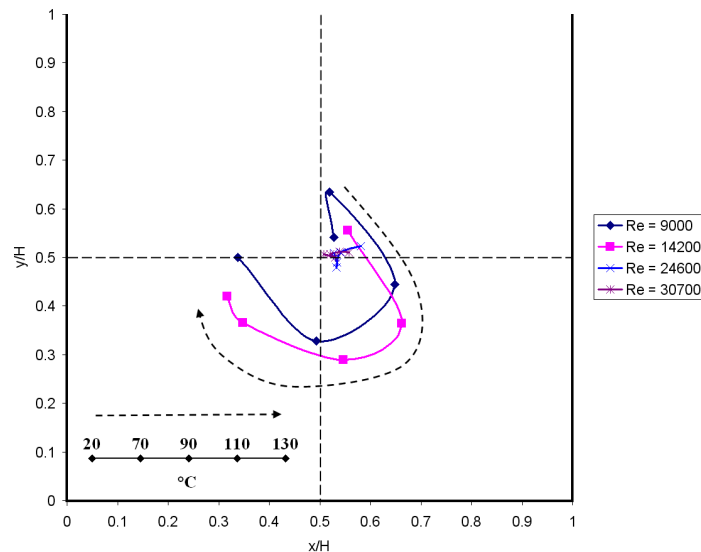
Figure 6.14: Trajectories of the centre of the main vortex as a function of the ground temperature for four different Reynolds numbers.
