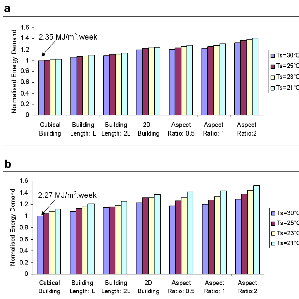
Figure 4.6: Weekly space cooling demands for a week with high wind speeds (a) and a week with low wind speeds (b) normalised by the results for the cubical building with T_s = 30\text{ }^\circ\text{C} for a street canyon with an aspect ratio of 1 using CHTC correlations developed for different geometries and temperature differences between building façades ( T_s ) and ambient air (here 20\text{ }^\circ\text{C} ).
