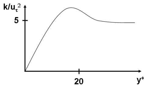
Figure 5.6: Schematic representation of the turbulent kinetic energy, scaled with the friction velocity as a function of the y^+ value for flat plate flow [181].
