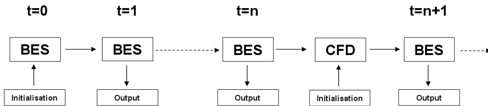
Figure 3.11: Schematics representation of the coupled model.
