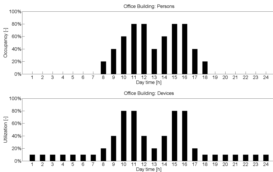
Figure 4.2: Utilization and occupancy schedules for office buildings.
