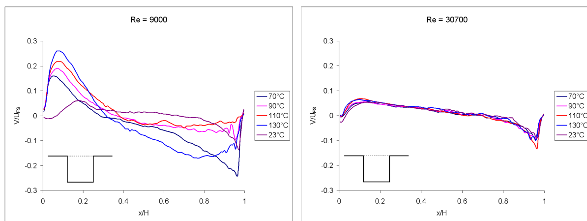
Figure 6.17: Normalised vertical velocity profiles at the top plane of the street canyon with different surface temperatures for two different Reynolds numbers.
