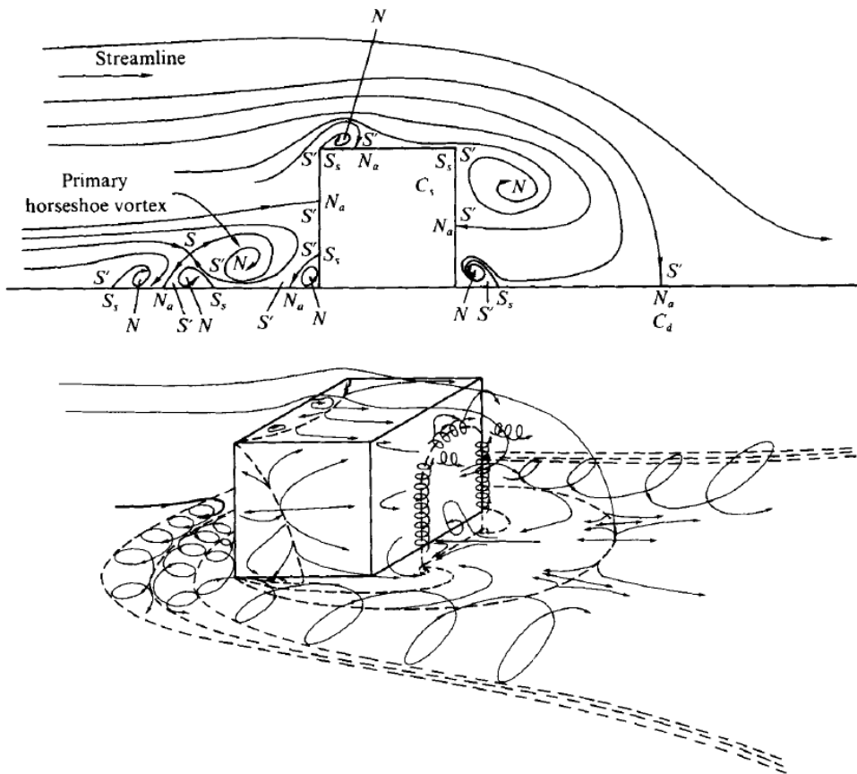
Figure 2.7: Sketch of the flow around a cube (taken from [70]).
