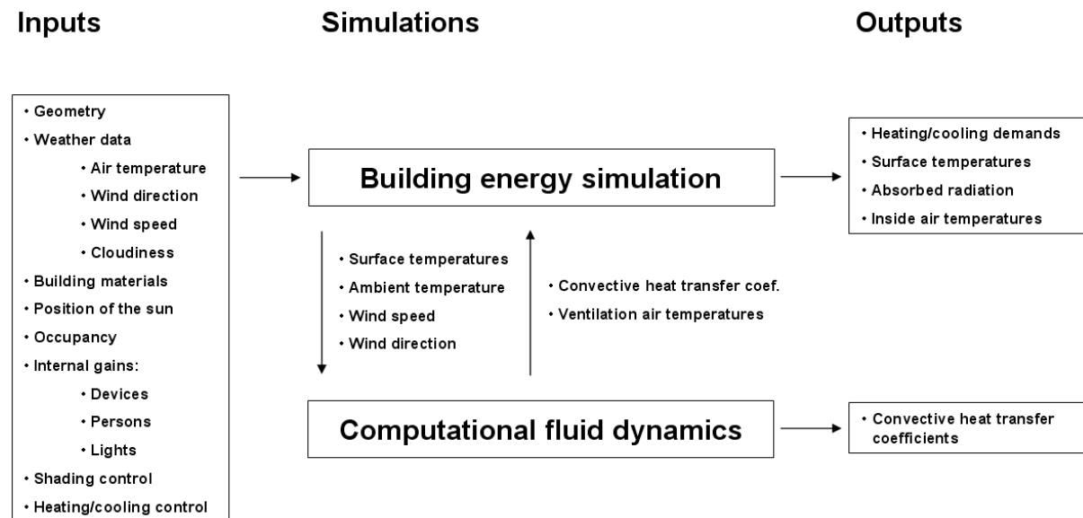
Figure 3.9: Schematics representation of the coupled model.
