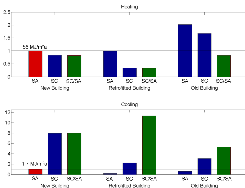
Figure 4.7: Annual space cooling and heating demands for three building types normalized by demands of the New stand-alone Building. Comparison between stand-alone buildings (SA) and buildings in street canyons (SC) with an aspect ratio of 1.
