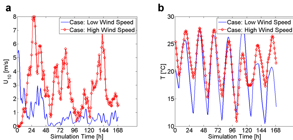
Figure 4.5: Wind speeds (a) and air temperatures (b) for the two studied weeks.
