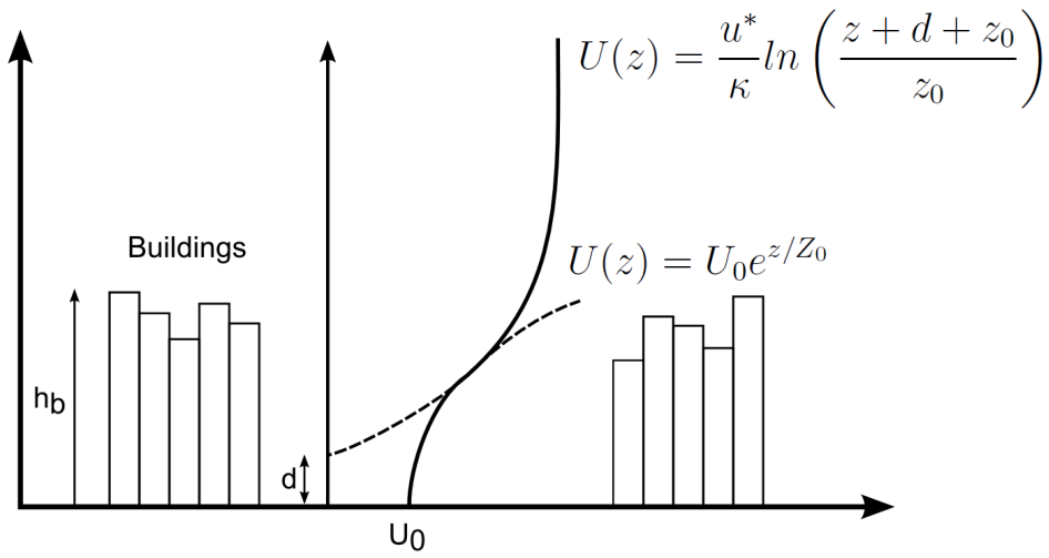
Figure 2.6: Sketch of an urban boundary layer (after [69]).
