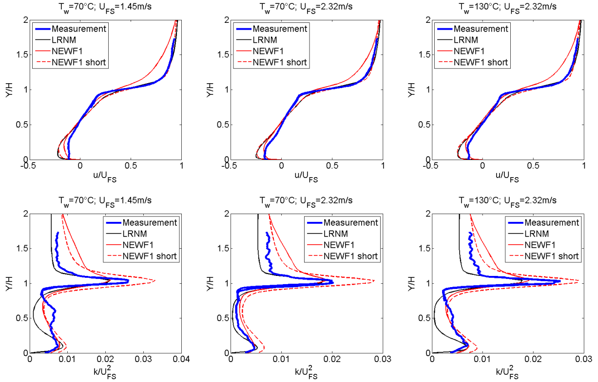
Figure 6.23: Normalised centreline profiles of the horizontal velocity and TKE. Wind tunnel measurements and CFD simulations for cases where all surfaces are heated using two different turbulence models and different near-wall modelling approaches (LRNM: Low-Reynolds number modelling with realizable k - \varepsilon ; NEWF1: non-equilibrium wall functions with standard k - \varepsilon ; NEWF1 short: NEWF1 with a short upstream domain).
