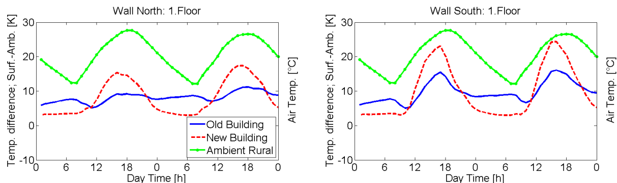
Figure 4.12: Differences between the wall surface temperature and ambient air temperature for the north and south façades of the first floor for the New and the Old Building with an aspect ratio of 1.
