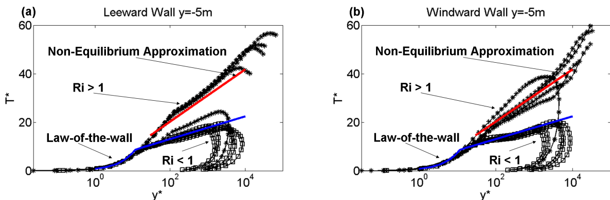
Figure 5.7: Dimensionless temperature profiles as a function of the y^* value along the horizontal centreline (see Figure 5.4b) of a street canyon for simulations with different global Ri numbers.
