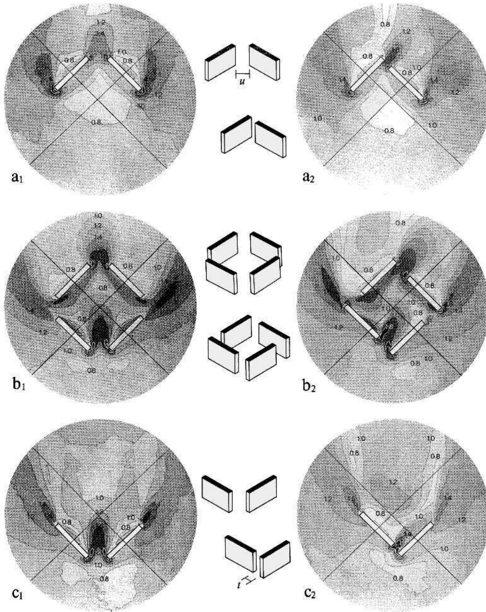
Figure 2.8: Flow around groups of buildings (taken from [71]).
