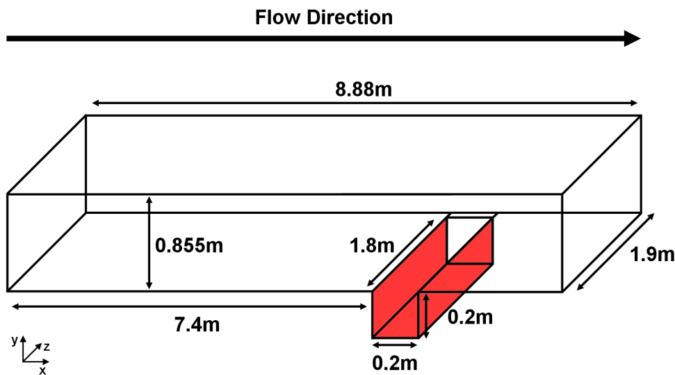
Figure 6.5: Dimensions of the wind tunnel model.
