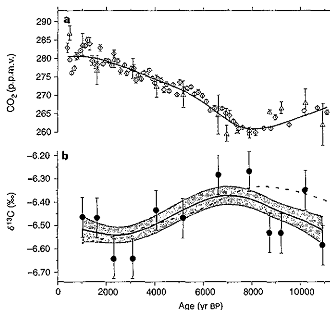
Figure 2 CO 2 concentrations and stable-isotope ratios, Taylor Dome. a , CO 2 concentrations. Open diamonds and triangles, mean CO 2 concentration. Error bars, 1\sigma of the mean. Solid line, spline fit 48 of the CO 2 results used as input for the single and double deconvolution. This spline fit method acts as a low-pass filter; parameters were selected to obtain a cut-off period of \sim 8,000 yr which is consistent with the low resolution of the \delta^{13}\text{C} record. b , Measured and calculated \delta^{13}\text{C} . Filled circles, \delta^{13}\text{C} values. Error bars, estimate of the reproducibility of the \delta^{13}\text{C} values. Solid line and shaded area, input values of \delta^{13}\text{C} for the Monte Carlo simulation. Dashed line, \delta^{13}\text{C} calculated with the single deconvolution 31 (land-biosphere-only hypothesis, h1; see text).
