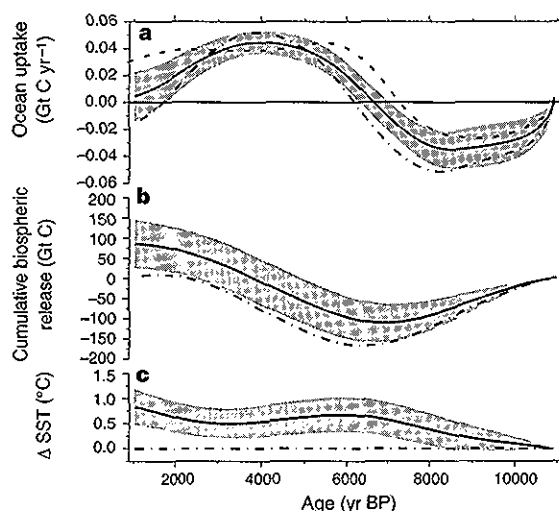
Figure 3 Comparison of our hypotheses. Dashed lines, land-biosphere-only hypothesis (h1). Solid lines, land biota–SST hypothesis (h2). The shaded areas indicate the 1 \sigma confidence interval of a Monte Carlo analysis, taking into account the uncertainty of the ice-core data. Dash-dotted lines, land biota–calcite hypothesis (h3). a, Ocean uptake. b, Cumulative biospheric release. c, Required change in SST.
