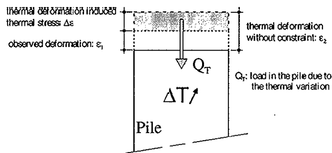
Figure 7 : Thermal stress in the pile
