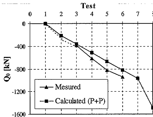
Figure 3 : Loading force at the top of the pile induced by the building during the construction of the each floor.
