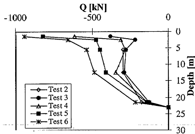
Figure 4 : Repartition of the weight in the pile after the construction of each floor and for the initial ground temperature ( \approx 11^\circ\text{C} )
