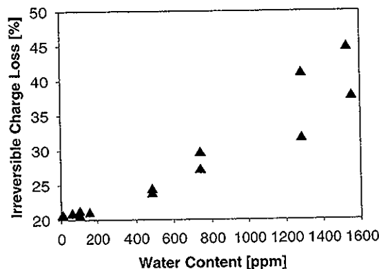
Fig. 2. Dependence of the irreversible charge loss of the graphite SFG 6 during the first cycle on the water content in the electrolyte (cell Li/1 M LiClO 4 in DMC+EC/SFG 6).
