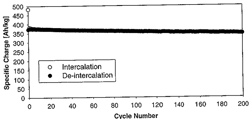
Fig. 1. Cycling performance of a negative electrode containing the graphite TIMREX SFG 6 with 5% carbon black, measured vs. lithium metal in the electrolyte 1 M LiClO 4 in DMC + EC. The cycling rate was \sim C/7 , and the specific charge is based on the weight of the graphite only.
