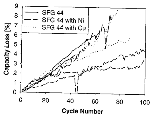
Fig. 6. Comparison of the capacity losses during galvanostatic cycling at a \sim C/7 rate of several SFG 44 electrodes without and with the metal additives copper and nickel (electrolyte 1 M LiClO 4 in DMC+EC; lithium counter-electrode).
