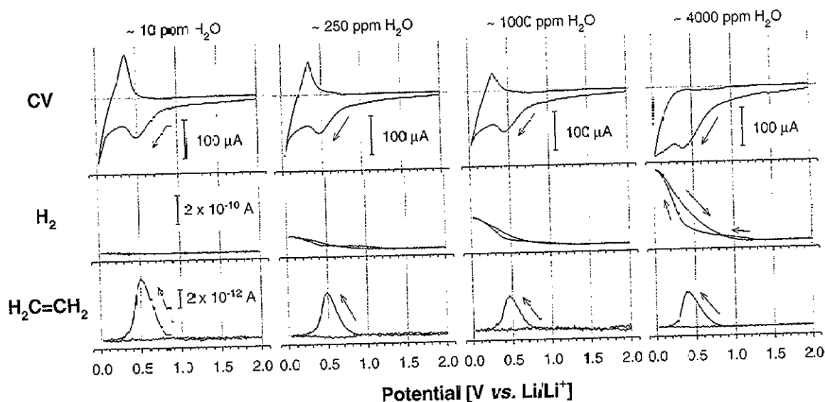
Fig. 3. Influence of water concentration in the electrolyte solution on the decomposition of 1 M LiClO 4 in DMC + EC: Cyclic voltammogram (CV) at 0.4 mV/s (first cycle) of the graphite SFG 6 and simultaneously recorded mass spectrometry cyclic voltammograms for the evolution of hydrogen (H 2 ) represented by m/z = 2 and ethylene (H 2 C=CH 2 ) represented by m/z = 27 .
