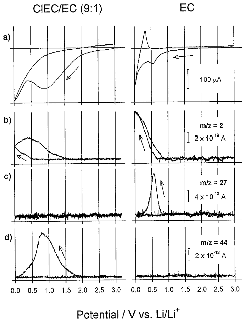
Fig. 4. CV (a) and MSCV (b, c, d) of graphite TIMREX® SFG 6 in 1 M \text{LiN}(\text{SO}_2\text{CF}_3)_2 in CIEC/EC (9:1) (left) and 1 M \text{LiN}(\text{SO}_2\text{CF}_3)_2 in EC (right). The MSCVs show m/z = 2 (b), m/z = 27 (c), and m/z = 44 (d), representing hydrogen, ethylene, and \text{CO}_2 , respectively.
