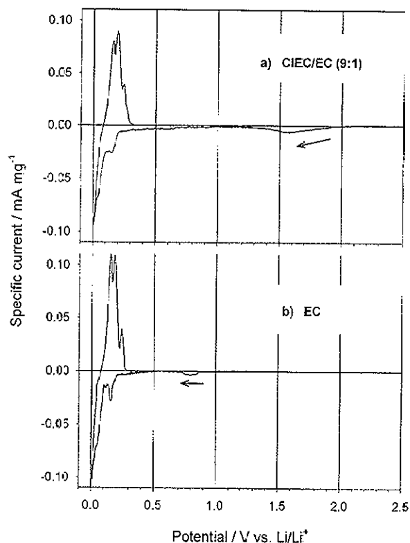
Fig. 1. Cyclic voltammograms of graphite TIMREX ® SFG 6 in (a) 1 M \text{LiN}(\text{SO}_2\text{CF}_3)_2 in CIEC/EC (9:1), and (b) in 1 M \text{LiN}(\text{SO}_2\text{CF}_3)_2 in EC, scan rate = 0.01 \text{mV s}^{-1} .
