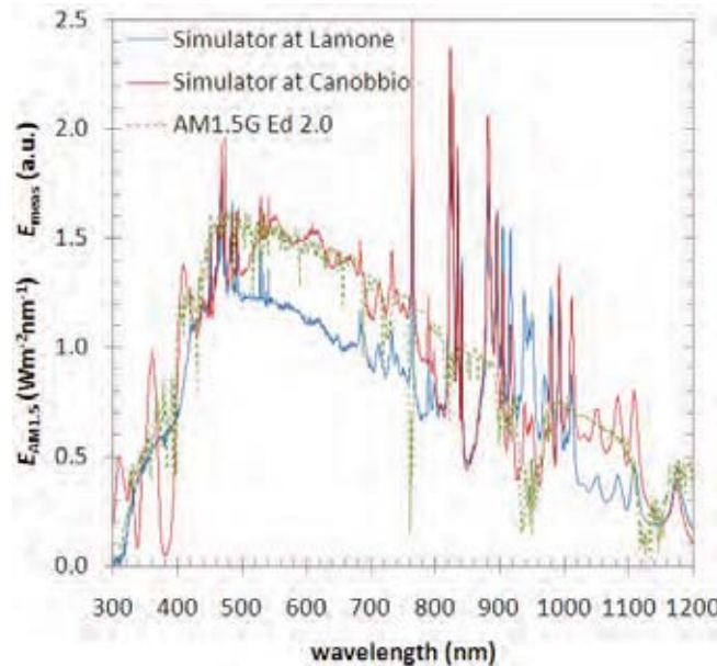
Figure : Comparison of relative spectral irradiance measurements of the two flash solar simulators used at SUPSI. In the laboratory at Canobbio, a class AA – AA – AA sun simulator Pasan IIIB is in use. It provides a stable 10 ms light pulse with a high fidelity spectrum w.r.t. AM1.5G. The measurements are compared to the AM1.5G Ed. 2 spectrum.
