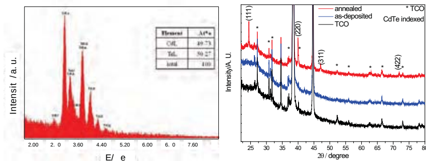
Figure 7: a) EDX spectra of CdTe, b) XRD patterns of bare TCO, as-deposited CdTe and annealed CdTe in argon atmosphere at 400 °C for 1 h
