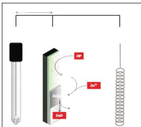
Figure 3. Schematic diagram of ZnO growth setup and mechanism by ECD.
