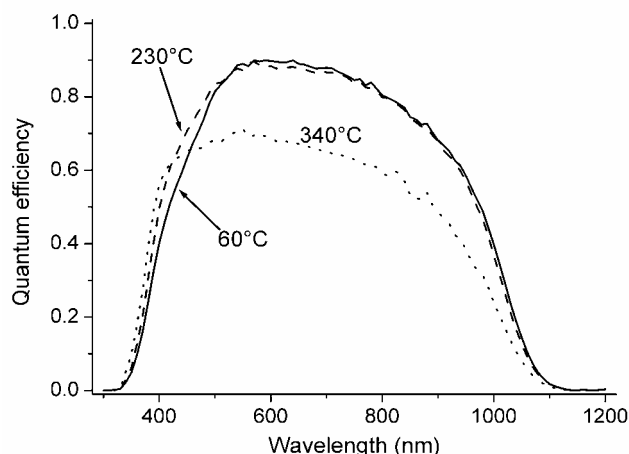
Figure 2: External quantum efficiencies of the 60, 230 and 340 °C samples. Reduced carrier collection was found for the 340 °C sample, compared with the 60 and 230 °C samples.
