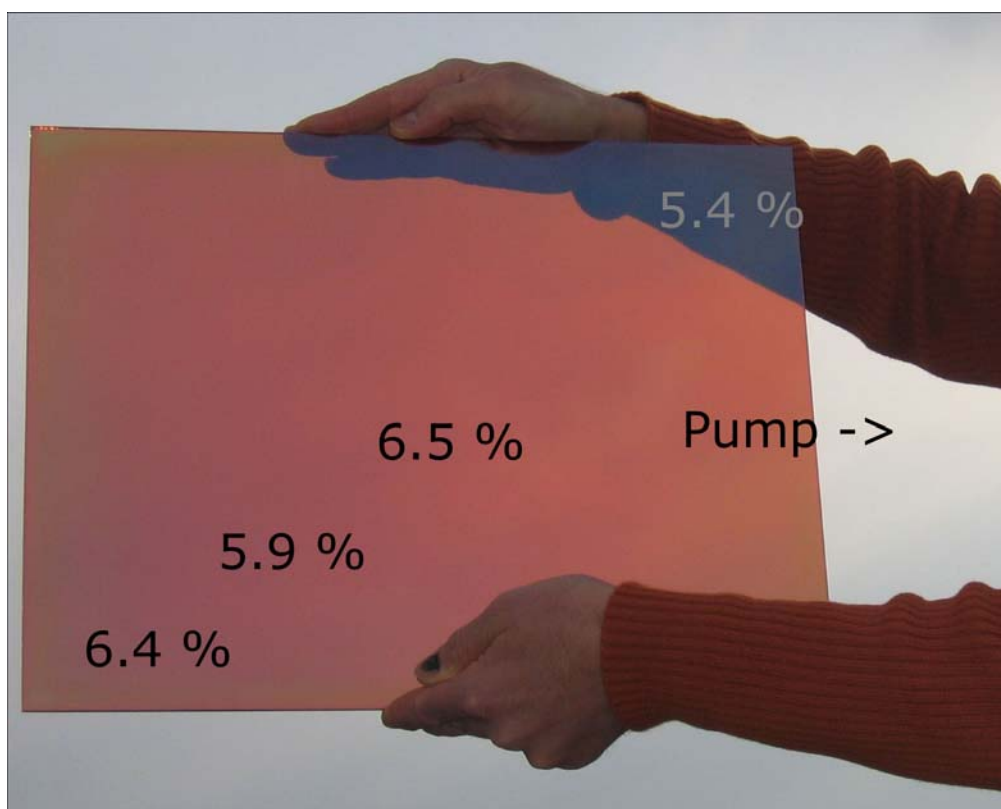
Fig. 2: Distribution of conversion efficiencies of solar cells deposited along the whole electrode ( 35 \times 45 \text{ cm}^2 ), represented here on a \mu\text{c-Si:H} high-rate film on glass. Cell thickness : 1 \mu\text{m} , deposition rate 0.7 nm/sec, deposited in the KAI-S reactor at IMT.
