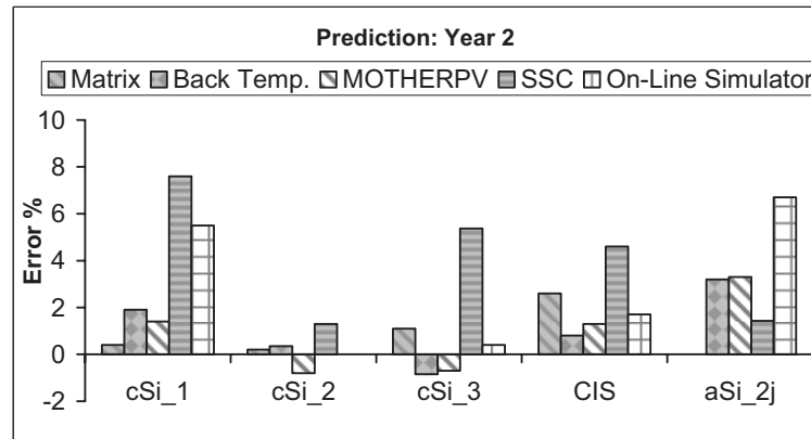
Figure 2: Shows the error between the measured and the predicted energy yield for year 2 dataset from the difference centers.
