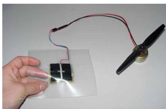
Figure 3: Pictures of flexible CIGS solar cell layers on a roll (left) and flexible mini-module to run a ventilator-fan.
