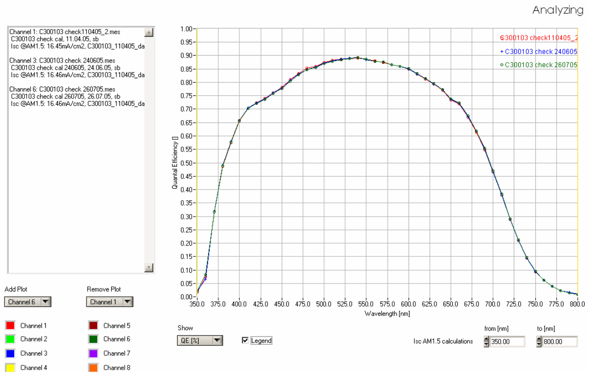
Fig 2: Evidence of SR apparatuses stability: Control measurements of a calibration device by the SRMS system A. The red curve represents the control QE-data of the device immediately after calibration on April 11, 2005. The following control with measurements done on 24 th June, 2005 (blue curve) and of 26 th July 2005 (green curve) show perfect stability of the QE system. Note that the system is always based on the calibration done on April 11, 2005.
