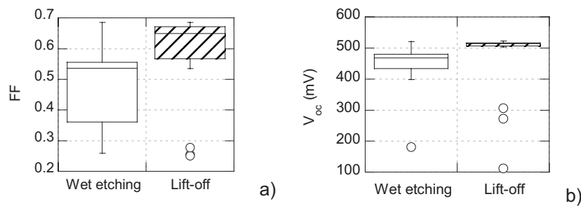
Fig.1: a) and b) fill-factor (FF) and the open-circuit voltage ( V_{oc} ) obtained with two different patterning techniques: wet etching (old) and lift-off (new) technique. The measurements were done on 16 single cells in both cases. The outliers (open-circle) are caused by localized shunts.
