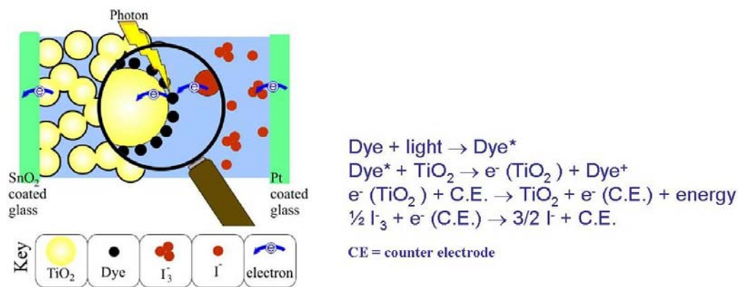
Figure 2: The principle of a DSC cell
