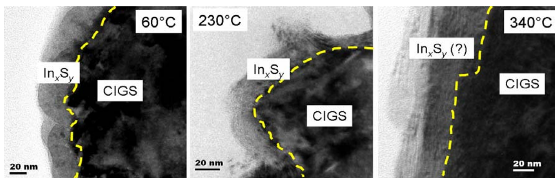
Figure 3: Bright-field transmission electron micrographs of the interfaces of CIGS with \text{In}_x\text{S}_y layers grown at 60, 230, and 340 °C. All three samples show inhomogeneous \text{In}_x\text{S}_y layer thicknesses, varying between 25 and 100 nm. For the 340 °C sample, a layered structure is found.
