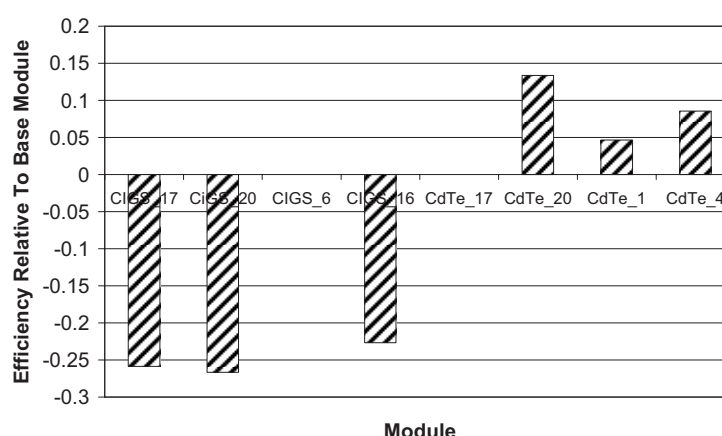
Figure 10: Efficiency of the different modules relative to the base module.
