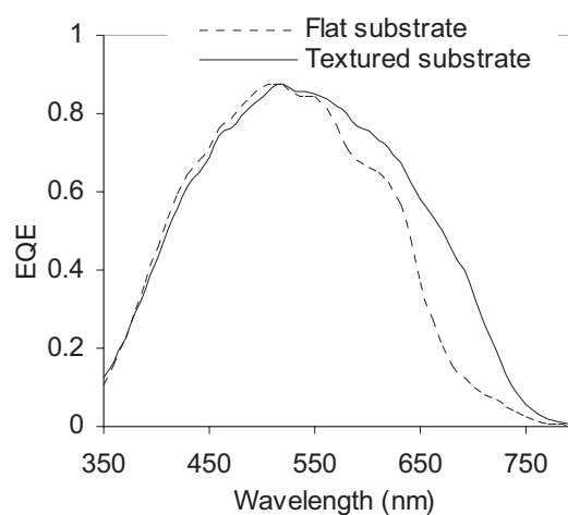
Fig. 2: Comparison of the External Quantum Efficiency (EQE) of the standard a-Si:H solar cells deposited at the IMT on flat substrate and on the new “second generation” textured film
