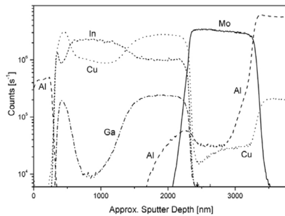
Figure 5: SIMS depth profile of CIGS/Mo layers in solar cells grown on Al foils at 500^\circ\text{C} . Diffusion of Al through the Mo back contact and contamination of CIGS is observed. The Ga-dip/In-peak is due to the 3-stage process and low In-Ga inter-diffusion at low temperature.
