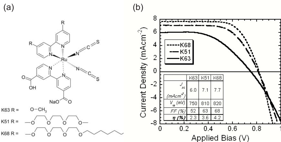
Figure 7: a) The sensitizer molecules used in this study; b) current-voltage characteristics under simulated AM 1.5 solar conditions at 100 \text{ mW cm}^{-2} for solid-state dye-sensitized solar cells incorporating K63 sensitizer (solid line), K51 sensitizer (dot-dashed line) and K68 sensitizer (dotted line). The inserted table shows the device performance values.
