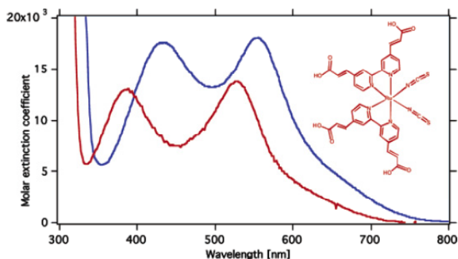
Fig.3: Structure of K8 (inset) and comparison of VIS-UV absorption spectrum with that of the prototype dye N3.
