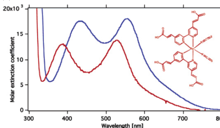
Fig.8: Molecular structure and optical properties of the dye K8.
