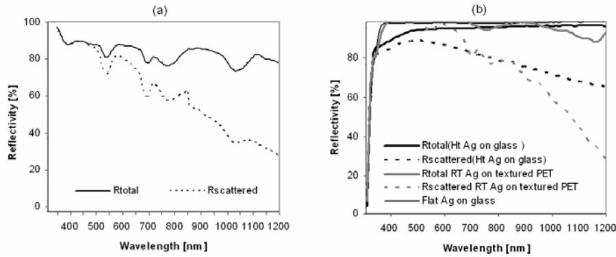
Fig. 4: (a) Total and scattered reflectivity of the Al-based back contact currently available at IMT on textured PET substrates. (b) Total and scattered reflectivity of the Ag-based back contacts currently available at IMT on glass (as-grown textured Ag deposited at high temperature and flat Ag deposited at room temperature) and on textured PET films.
