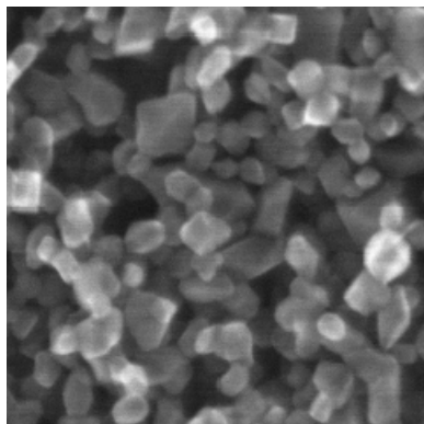
Fig. 6: SEM image of photovoltaic-quality titania mesoporous film
