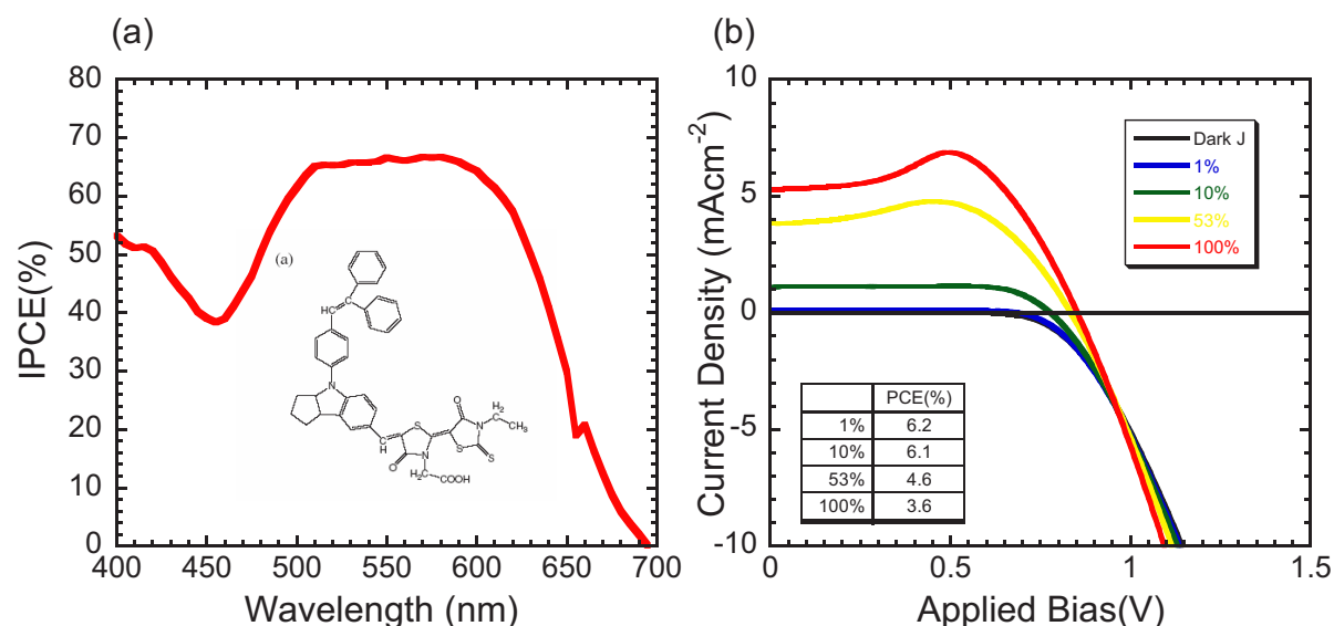
Figure 8: a) Incident photon-to-electron conversion efficiency spectrum for a solid-state dye-sensitized solar cell incorporating an indoline based organic dye: the inserted figure is the chemical structure of the dye. b) Current-voltage characteristics of a similar device to that measured in (a) under simulated solar AM 1.5 illumination over a range of illumination intensities.
