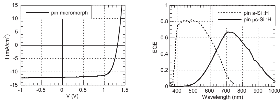
Fig. 3: I-V curve and external quantum efficiencies (EQE) of the best micromorph tandem solar cell fabricated in 2005 with a conversion efficiency of 11.6% (see Table 1).
