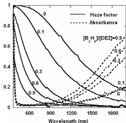
Fig. 6 : Absorbance and haze factor (i.e. diffuse / total transmittance ratio) curves for LP-CVD ZnO series deposited with various doping ratios (i.e. B_2H_6/DEZ ratio). All Layers with 10 \Omega_{sq} . [Ste05].
