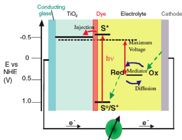
Fig.2: Principle of operation of the dye-sensitised nanocrystalline solar cell. Photoexcitation of the sensitizer (S) is followed by electron injection into the conduction band of an oxide semiconductor film. The dye molecule is regenerated by the redox system, which itself is regenerated at the counter electrode by electrons passed through the load. Potentials are referred to the normal hydrogen electrode (NHE).
