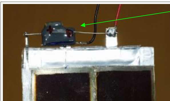
DC/DC converter connected to Li-ion battery and Dye Solar Cell module with 2 cells forming the Euro-PSB assembly
