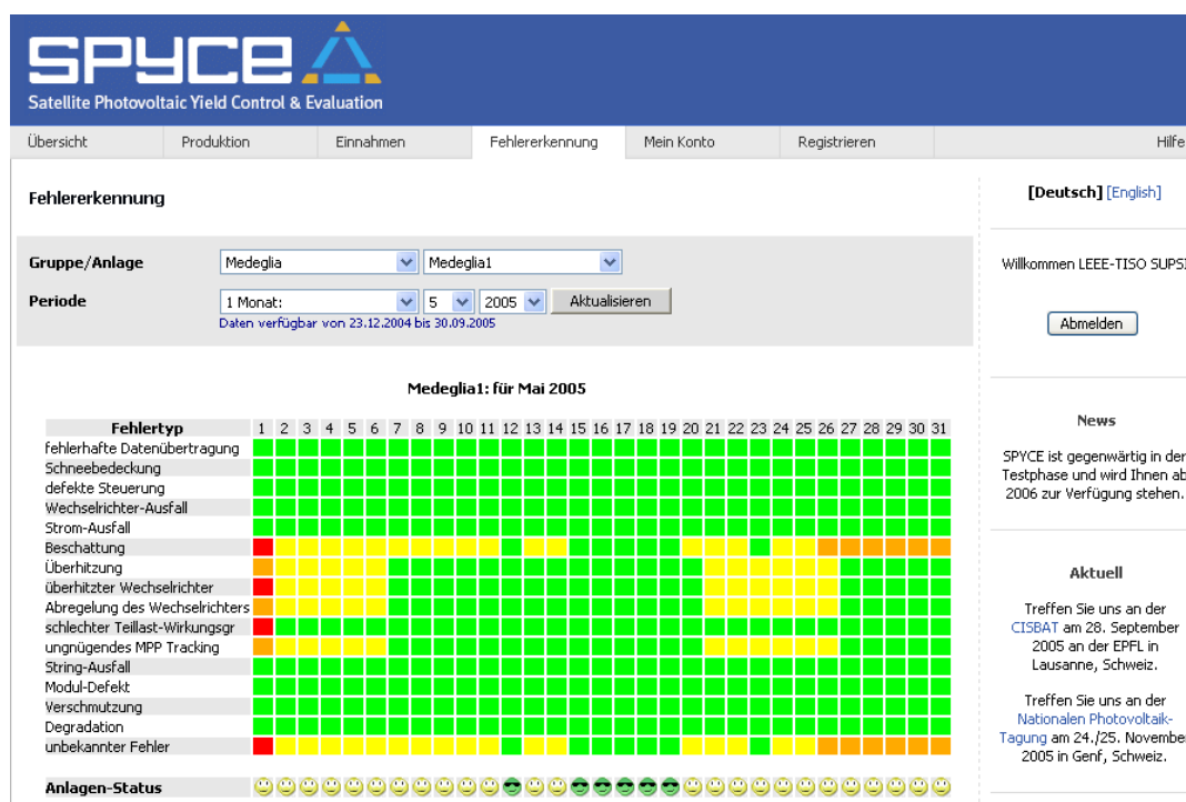
Figure 5: results of the Failure Detection Routine for a PV system with shading and power limitation at days with high irradiance
