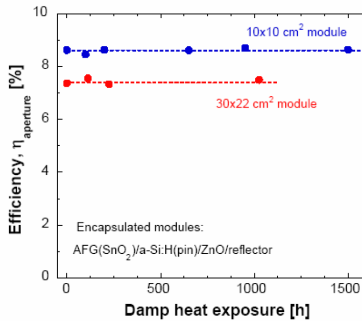
Fig 1 Evolution of the efficiency of encapsulated solar modules submitted to damp-heat test. These modules use LP-CVD ZnO as back contact.
