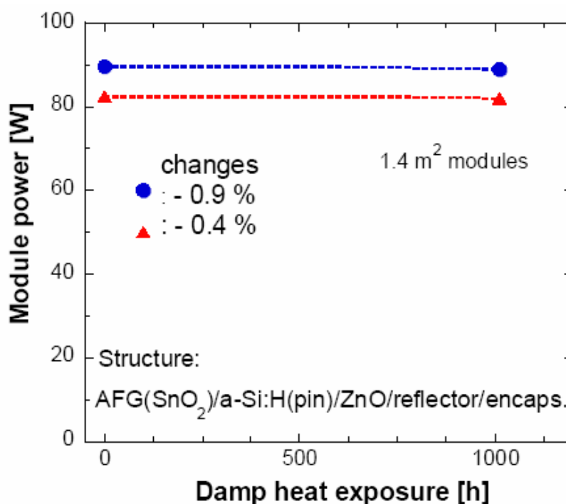
Fig 3 Damp heat experiments of 1.4 m 2 a-Si:H modules performed and characterized by TÜV Rheinland (Germany). Both modules show a good stability and a change of less than 1 % after 1000 h of damp heat exposure.
