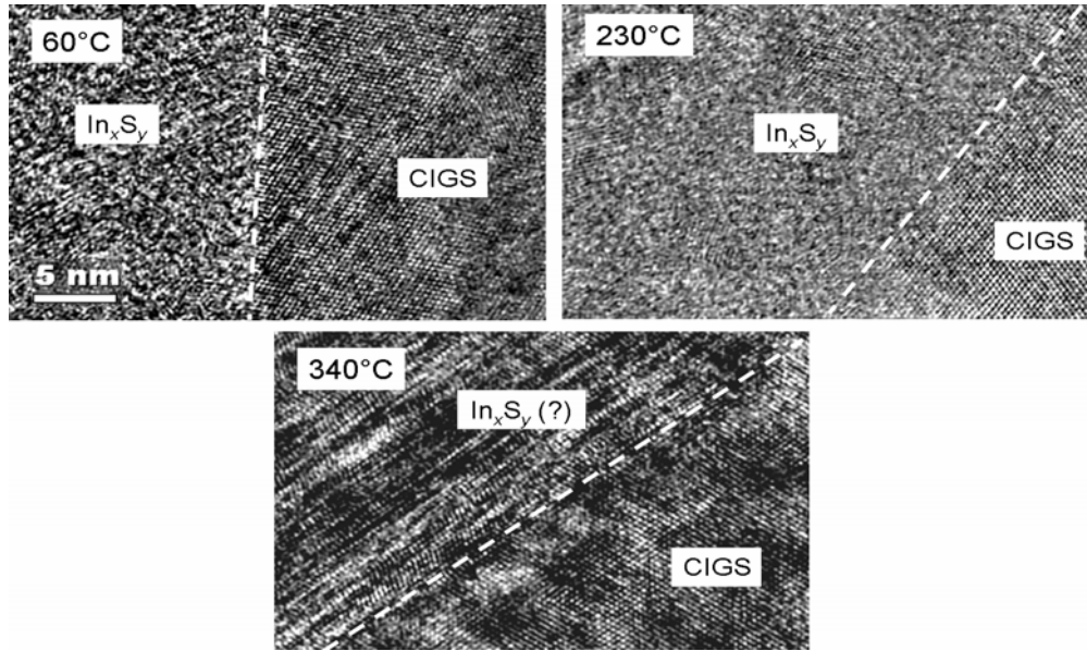
Figure 4: High-resolution transmission electron micrographs of the interfaces of CIGS with \text{In}_x\text{S}_y layers grown at 60, 230, and 340 °C. A large density of planar defects is revealed in the buffer layer of the 340 °C sample, directly at the interface to CIGS.
