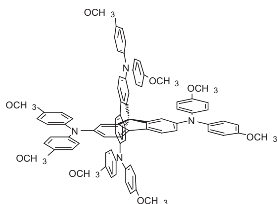
Figure 1: structure of spirobifluorene hole-conducting p-type organic semiconductor. The fluorene structures are perpendicular, conjoined through a common carbon site.
