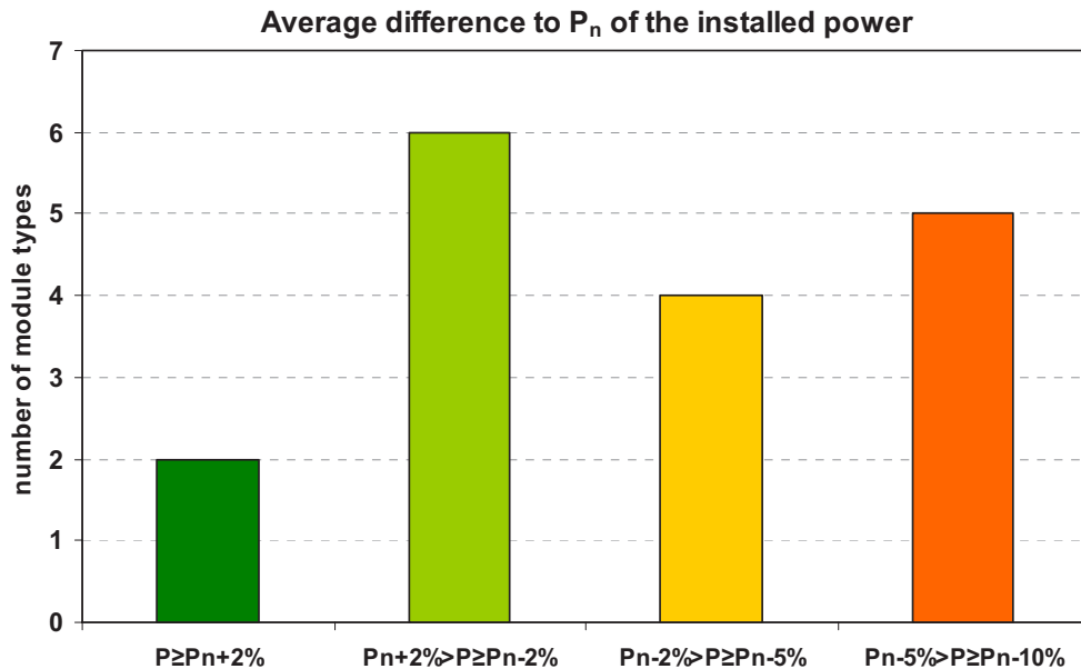
Figure 1: Power measured after light soaking: Number of module types with an average difference in the range of P_n + x\% > P_{\text{meas,avg}} > P_n + y\% .
