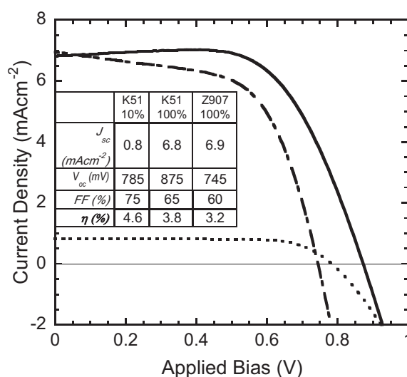
Figure 6: Current voltage characteristics under simulated AM 1.5 solar conditions ( 100 \text{ mWcm}^{-2} ) for a full device containing K51 sensitizing dye (solid line) and Z907 sensitizing dye (dot-dashed line). Also shown is the K51 device illuminated by 10 \text{ mWcm}^{-2} simulated sun light. The standard device performance parameters, as calculated from the JV data, are displayed in the inserted table.
