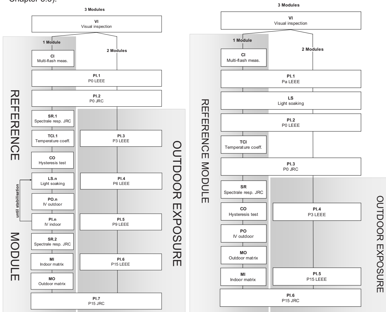
Figure 3: Thin-Film modules test procedure (left) and crystalline silicon test procedure (right).
