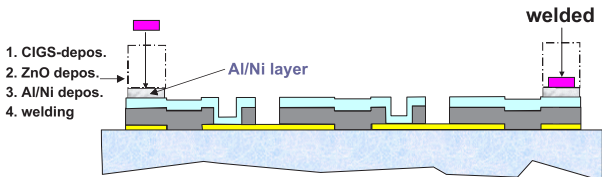
Fig. 3 Ultrasonic welding
