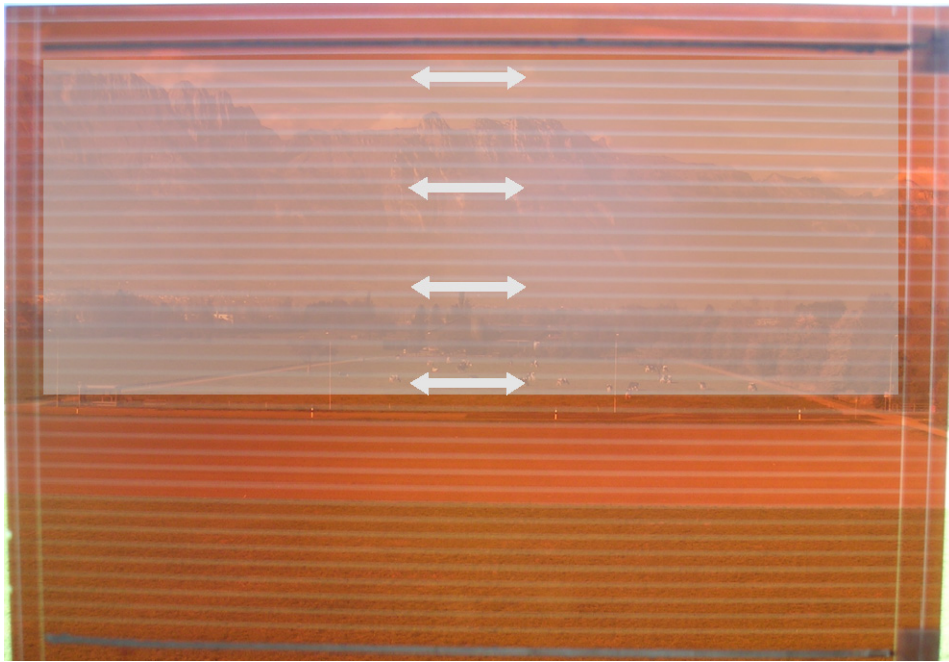
Fig. 6: Photograph of an a-Si:H p-i-n module (300x220mm), the marked white area indicates the scanned section with the results shown in Fig. 7
