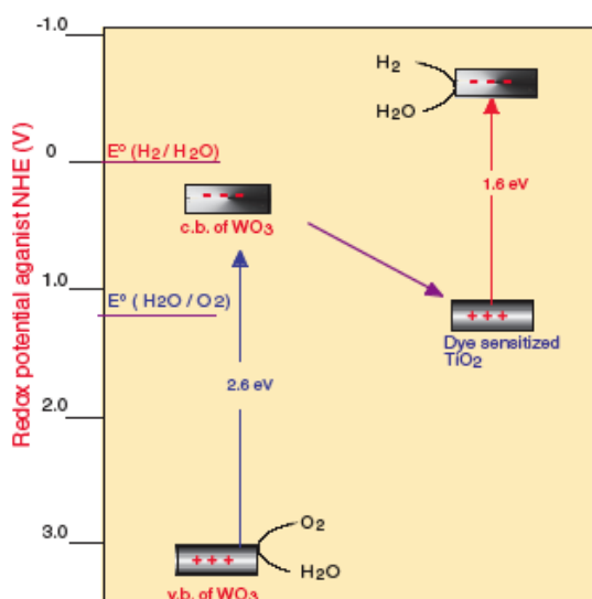
Fig.5: schematic of energy levels and electrical series connection of a tandem arrangement for solar photoelectrolysis. As stated in the text, the two photosystems are also in optical series.
