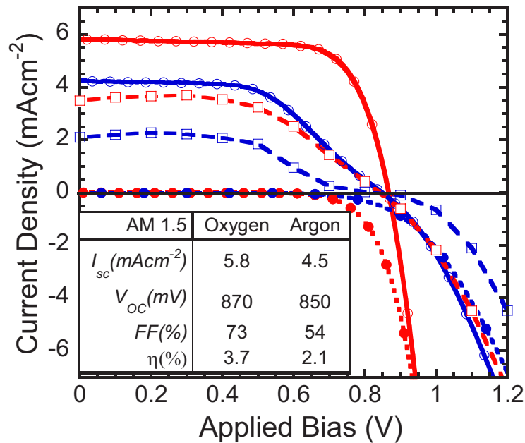
Figure 5: Current-voltage curves for solid-state dye sensitized solar cells incorporating an “oxygen-sprayed” compact layer (red curves) and an “argon-sprayed” compact layer (blue curves), in the dark (dotted lines, solid circles), under monochromatic 514 nm incident illumination with an intensity of 25 \text{ mWcm}^{-2} (dot-dashed lines, open squares) and under simulated AM 1.5 solar conditions at 100 \text{ mWcm}^{-2} (solid lines, open circles).
