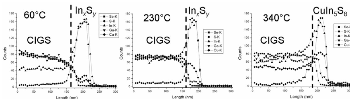
Figure 6: Linear elemental distribution profiles across CIGS/ \text{In}_x\text{S}_y interfaces. Cu and Ga diffusion from CIGS into \text{In}_x\text{S}_y are revealed, as well as Cu depletion on the CIGS side of the interface for the 230 and 340 °C samples. Only for the 340 °C sample, also enhanced In enrichment on the CIGS side of the interface was found. All effects increase with increasing \text{In}_x\text{S}_y deposition temperature.
