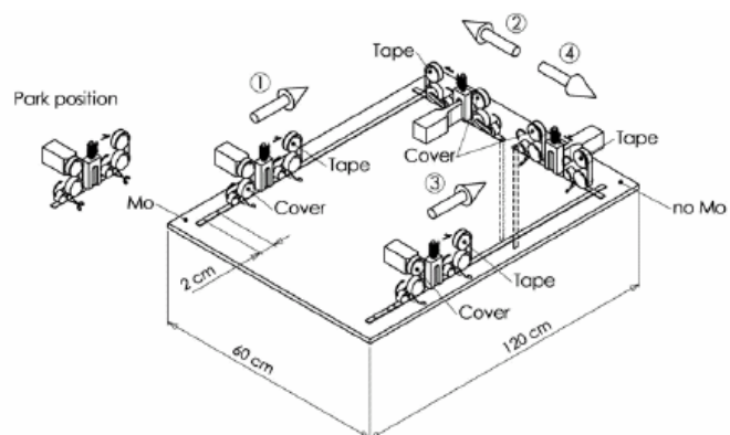
Fig. 4b Welding sequence
