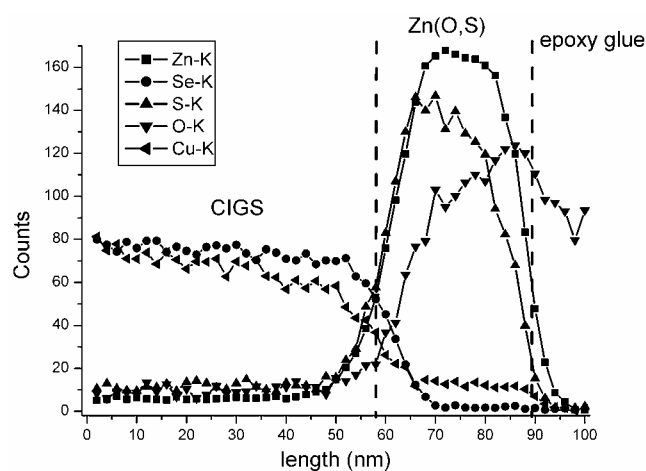
Figure 8: Elemental distribution profiles across the interface between CIGS type 2 and Zn(O,S)10%, obtained by energy-dispersive x-ray spectrometry.
