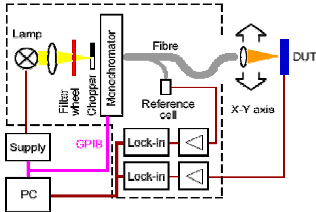
Fig. 4: Functional principle of the Spectral Response Measurement System (SRMS)
