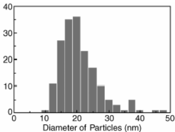
Fig.7: Histogram showing the frequency of occurrence of a given particle size for a mesoscopic \text{TiO}_2 film prepared at 230^\circ\text{C} , which has demonstrated optimal photo-voltaic performance.
