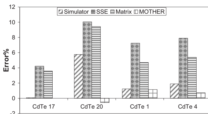
Figure 9: Accuracy of site-to-site (Widderstall/Helsinki) and module-to-module prediction of similar CdTe modules but with different power ratings
