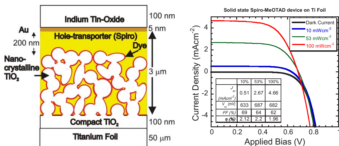
Figure 4: a) The scheme of a solid-state dye-sensitized solar cell fabricated on a titanium foil substrate.
