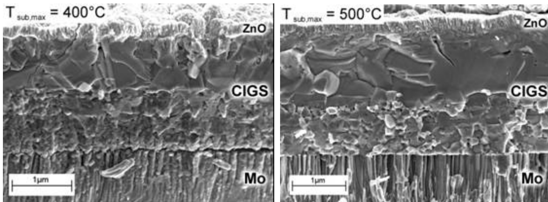
Figure 4: SEM cross-section images of solar cells on Al foils where CIGS layers were grown at a 400^\circ\text{C} (left) and 500^\circ\text{C} (right), the mentioned temperature is a reference value and not the exact substrate temperature.
