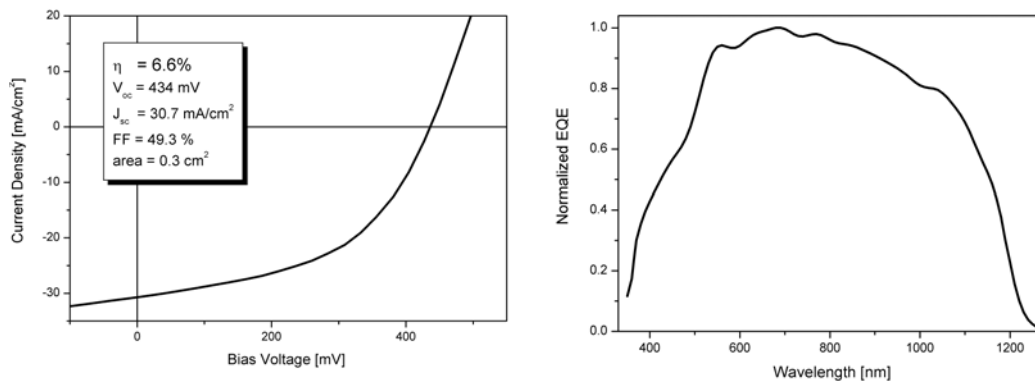
Figure 6: Current-voltage characteristic (left) and quantum efficiency (right) of a CIGS solar cell on Al foil. Neither Na was incorporated in CIGS absorber nor any AR coating was applied. This 6.6% efficiency is the highest value of efficiency reported to date for CIGS cell on Al foil. Addition of Na in CIGS will further increase the cell efficiency.
