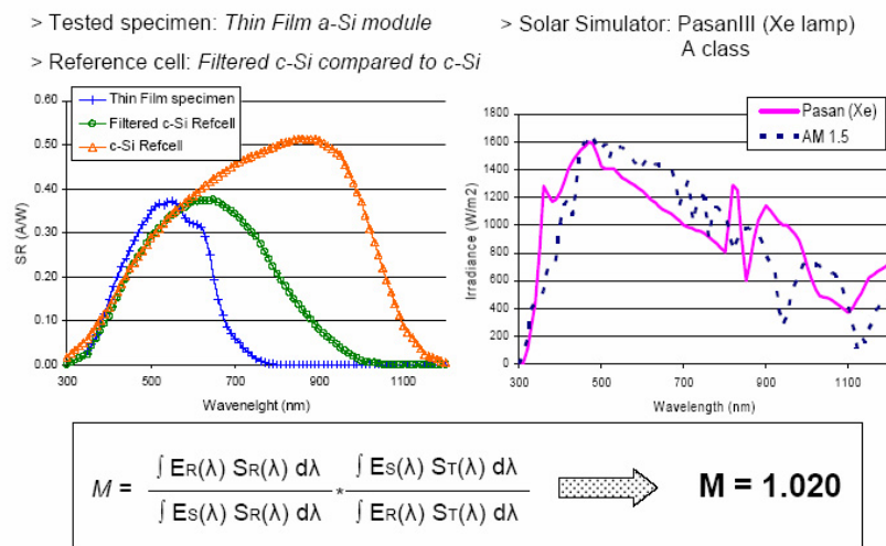
Figure 1: Spectral response of an a-Si single-junction module and the two reference cells (filtered e non-filtered), spectrum of the Xe-lamp and of the AM1.5 reference.
