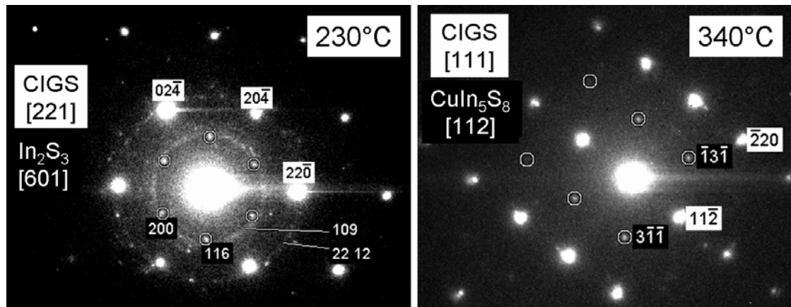
Figure 5: Selected-area electron diffraction patterns from the interfaces of CIGS with \text{In}_x\text{S}_y layers grown at 230 and 340 °C. A tetragonal \beta\text{-In}_2\text{S}_3 crystal structure was revealed for the 230 °C sample. For the 340 °C sample, cubic \text{CuIn}_5\text{S}_8 formed instead of \text{In}_x\text{S}_y . The reflections from the \text{CuIn}_5\text{S}_8 layer are barely visible, thus, there were outlined by circles.
