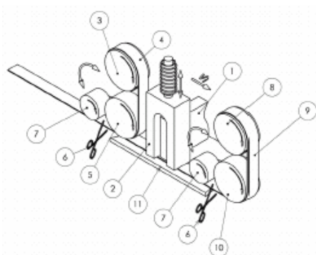
Fig. 4a Concept of welding/tapes application head
