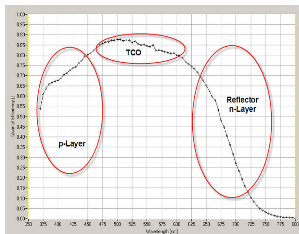
Fig 3: Quantum efficiency (QE) of an a-Si:H cell, sub layers are characterized by red areas
