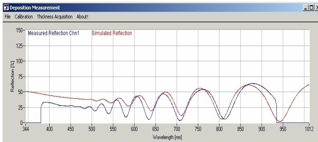
Fig 3: User Interface of the thickness measuring tool (developed by NTB), where for comparison the measured data and the fitted spectrum of an a-Si:H layer of 690 nm on glass is plotted.
