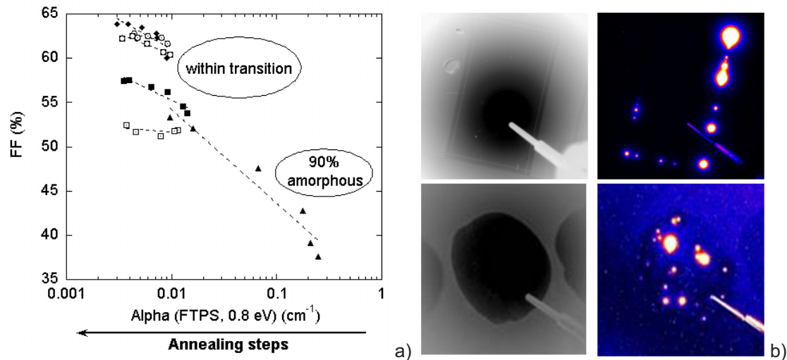
Fig. 7 a) FF of solar cells as a function of defect densities measured by FTPS, for \mu\text{c-Si} solar cells with different crystalline fraction b) IR images (left) and IRLIT images (right) of sample with different shunt structures. Temperature scale for the IRLIT image: 3 mKelvin..
