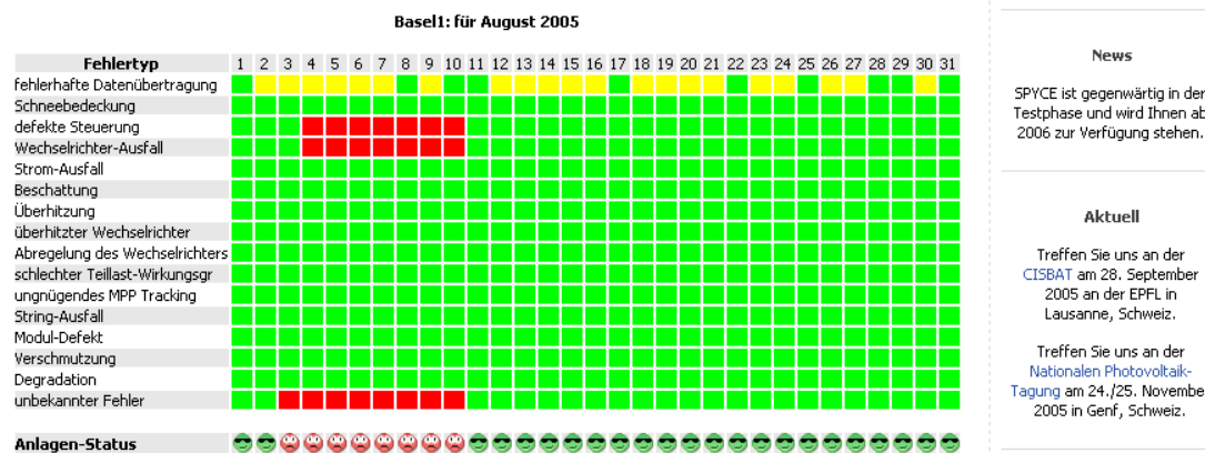
Figure 4: results of the Failure Detection Routine for a PV system with defect inverter from 4th to 10th August 2005
