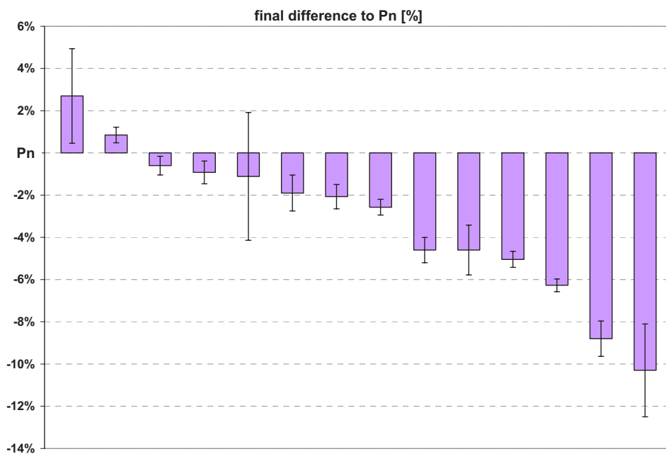
Figure 2: Power measured after light soaking: Average deviation from nominal power P_n with the standard deviation of the measured modules (6-8).
