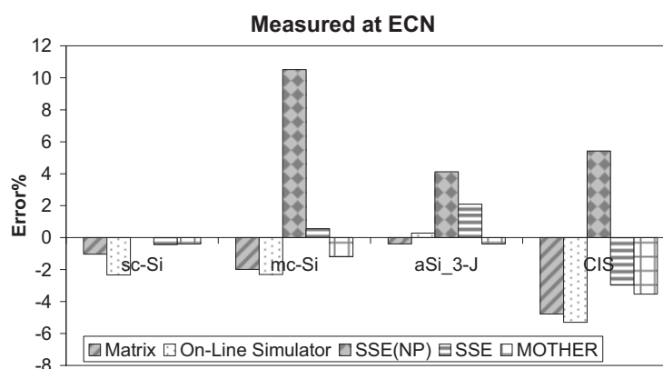
Figure 6: Prediction of the Energy Yield at ECN
