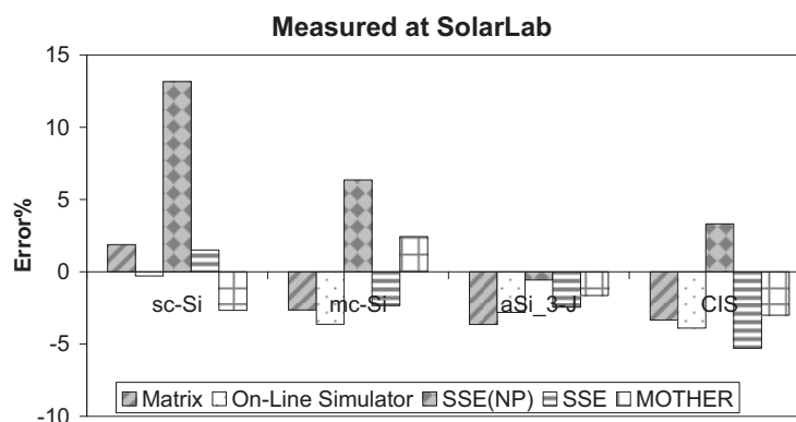
Figure 5: Prediction of the Energy Yield at SolarLab
