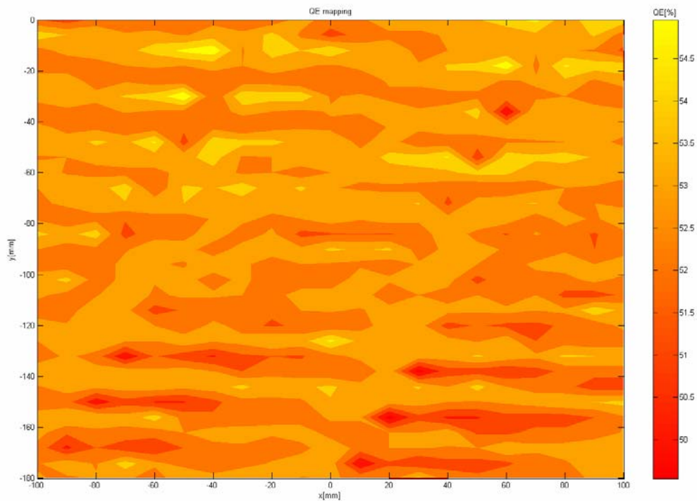
Fig. 7 QE (quantum efficiency, spectral photocurrent) mapping results on an UNAXIS a-Si:H prototype module (1.4m 2 ) shown in the sub-area of 200x180mm 2 . The deviation of the measured QE uniformity is within +/- 2.5% at a wavelength of 550nm (based on 360 individual measurement positions in the scanned area)
