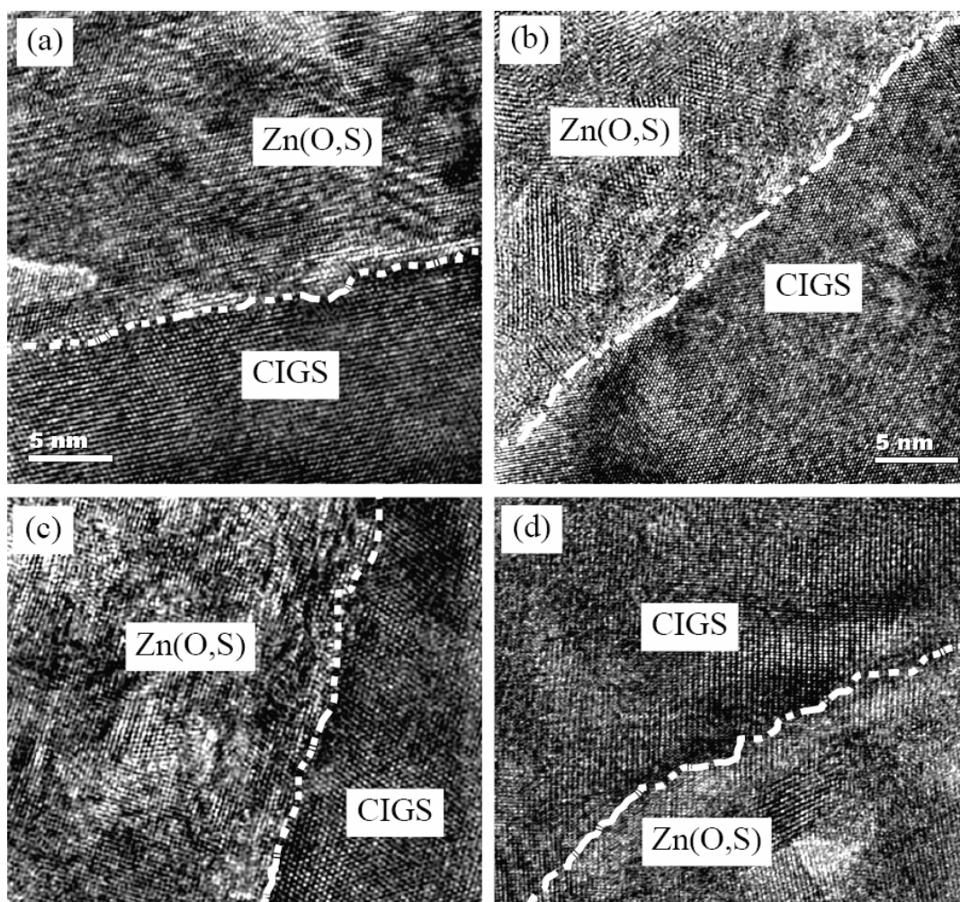
Figure 7: High-resolution transmission electron micrographs of interfaces between CIGS type 1 and Zn(O,S)5% (a), Zn(O,S)20% (b), Zn(O,S)10% (c), and between CIGS type 2 and Zn(O,S)10% (d).
