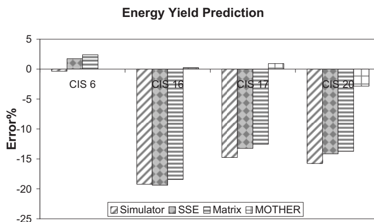
Figure 8: Accuracy of site-to-site (Widderstall/Helsinki) and module-to-module prediction of similar modules but with different power ratings
