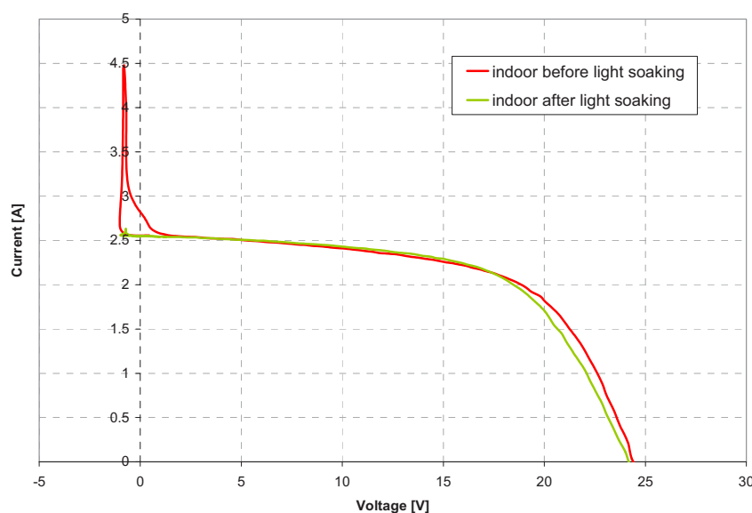
Figure 3: IV curves of a indoor measured CIS module (ST40) before and after light soaking.
