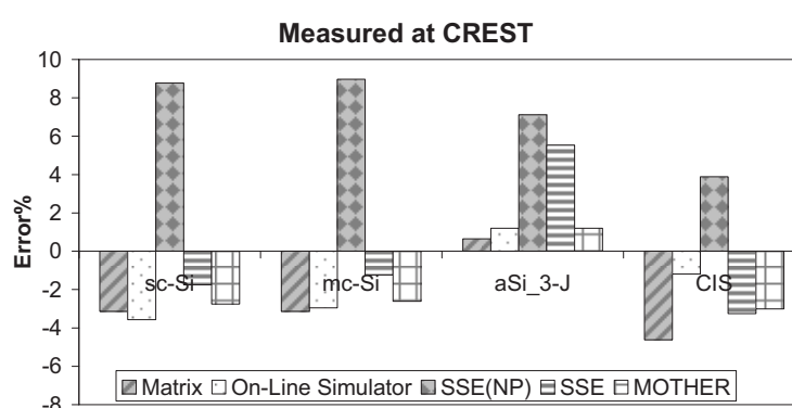
Figure 7: Prediction of the Energy Yield at CREST
