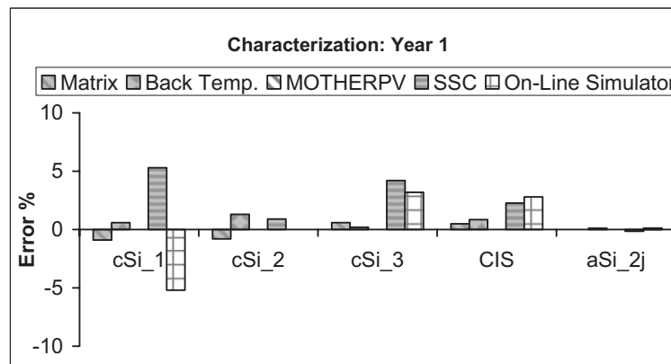
Figure 1: Shows the error between the measured and modeled energy yield for year 1 dataset from the difference centres.
