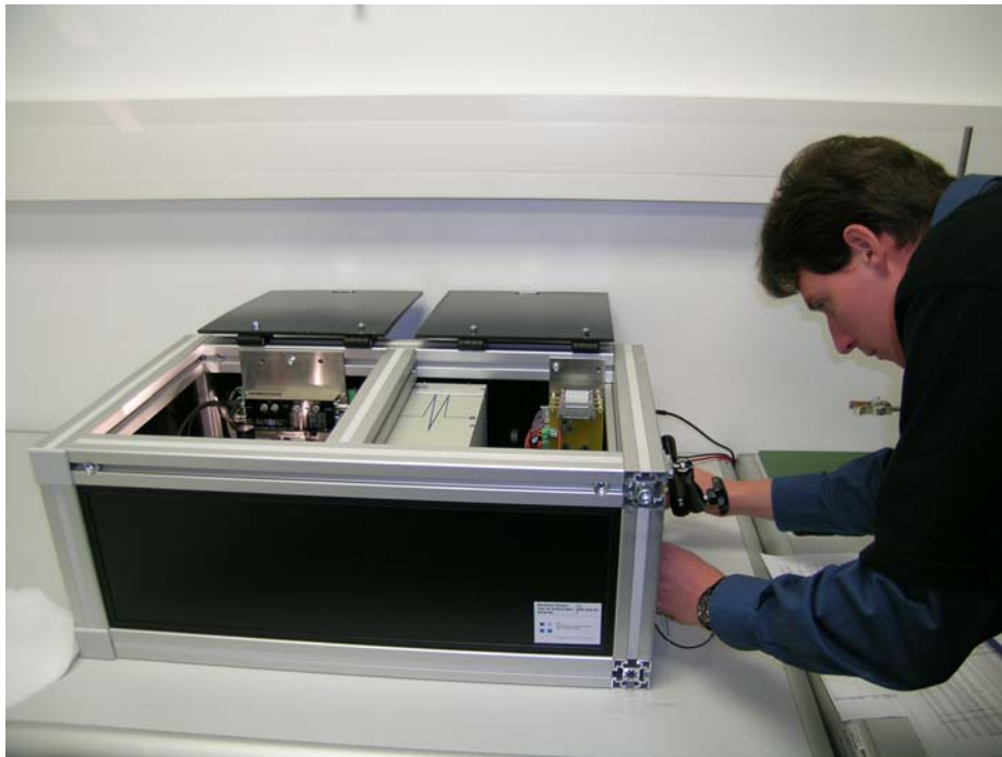
Fig. 1: Compact and well-designed SRMS A at Neuchâtel.
