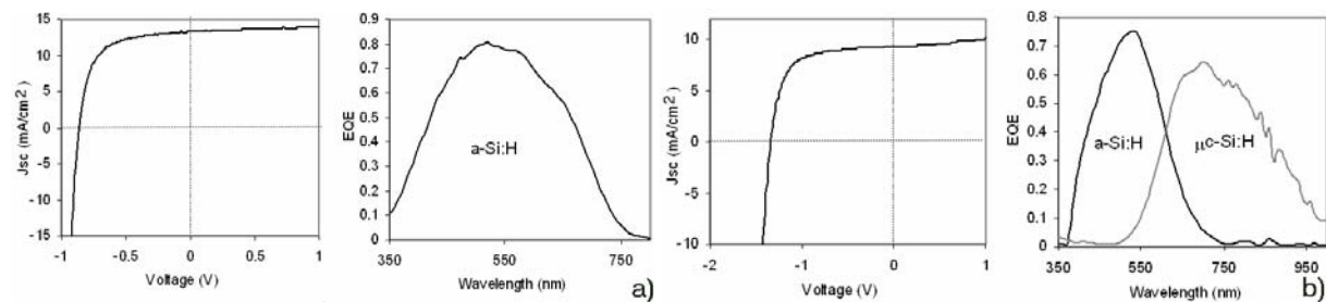
Fig. 5: a) I-V and EQE curves of the a-Si:H solar cells deposited on PET substrate. The back reflector consisted in Al and ZnO layers deposited by sputtering. ITO was used as top contact. b): IV and EQE curves of the micromorph solar cell deposited on PET substrate. The back reflector consisted in Ag and ZnO layers deposited by sputtering. LPCVD-ZnO was used as top contact.
