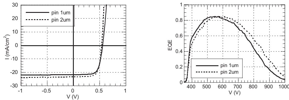
Fig. 2: I-V curves and external quantum efficiencies (EQE) of 1 and 2 microns thick p-i-n microcrystalline silicon solar cells deposited on LPCVD ZnO.
