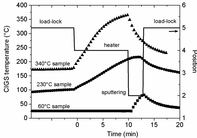
Figure 1: Substrate temperatures and positions of the samples in the sputtering chamber in dependence of the duration. The samples were termed after the average substrate temperature during the sputtering, 60, 230, and 340 °C.
