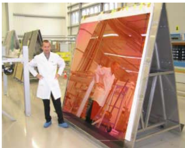
Fig. 1: \text{a-Si:H} film deposited on glass of 5\text{ m}^2 area of Unaxis' most recent generation of KAI reactor.
