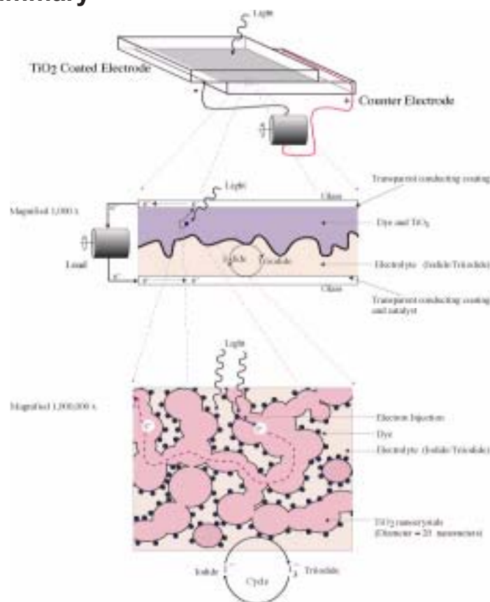
Fig.1: Structure of dye-sensitised photoelectrochemical cell on different scales. (Top): a complete cell (centimeter scale). (Centre): electrodes and electrolyte, micron scale. (Bottom) nanoscale semiconductor interconnected porous layer, with adsorbed monolayer of dye and entrained electrolyte.
