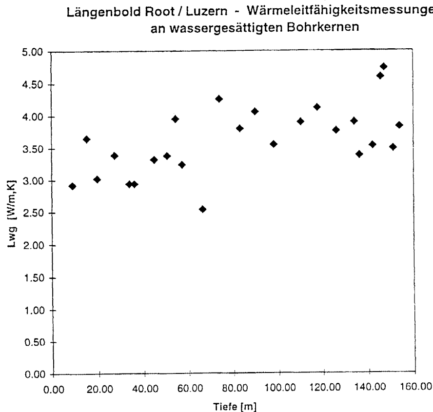
Fig. 8 Laboratory measurements of the ground samples taken in a borehole drilled between the north and south borehole heat exchangers (Schärli and Rybach, 1999).
