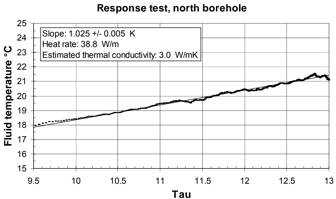
Fig. 6 Estimation of the thermal conductivity for the north borehole.
