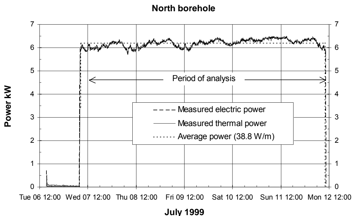
Fig. 4 Evolution of the injected thermal power in the north borehole.
