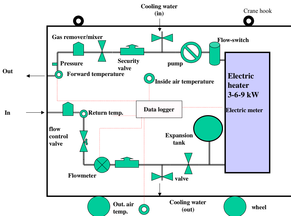
Fig. 2 Schematic view of the response test device.
