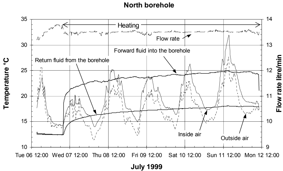
Fig. 5 Evolution of the measured temperatures and flow rate in the north borehole.
