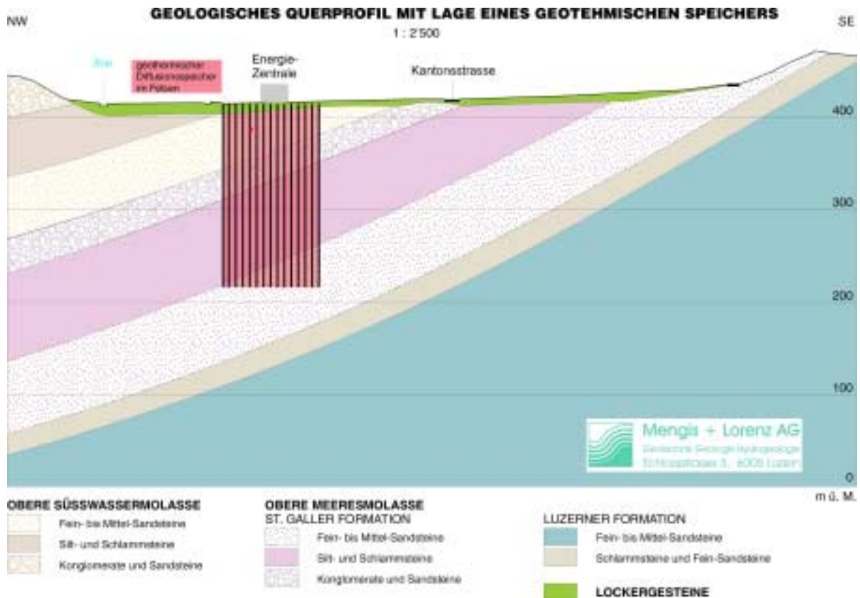
Fig. 1 Geological model of the ground at the site of the boreholes of the future ground heat storage (Keller, 2000).
