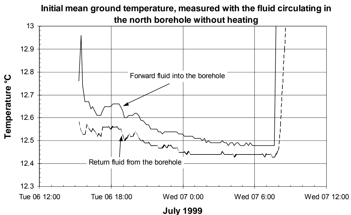
Fig. 3 Evolution of the fluid temperature in the north borehole before heating.
