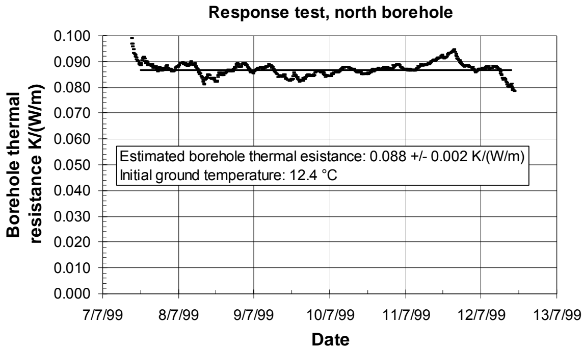
Fig. 7 Estimation of the effective borehole thermal resistance of the north borehole.
