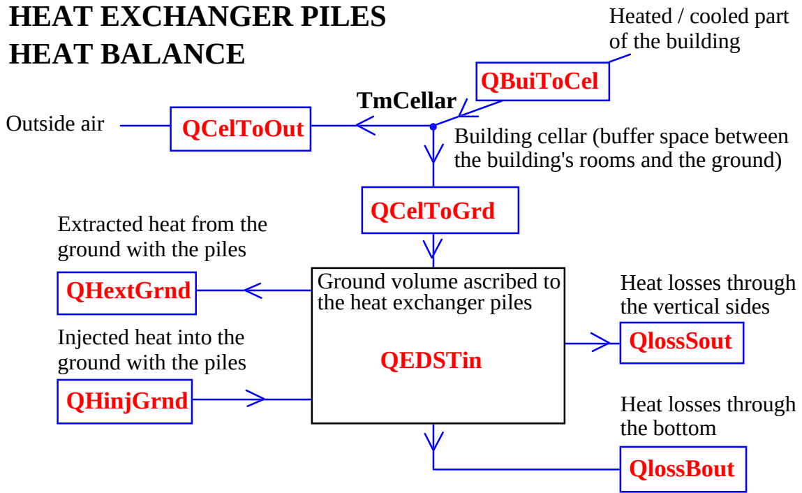
Fig. 5.2 Energy fluxes diagram of the heat exchanger piles.
