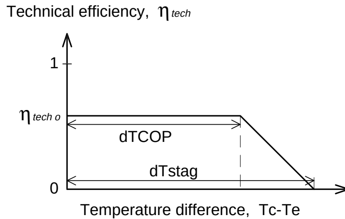
Fig. 3.1 Technical efficiency shape of the heat pump / cooling machine.
