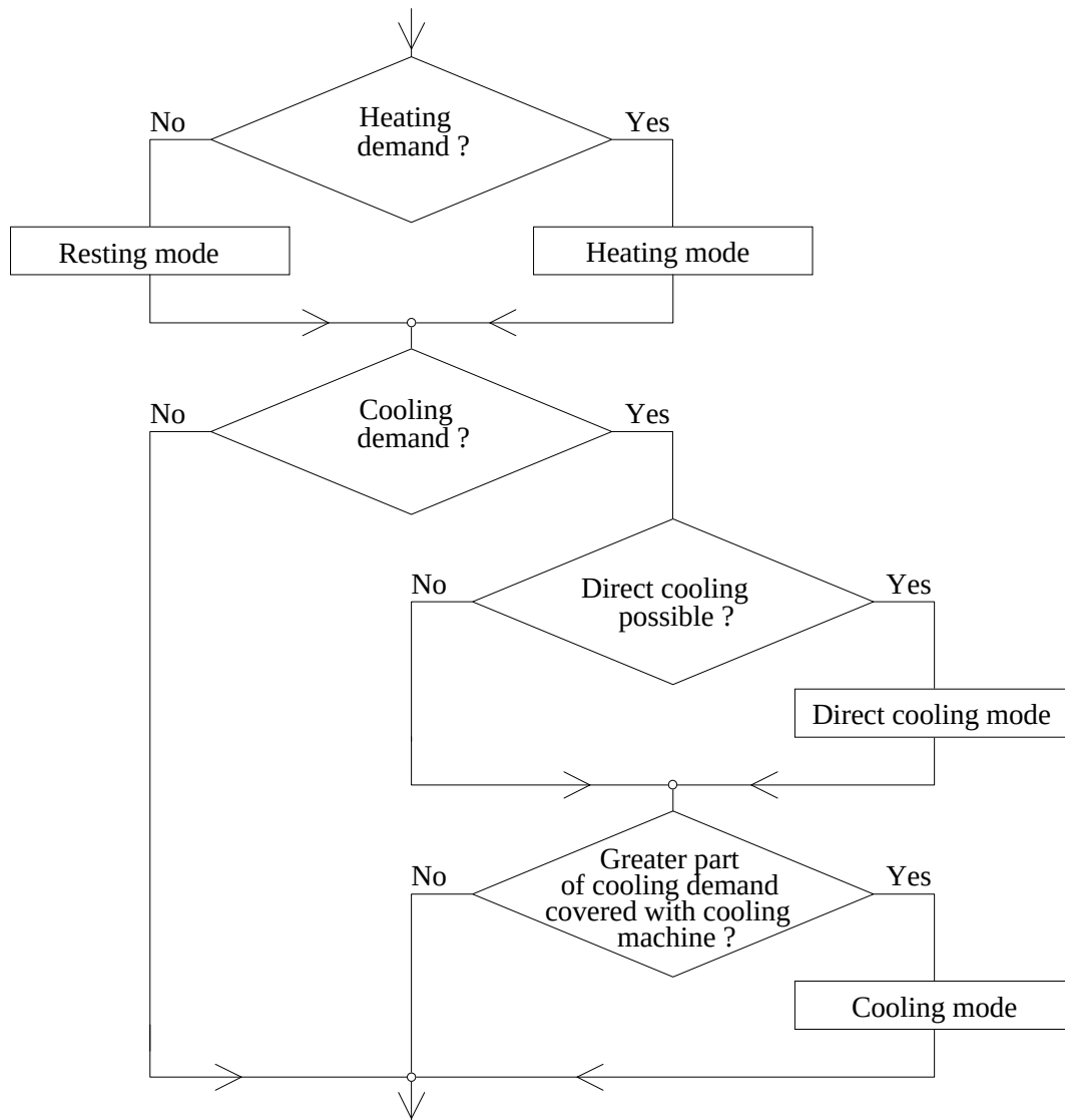
Fig. 2.3 Schematic presentation of the procedure followed to determine the operational mode.
