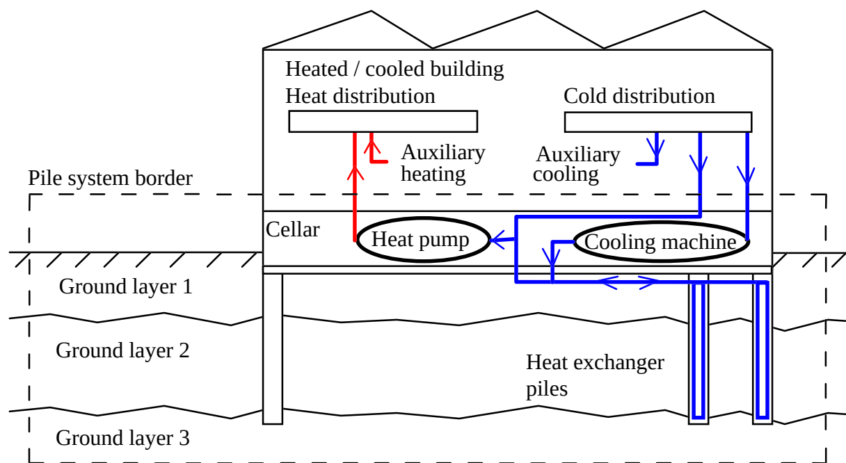
Fig. 2.1 Schematic view of a heat exchanger pile system. The part of the system which is simulated by the PILESIM programme is delimited by the pile system border shown with the dashed line.
