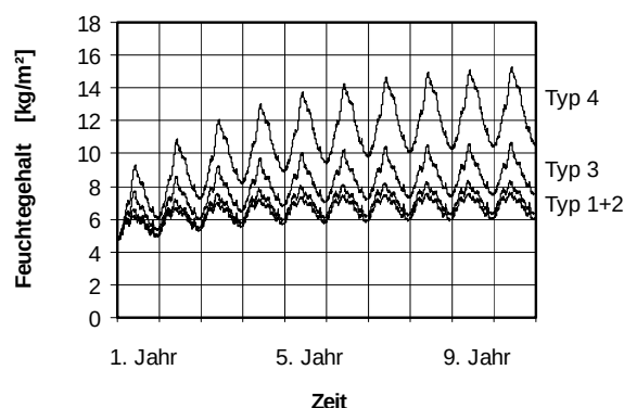
Figure 2: Moisture content inside a wall by using different lining boards (types of treatment), without rain load
