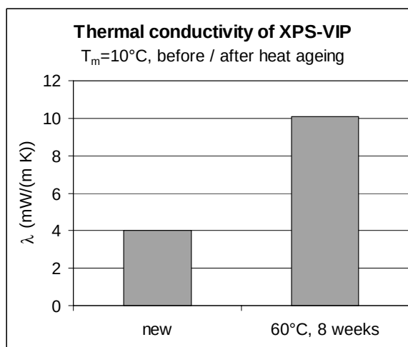
Fig. 3: Thermal conductivity of a VIP before and after application of a heat ageing procedure adapted from the draft EN product standard for PUR foams.
