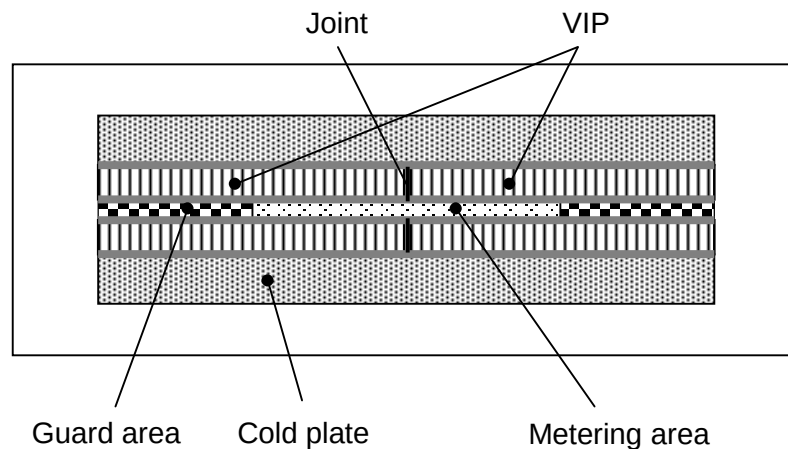
Fig. 5: Measurement of the edge conductance in a symmetric guarded hot plate facility. Two 375 x 750 mm 2 specimens were placed on each side. The 1-dimensional thermal conductivity was measured with two 750 x 750 mm 2 specimens.
