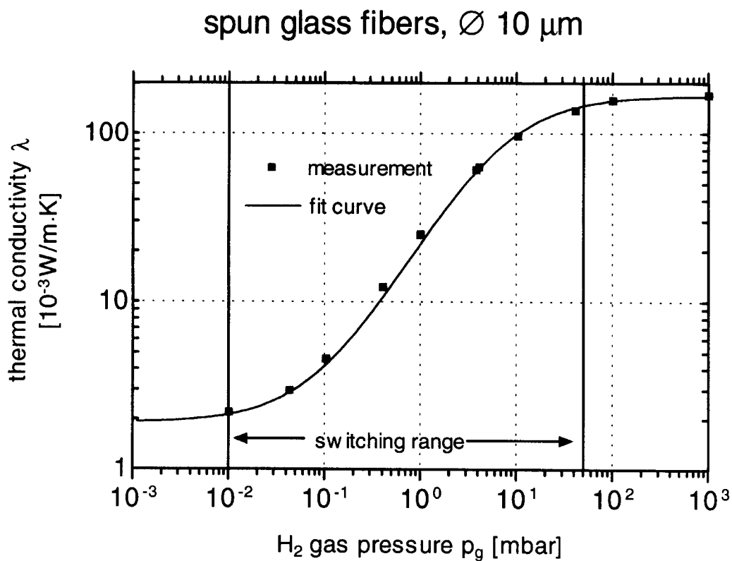
6. Thermal conductivity of a glass fiber board as a function of H 2 pressure
