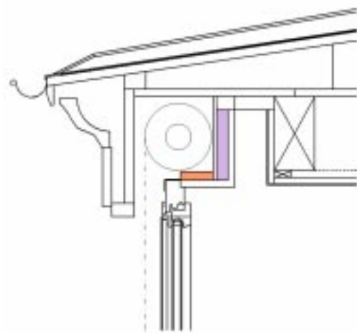
Fig. 8: Installation of vacuum insulation panels in roller blind boxes
