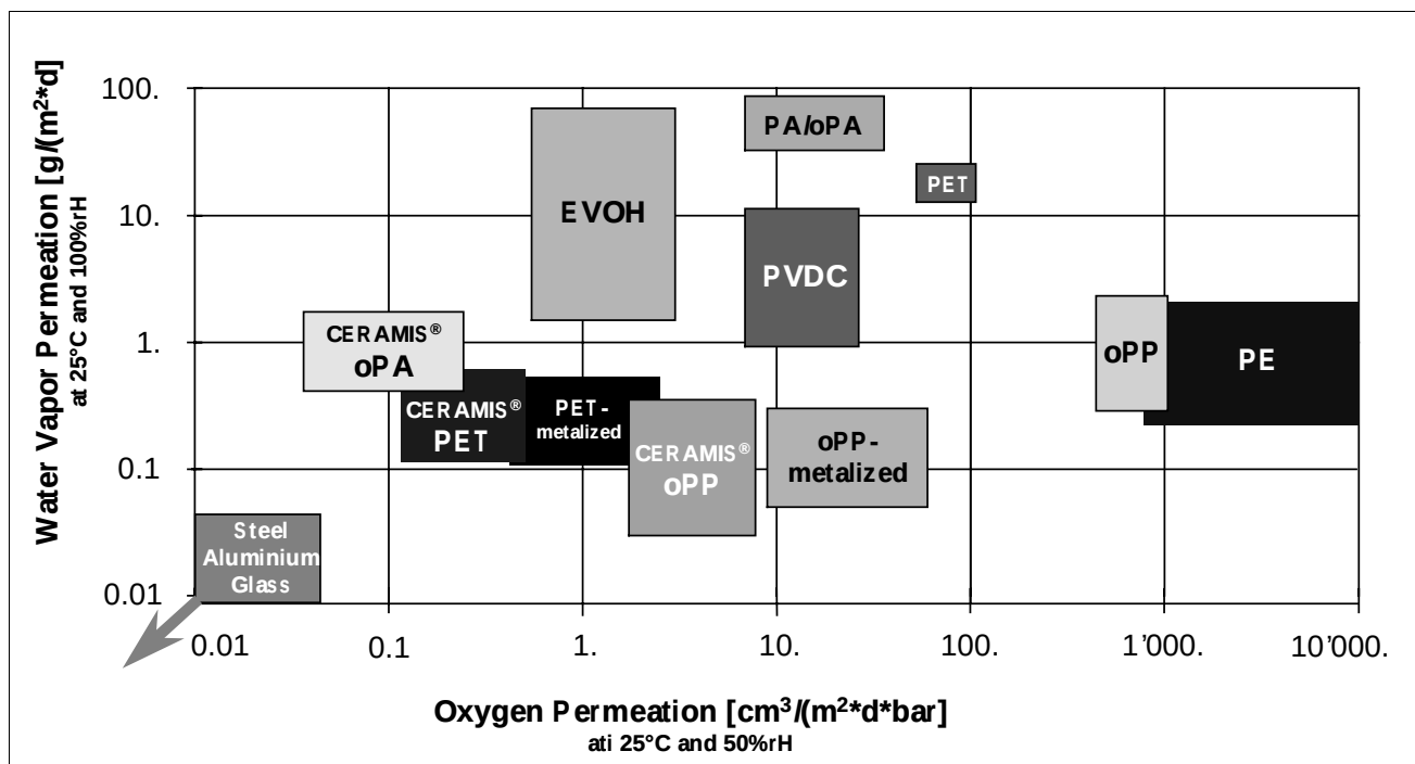
Fig. 2: Barrier - Permeation rates in comparison
