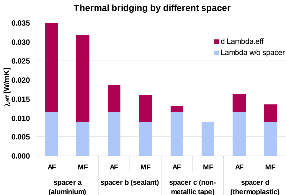
Figure 16: Thermal bridge edge effect of different spacers in façade panel constructions. The used VIP have metallized- (MF) or aluminium foil (AF) envelopes. The center-of-panel conductivity is 8 \cdot 10^{-3} \text{ W/(m}\cdot\text{K)} . The outside facing is 6 mm glass and the inside facing is 1.5 mm aluminium. "d Lambda.eff" is the increase for a panel of 100 \times 100 \times 2 \text{ cm}^3 compared to \lambda_{cop} .
