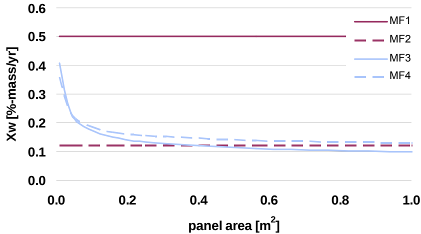
Figure 9: Edge effect on weight increase by water vapour permeation through four different metallized films. For the MF1 and MF2 samples, an edge effect could not be determined since the panels were too small (rectangular panel).
