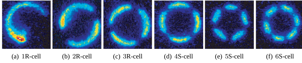
Fig. 1: Streamwise integrated chemiluminescence images taken from the downstream jet axis of a 22.5% \text{H}_2 (78.5% \text{CO}_2 ) jet flame burning in (a) 24.6% \text{O}_2 (75.4% \text{CO}_2 ) co-flow; (b) 26.0% \text{O}_2 co-flow; (c) 27.5% \text{O}_2 co-flow; (d) 31.0% \text{O}_2 co-flow, (e) 40.0% \text{O}_2 co-flow, and (f) 21.5% \text{H}_2 (79.5% \text{CO}_2 ) jet flame burning in 70.0% \text{O}_2 co-flow. "R" designates rotating and "S" stationary cell patterns. Fuel centerline and oxidizer velocities are U_F = 76 and U_O = 4 cm/s, respectively. [Figs. (a)-(e) taken with permission from Ref. [3]]
