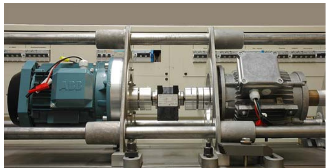
Fig. 17: Mechanical connection of ASM ⇔ BLDC motors
