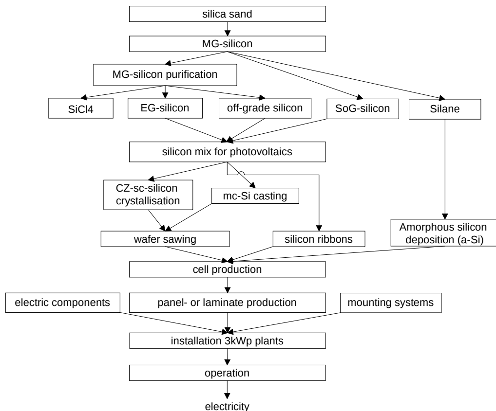
Fig. 1: Different sub systems investigated for the production chain of silicon cells based photovoltaic power plants installed in Switzerland. MG-silicon: metallurgical grade silicon, EG-silicon: e-lectronic grade silicon, SoG-silicon: solar-grade silicon, a-Si: amorphous silicon
