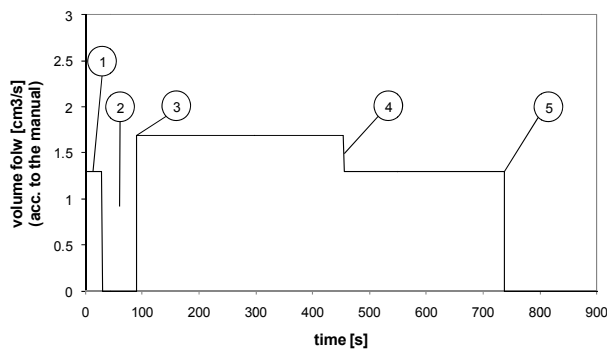
Fig.52: Regeneration procedure with standstill burner (system MK)
