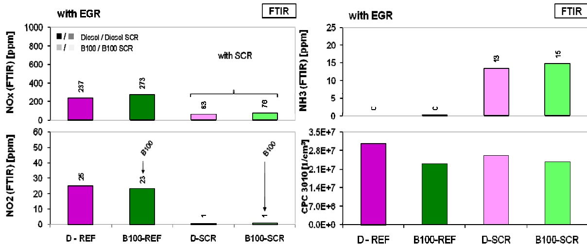
Fig. 27: Average emissions in ETC with Diesel & B100, with and w/o SCR Iveco F1C E4
