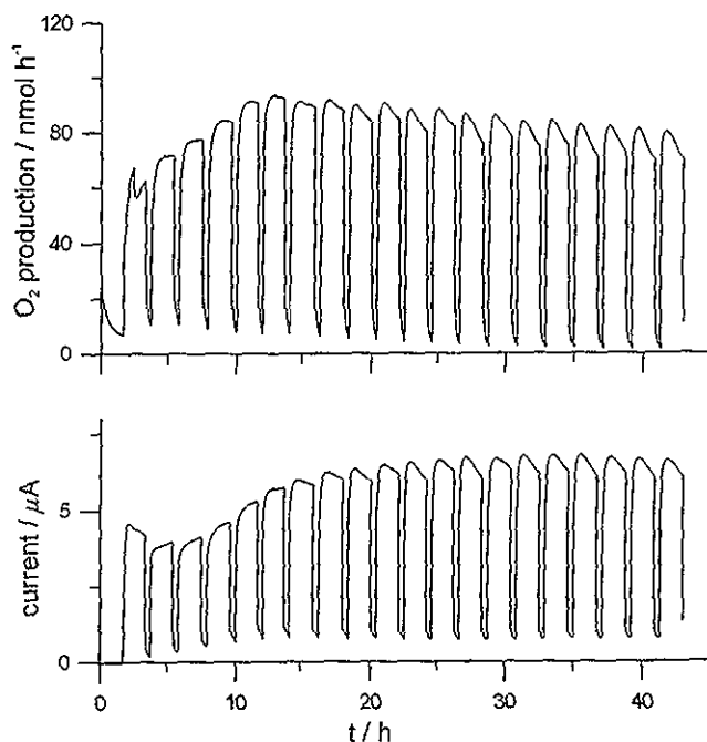
Fig. 12. Chronoamperometry of an electrochemically prepared AgCl-coated \text{SnO}_2:\text{F} electrode ( 1 \text{ cm}^2 ), modified with a thin gold layer ( 100 \text{ \AA} ), at 0.0 \text{ V} vs. \text{Hg}/\text{Hg}_2\text{SO}_4 , with illumination and dark periods, similar as in Figs. 5–8. The \text{O}_2 production rate ( \text{nmol h}^{-1} ) and the photocurrent ( \mu\text{A} ; anodic current is drawn upwards) are plotted vs. time. The light intensity at the AgCl-coated electrode was approximately 50 \text{ mW cm}^{-2} (illuminated through the cold light filter). During the period shown, the reoxidation was 64% and the number of turnovers of AgCl was 11.
