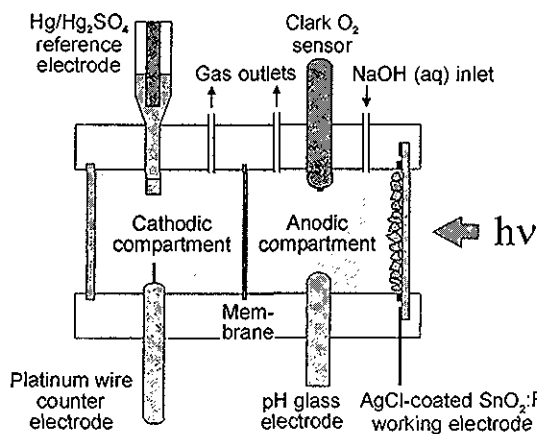
Fig. 4. Two-compartment photoelectrochemical cell for light-assisted water splitting.
