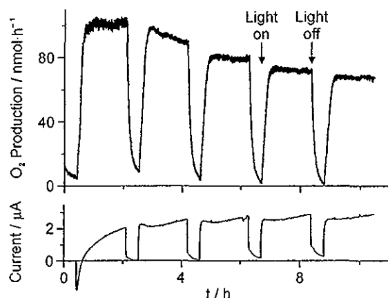
Fig. 5. Chronoamperometry of a precipitated, AgCl-coated \text{SnO}_2:\text{F} electrode at 0.0 V vs. \text{Hg}/\text{Hg}_2\text{SO}_4 , with illumination and dark periods. The \text{O}_2 production rate ( \text{nmol h}^{-1} ) and the photocurrent ( \mu\text{A} ; anodic current is drawn upwards) are plotted vs. time.
