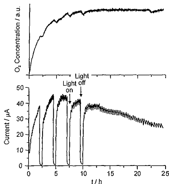
Fig. 10. Chronoamperometry of an electrochemically prepared, AgCl-coated SnO_2:F electrode (area, 5\text{ cm}^2 ) at 0.0 V vs. Hg/Hg_2SO_4 , with illumination and dark periods, in a two-compartment photoelectrochemical cell for light-assisted water splitting. Upper curve: concentration of dissolved O_2 in the anodic cell compartment (arbitrary units); O_2 saturation is reached after a few hours. Lower curve: polarization current ( \mu A ; anodic current is drawn upwards).
