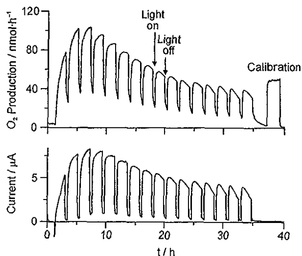
Fig. 8. Same chronoamperometric illumination experiment as in Figs. 5 and 6, but with an electrochemically prepared AgCl-coated SnO_2:F electrode.
