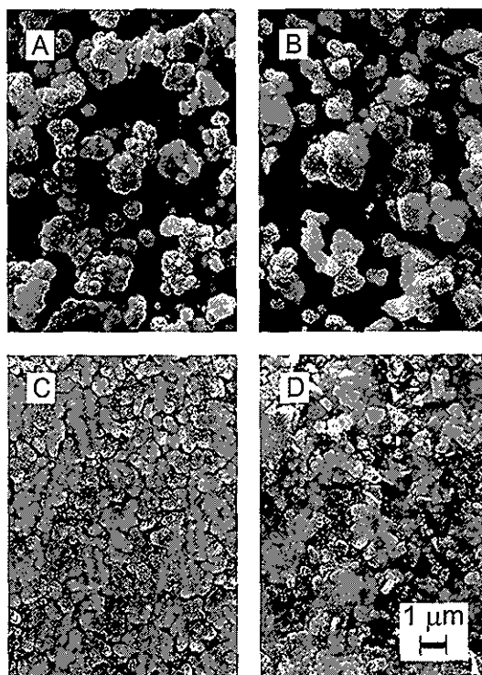
Fig. 9. Scanning electron micrographs of AgCl layers on SnO_2:F electrodes; (A) fresh, precipitated AgCl layer; (B) precipitated AgCl layer after a photoelectrochemical experiment; (C) fresh, electrochemically prepared AgCl layer; (D) electrochemically prepared AgCl layer after a photoelectrochemical experiment.
