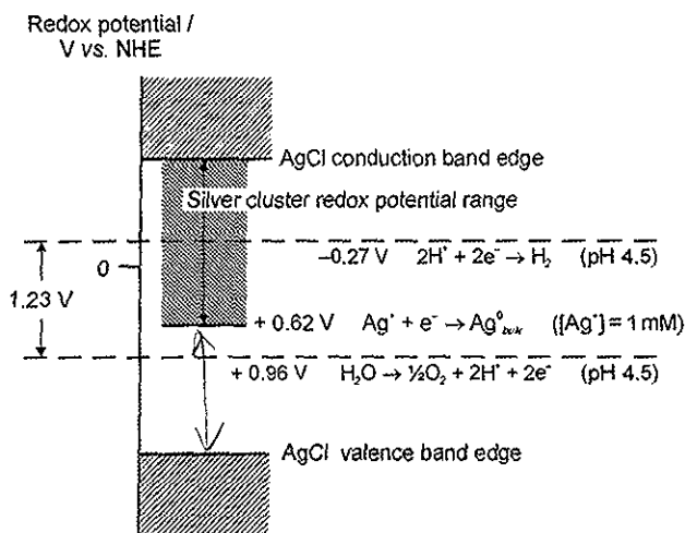
Fig. 11. Redox potentials for Ag^+/Ag_{bulk}^0 at [Ag^+] = 10^{-3}\text{ M} , for the oxidation ( O_2/H_2O ) and reduction ( H_2O/H_2 ) of water at pH 4.5, and position of the semiconductor band edges of AgCl. The band edges are approximately at +2.1 V (valence band) and at -1.2 V vs. NHE (conduction band [28]). The electrochemical potential range of small silver cluster is indicated (shaded region).
