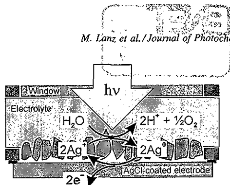
Fig. 1. Photocatalytic oxidation of water to O_2 on an AgCl-coated electrode and electrochemical reoxidation of the reduced silver.
