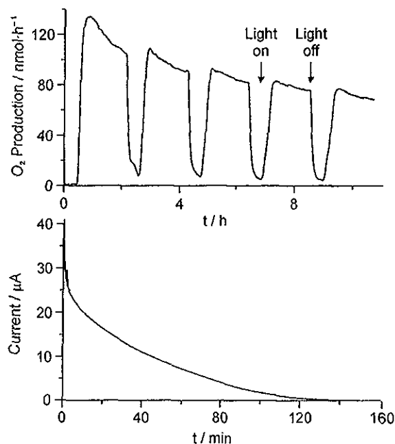
Fig. 7. Oxidation of water to O_2 on a precipitated, AgCl-coated SnO_2:F electrode under illumination, followed by electrochemical reoxidation of the reduced silver by chronoamperometry at 0.0 V vs. Hg/Hg_2SO_4 .
