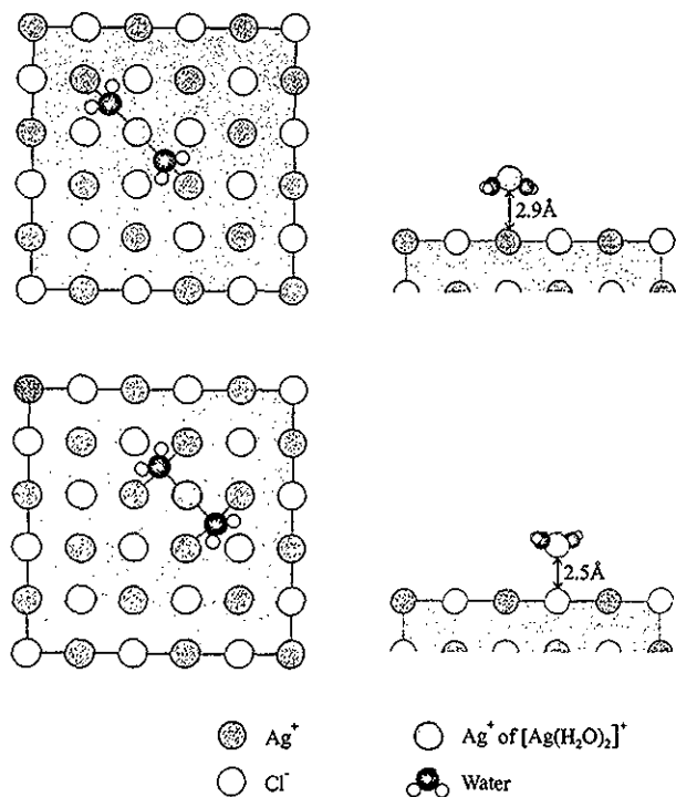
Figure 13. The two stable positions 1 (upper part) and 2 (lower part) of [\text{Ag}(\text{OH}_2)_2]^+ on the (\text{AgCl})_{108} surface. The \text{O}-\text{Ag}^+-\text{O} angle is 160^\circ and 200^\circ , respectively. On the left, bonding interactions are dashed.
