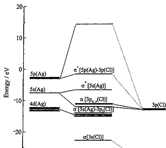
Figure 3. Correlation diagram of an AgCl molecule. On the left are the energy levels of the silver ion, and on the right are those of the chloride ion. The HOMO-LUMO electronic transition occurs at 3.9 eV and is of 5s(\text{Ag}) \leftarrow n[3p_{xy}(\text{Cl})] charge-transfer type.
