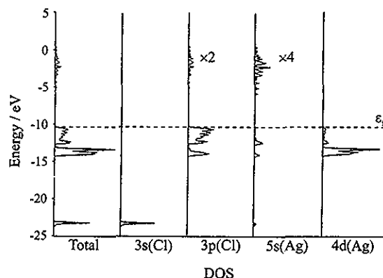
Figure 5. Density of states (DOS) and the contributions of 3s(Cl), 3p(Cl), 5s(Ag), and 4d(Ag) in the energy region from -25 to 5 eV. The dashed horizontal line indicates the Fermi level \epsilon_f at -10.3 eV.
