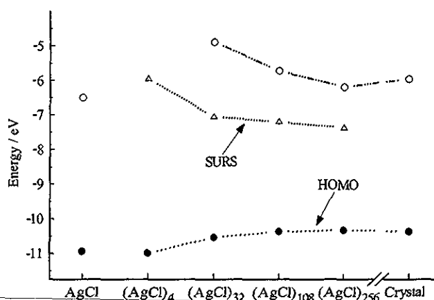
Figure 9. Frontier orbitals in dependence of the (\text{AgCl})_n cluster size.
