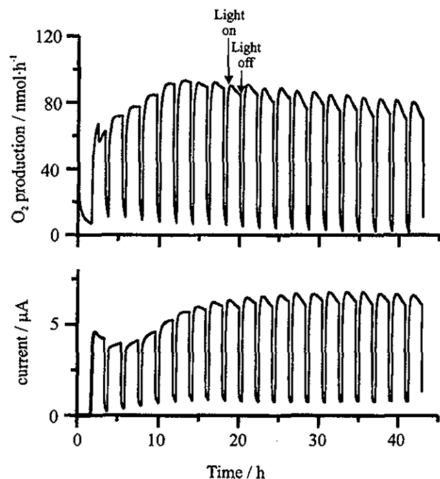
Figure 1. Photoelectrochemical experiment illustrating the photocatalytic oxidation of water on an electrochemically prepared AgCl-coated \text{SnO}_2/\text{F} electrode ( 1 \text{ cm}^2 ) modified with a thin gold layer ( 100 \text{ \AA} ) polarized at 0.0 \text{ V} vs \text{Hg}/\text{Hg}_2\text{SO}_4 . Oxygen production vs time (upper graph) and current vs time (lower graph). 6
