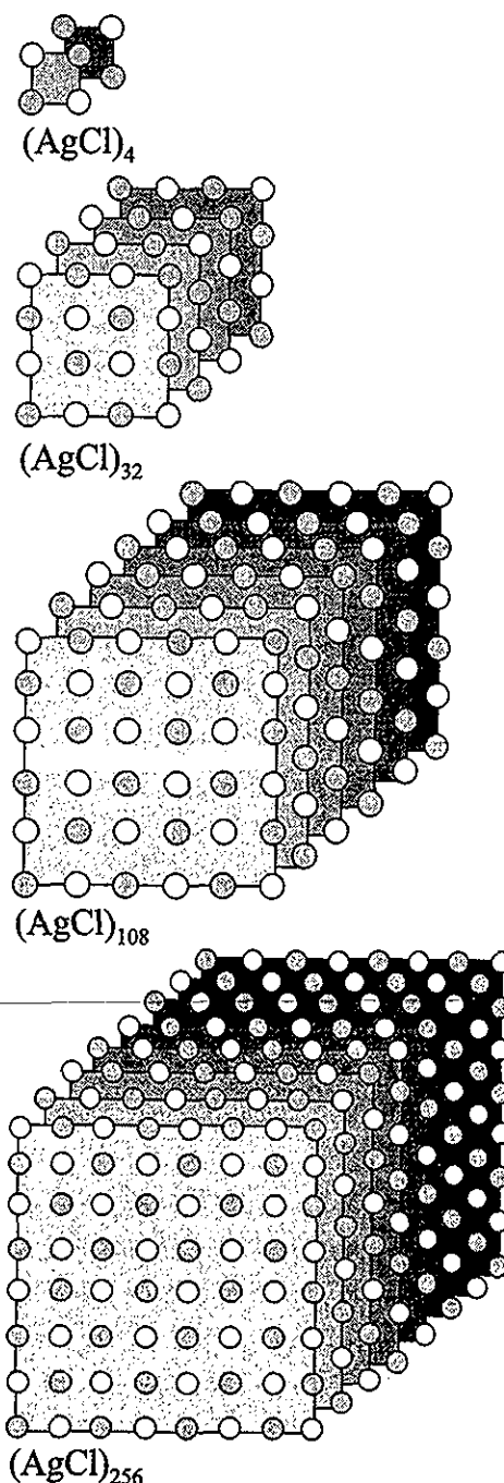
SCHEME 1: (\text{AgCl})_n Clusters; Grey Circles Represent the Silver Ions, White Circles the Chloride Ions.
