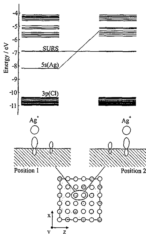
Figure 14. The 5s(\text{Ag}) levels deriving from [\text{Ag}(\text{OH}_2)_2]^+ on (\text{AgCl})_{108} positions 1 (left) and 2 (right), qualitatively explained below.
