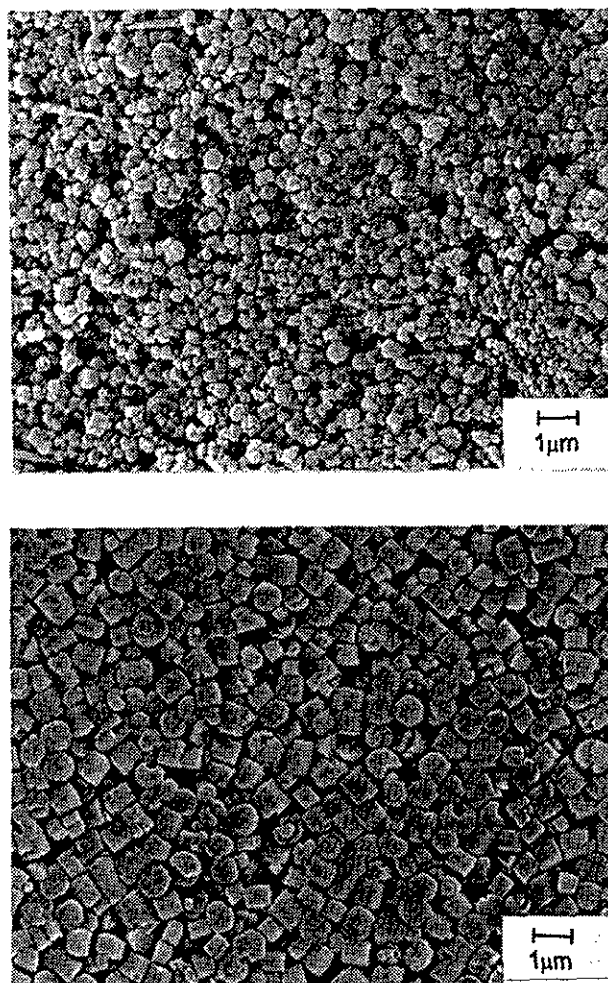
Figure 1. Scanning electron microscopy pictures of the commercial (on top) and the self-synthesized (on bottom) zeolite L samples.
