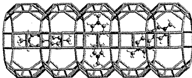
SCHEME 1: Different Spatial Configurations to Be Considered for MV^{2+} in the Channels of Zeolite L
