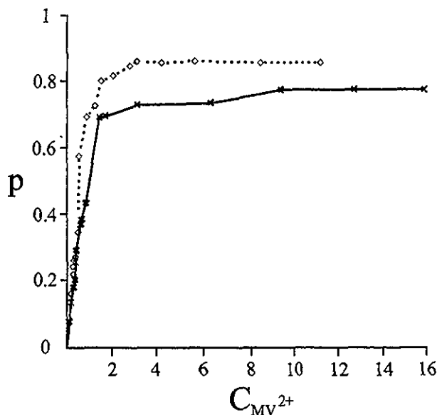
Figure 2. The occupation probability p of the MV 2+ -L zeolite as a function of C_{\text{MV}^{2+}} , which is the number of moles of MV 2+ per mole of zeolite L unit cells present in the aqueous suspension. Experiments with self-synthesized zeolite are indicated by diamonds ( \diamond ) and experiments with commercial zeolite by crosses ( \times ).
