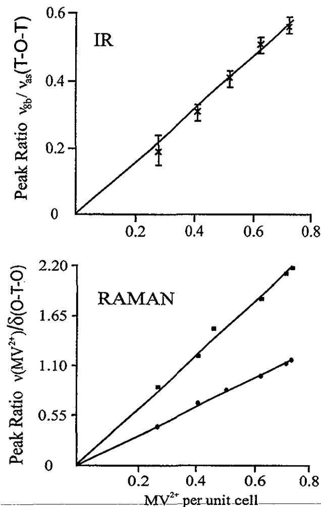
Figure 9. Top graph (concerning IR spectra) shows a correlation between the loading p ( MV^{2+} per unit cell) of MV^{2+} -L and the ratio of the area of the \nu_{86}(MV^{2+}) = 1507\text{ cm}^{-1} band and the \nu_{as}(T-O-T) = 1040\text{ cm}^{-1} band. Bottom graph shows the same for the Raman bands \nu_{86}(MV^{2+}) = 1651\text{ cm}^{-1} shown by squares (■) and \delta_{92}(MV^{2+}) = 1184\text{ cm}^{-1} shown by circles (●) in both cases with respect to the \delta(O-T-O) = 500\text{ cm}^{-1} zeolite band.
