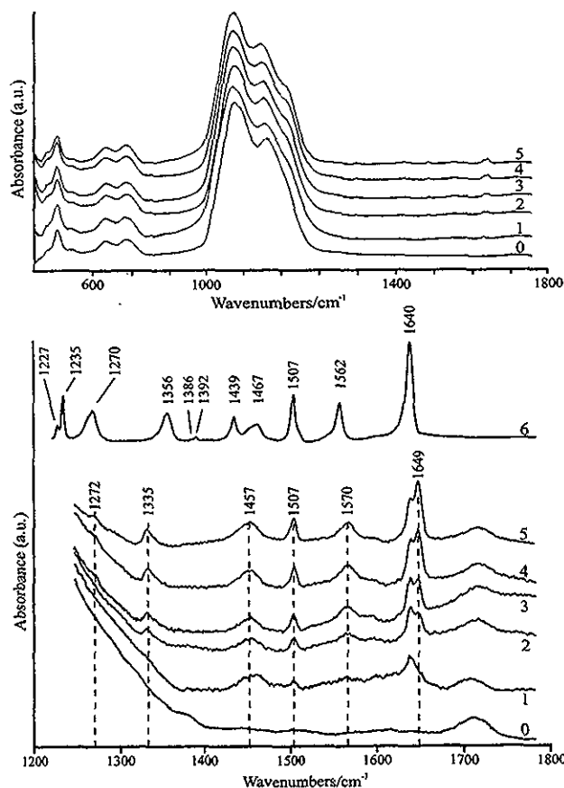
Figure 4. Above: IR absorption spectra of MV 2+ -L zeolite at different loadings. The numbers 0, 1, 2, ..., 5 refer to p = 0, 0.27, 0.41, 0.52, 0.62 , and 0.72 , respectively. Below: Enlargement of the IR absorption spectra 0 to 5 shown above and 6 of a MVCl 2 -KBr pellet between 1220 and 1800 cm -1 .
