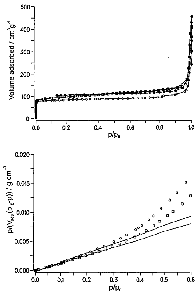
Figure 10. (a) Nitrogen isotherms of commercial zeolite (O) and of self-synthesized zeolite (□). The filled symbols represent the desorption data. (b) BET-plot of commercial (O) and of self-synthesized zeolite (□) in the p/p_0 range of 0.05–0.25.
