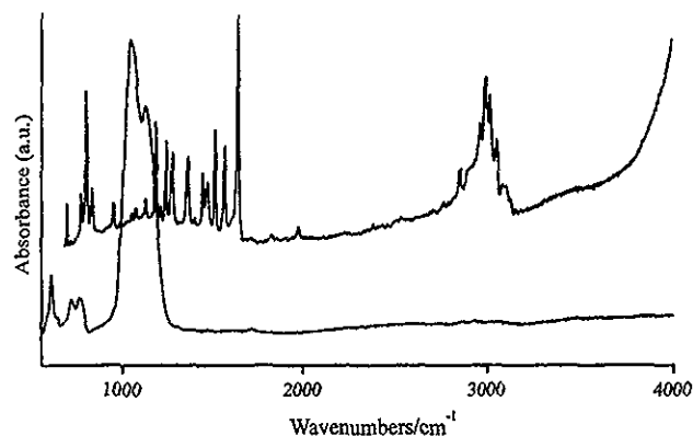
Figure 3. Overview of a thin layer unloaded zeolite L IR spectrum in high vacuum (below) and of MVCl 2 in a KBr pellet (above).
