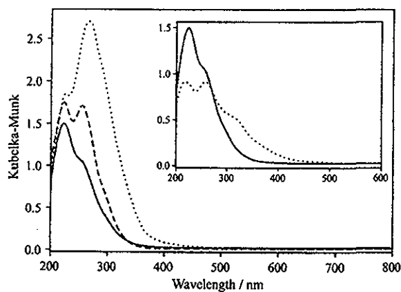
Figure 2. UV/vis absorption spectra of \text{Ag}_2\text{S}\text{--NaA-}0.05 (solid line), \text{Ag}_2\text{S}\text{--NaA-}0.10 (dashed line), and \text{Ag}_2\text{S}\text{--NaA-}0.50 (dotted line) before exposure to ambient conditions. The inset shows the spectrum of freshly synthesized \text{Ag}_2\text{S}\text{--NaA-}0.05 under inert atmosphere (solid line) and after 3 h under ambient conditions (dotted line).
