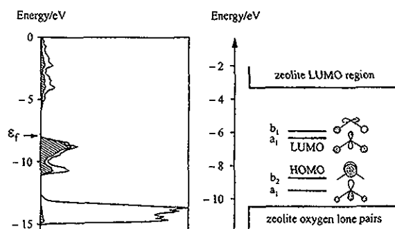
Figure 1. Left: Density of states (DOS) plot of \alpha\text{-Ag}_2\text{S} . The hatched region indicates the contribution of sulfur 3p-states (BICON-CEDiT 5 calculation). The Fermi level \epsilon_f is marked by an arrow. Right: HOMO–LUMO region of a hypothetical \text{Ag}_2\text{S} molecule in comparison to the HOMO–LUMO region of zeolite A (ICON-EDiT 6 calculation).
