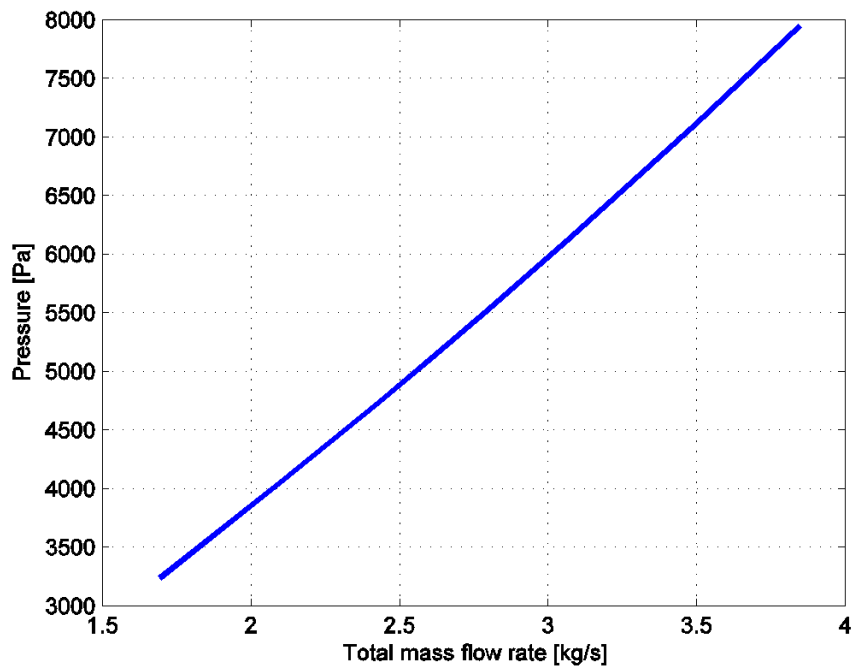
FIGURE 15: PRESSURE DROP AS A FUNCTION OF THE TOTAL MASS FLOW RATE.
