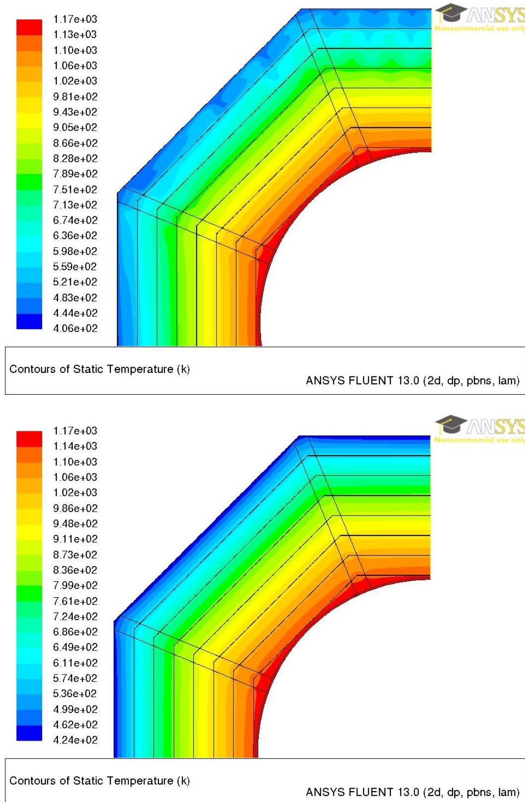
FIGURE 11: STATIC TEMPERATURE DISTRIBUTION FOR OPERATING PRESSURE OF 101'325 Pa (TOP) AND 100 Pa (BOTTOM) – NUMBER OF SHIELDS: 8.
