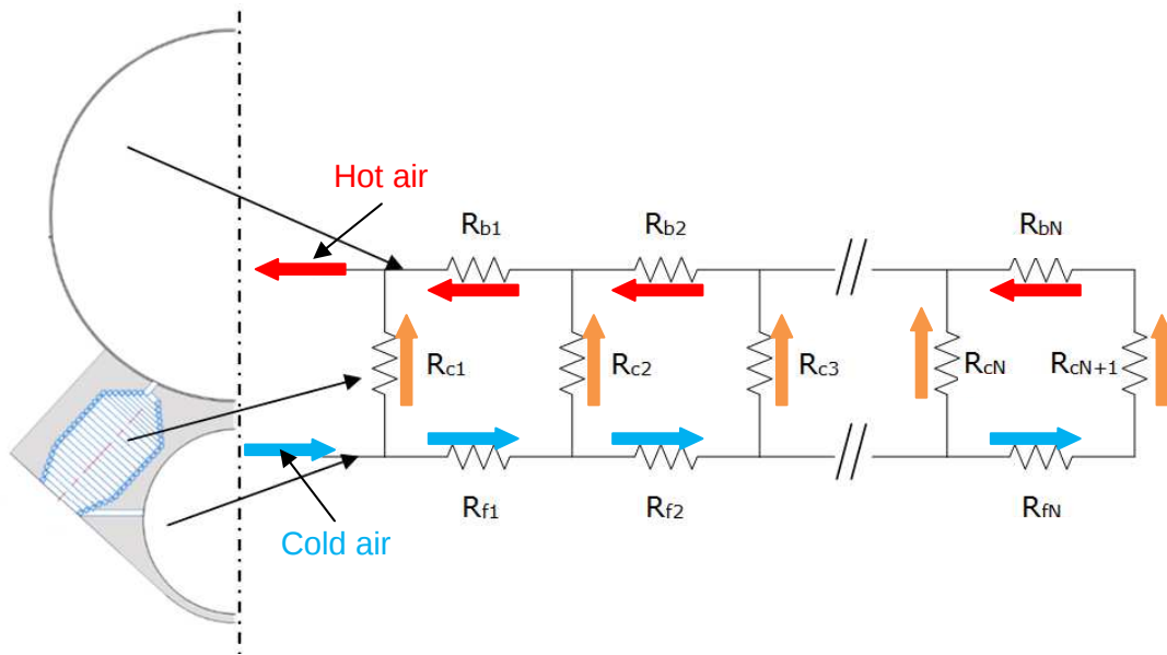
FIGURE 2: RECEIVER ELECTRICAL ANALOGY.
