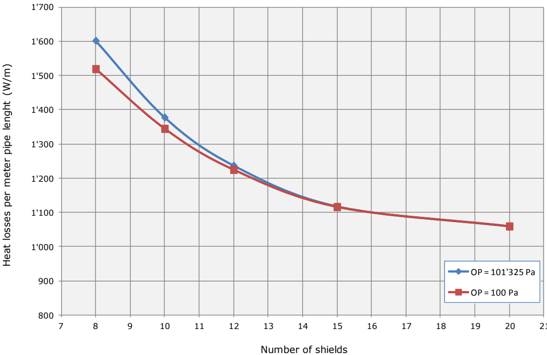
FIGURE 15: CASE 2 - HEAT LOSSES VERSUS NUMBER OF SHIELDS.
