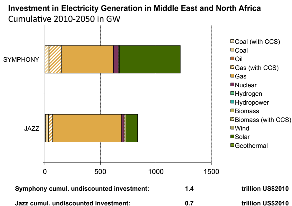
Figure 65 – Cumulative investment needs by 2050 in Middle East and North Africa in electricity generation infrastructure
