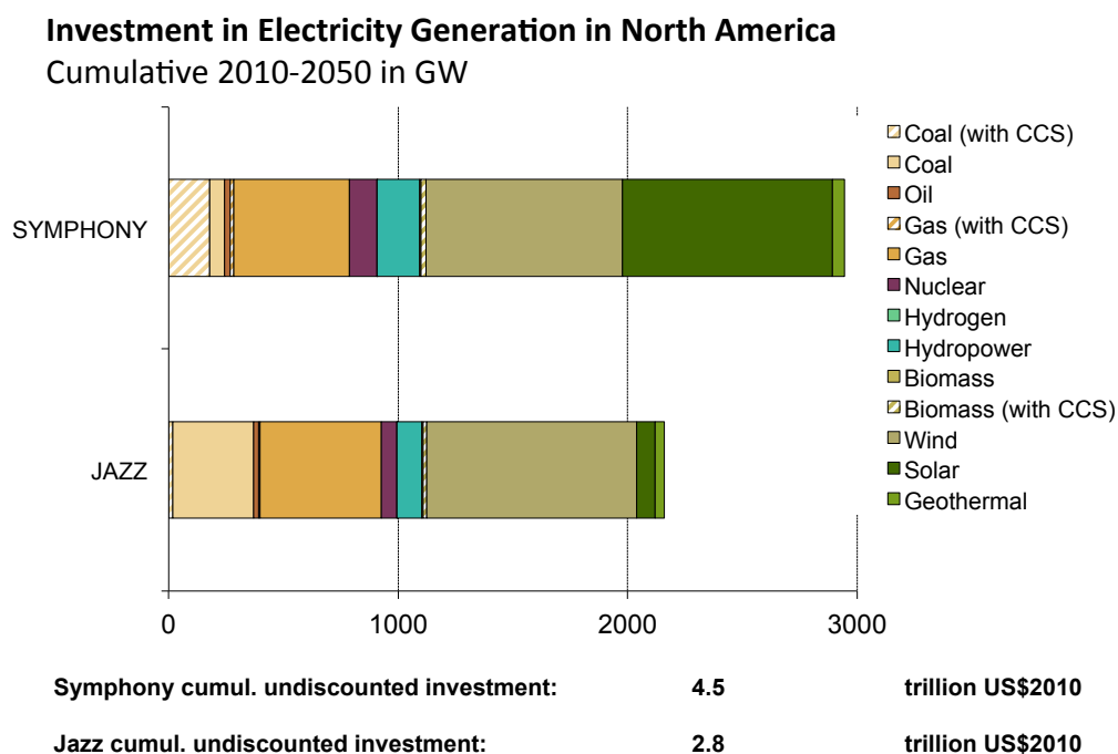
Figure 69 – Cumulative investment needs by 2050 in North America in electricity generation infrastructure
