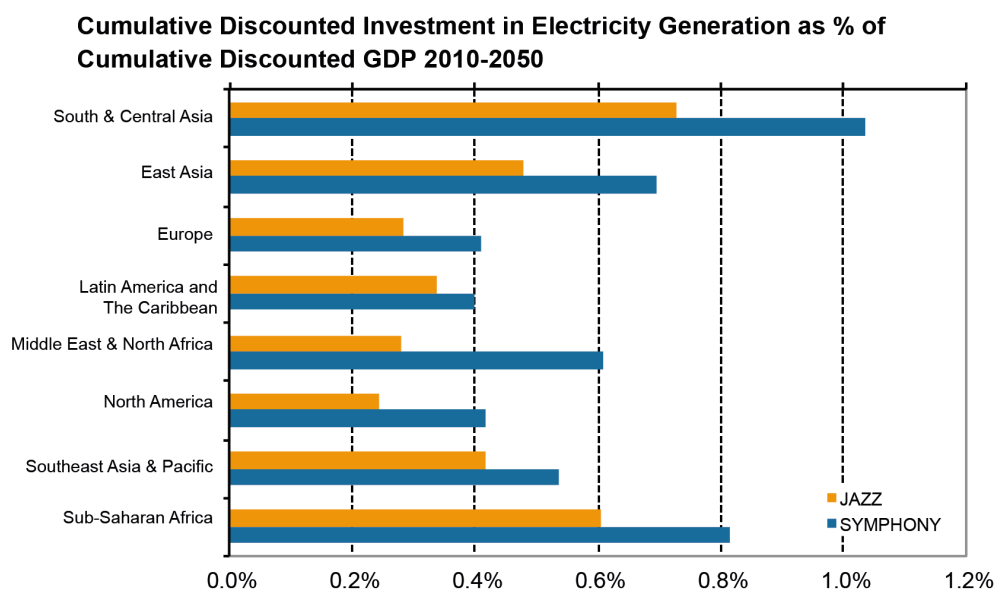
Figure 79 – Cumulative discounted investment in electricity generation as % of cumulative discounted GDP 2010 – 2050
