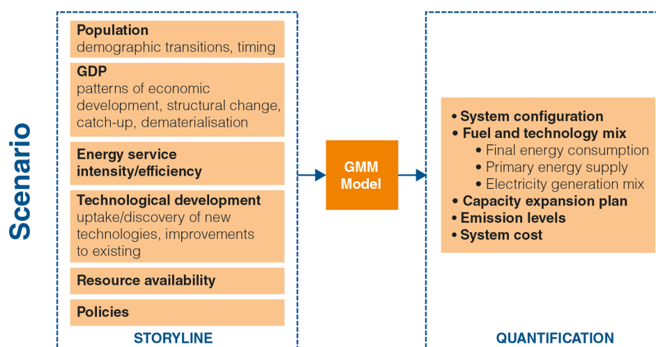
Figure 27 – WEC scenarios quantification: Use of a GMM MARKAL model
