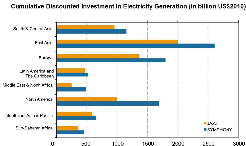
Figure 81 – Cumulative discounted investment in electricity generation in billion US$2010
