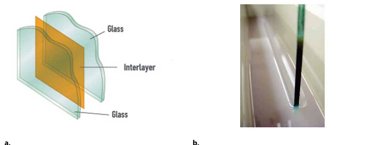
Figure 2. a. Thermo-acoustic interlayer for heat absorbing windows. Source: Nanohouse initiative Australia (UTS., 2002). b. Immersion bath for the deposition of pro.Glass Barrier 401 (special coating containing nano-ZnO) on a glass panel (Öko-Institut e.V., 2012).
