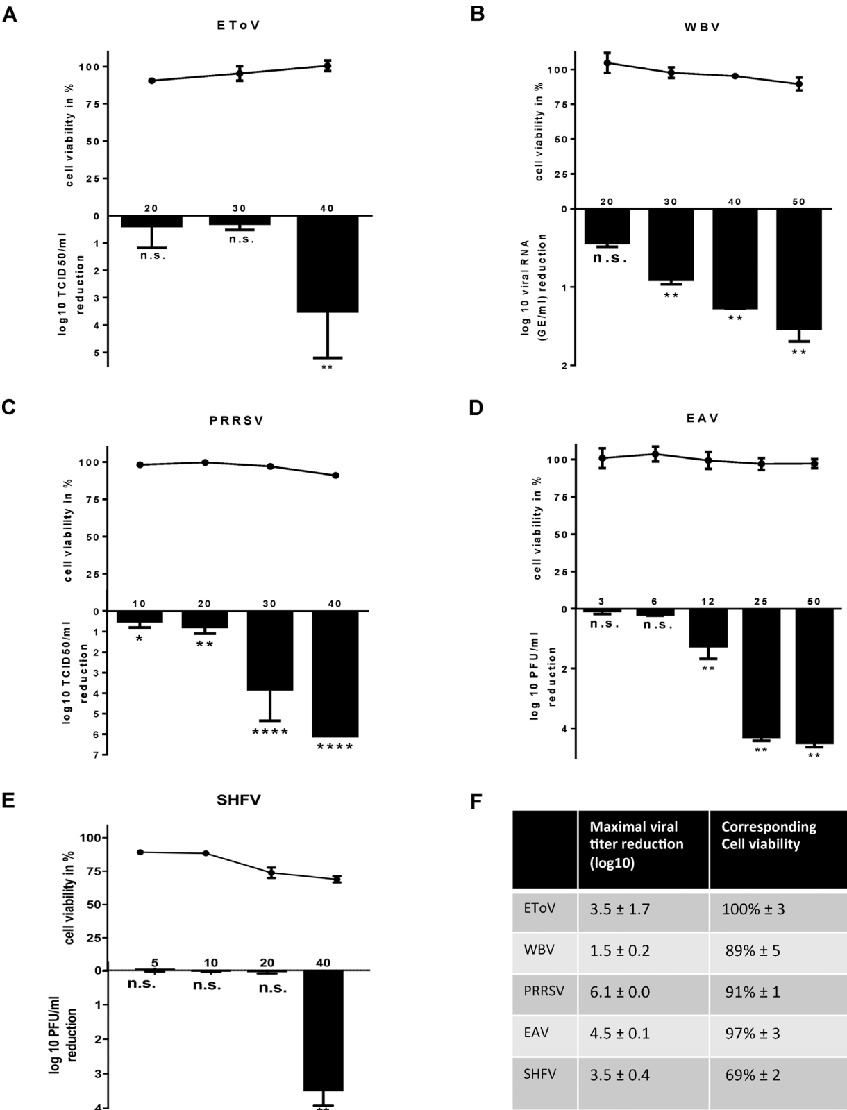
Fig. 1. K22 affects diverse nidoviruses. The log reduction in virus yield (bars) and the percent of cell viability (solid line above bars) are shown for K22-treated torovirus- (A) bafinivirus- (B) and arterivirus-infected (C, D and E) cell lines of equine (E-Derm for EToV), fish (EPC for WBV), primate (MARC-145 for PRRSV and MA-104 cells for SHFV) or rodent (BHK-21 for EAV) origin. The cells were infected 4 h after treatment with different concentrations of K22 or solvent (DMSO) as a control. At 12 h (WBV, EAV), 24 h (SHFV) or 48 h (EtoV, PRRSV) post infection, viral titres or intracellular RNA levels were determined. Log reduction of virus production induced by K22 was calculated by comparing titres obtained in DMSO-treated cells (control) with titres obtained in cells treated with different concentrations of K22. Cytotoxicity was assessed with a Promega CytoTox-Glo™ Cytotoxicity Assay (for EToV), a CellTiter 96 AQ ueous nonradioactive cell proliferation assay (for PRRSV and EAV) or a MTT assay (for SHFV and WBV) and expressed in% of cell viability. Maximal viral titre reduction and the associated cell viability were determined for each virus and summarized in table format (F). Data are shown as mean ( ± SD) of 3–9 biological repeats. Statistical test: Mann-Whitney. n.s. = non-significant, *, p < 0.1, **, p < 0.01, ***, p < 0.001, ****, p < 0.0001.
