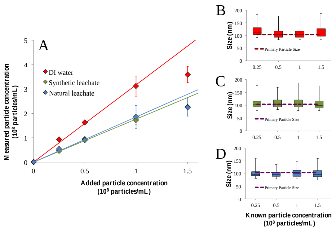
Figure 2: Particle number concentration calibration curves of Au nanoparticles suspended in DI H 2 O, synthetic and natural MSWI landfill leachates compared to the expected 1:1 known particle number to measured particle number ratio (A). A linear regression line of each of the calibration curves is presented through the linear portion of the data set (0 to 1 \times 10^8 particles/mL) with a predicted extension of the regression line until 1.5 \times 10^8 particles/mL to exemplify how these data are not in the linear range. Particle size distribution of particles measured at different dilutions in DI H 2 O (B), synthetic (C) and natural MSWI (D) leachates. For the box plots, 25% quantiles appear within the box plot with average particle size indicated by black line therein. Whiskers represent 95% of particle size distribution (outliers not shown). Purple dashed lines indicate Au ENM primary particle size (100 nm).
