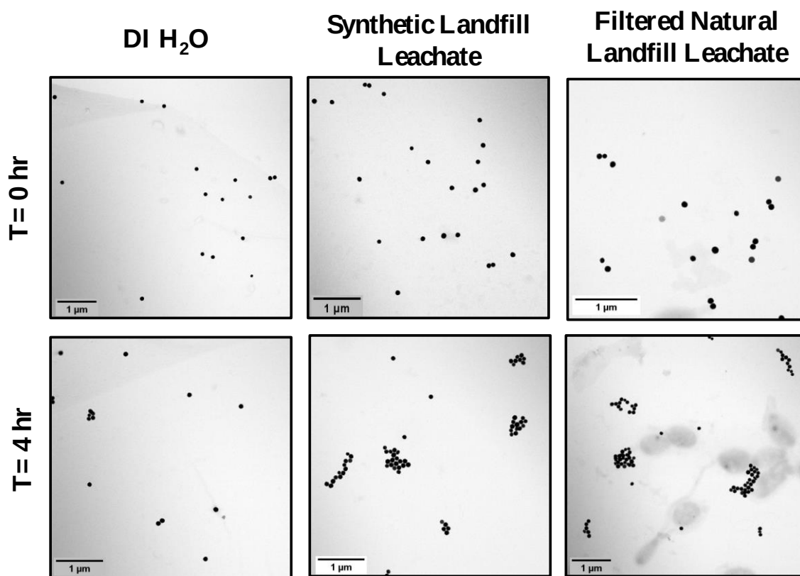
Figure 6: TEM images of Au ENM agglomeration state at T=0 hr and T=4 hr in DI H 2 O, synthetic landfill leachate and natural landfill leachate (filtered through 0.45 μm filter). Disperse, single particles are evident in all T= 0 samples and the DI H 2 O sample after 4 hrs, yet agglomeration is noted in both synthetic and natural landfill leachates after 4 hrs in solution. In the case of synthetic leachate, homoagglomeration (rather than heteroagglomeration) is evident; likely due to the high concentration of ENM dispersed in a solution with a relatively high salt concentration. In contrast, the ENM suspended in the natural leachate sample seemingly are affected by homoagglomeration as well as heteroagglomeration to the natural particles in the leachate.
