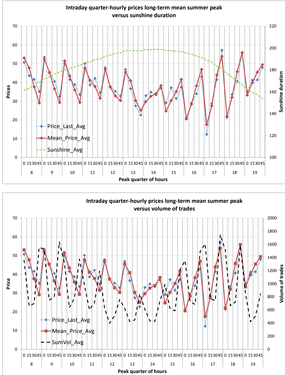
Figure 3: Seasonality pattern of the last prices and average prices bid for a certain quarter of an hour during the peak hours in summer. The right axes show the sunshine duration (upper graph) and the sum of volumes traded (lower graph).
