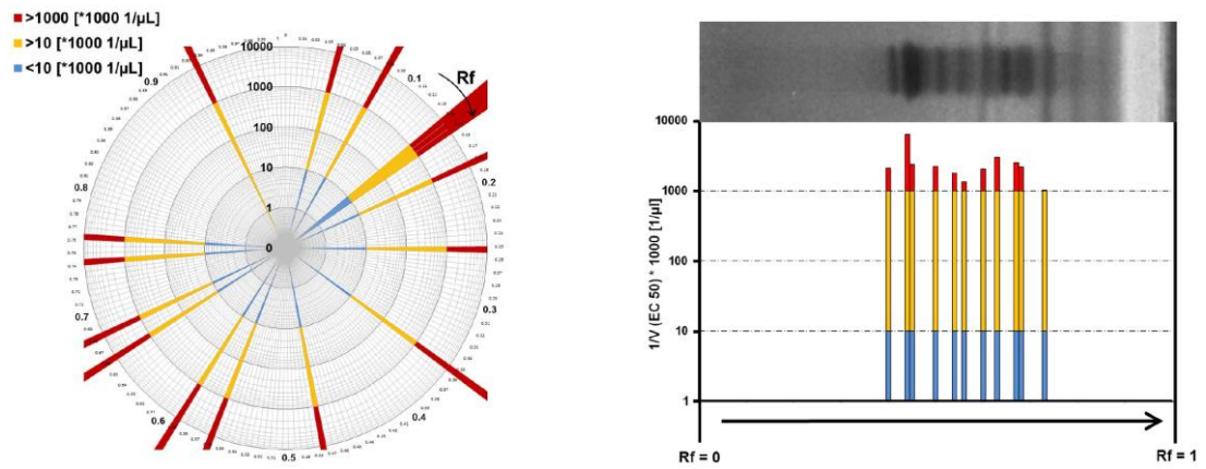
Figure 1. The left panel shows a rosette of polarity (based on retention factor, Rf) and toxicity (based on dilution factors) from a leachate from a landfill site (presentation of Stephan Weiß and Wolfgang Schulz, Landeswasserversorgung Baden-Württemberg, Dübendorf 15.12.2015). The right panel shows the principle of translating band intensity (b/w image) into toxicity. The different colours in the images indicate an increasing level of toxicity (blue < yellow < red).
