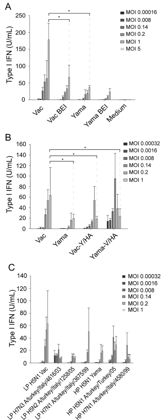
Figure 1 H5N1 AIV induce IFN in chicken splenocytes. Splenocytes were stimulated with various doses of AIV for 24 h. In (A), live and BEI-inactivated Vac and Yama viruses are shown. In (B), Vac and Yama are compared with the reassortants Vac-Y/HA and Yama-V/HA. In (C), various natural isolates of LPAIV and HPAIV are shown. IFN was quantified by bioassay. The averages of triplicate cultures with standard deviations are shown. The * indicates statistical differences calculated with the students t -test ( p < 0.05 ). The results are representative for at least three independent experiments.
