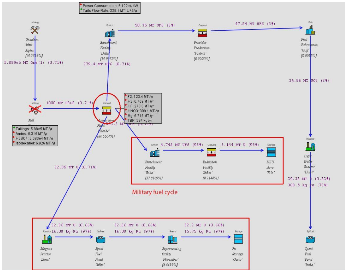
Above: a diagram showing the fuel cycles and material flows in Country A
