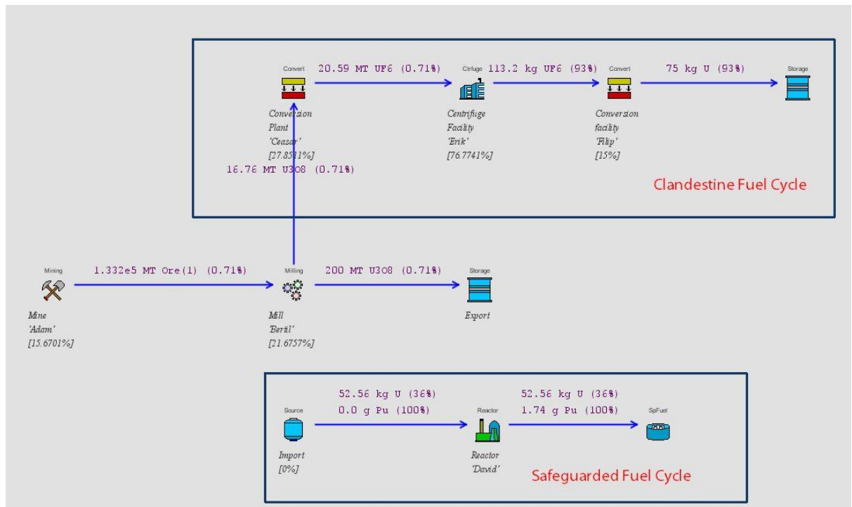
Above: a diagram showing the fuel cycles and material flows in Country C
